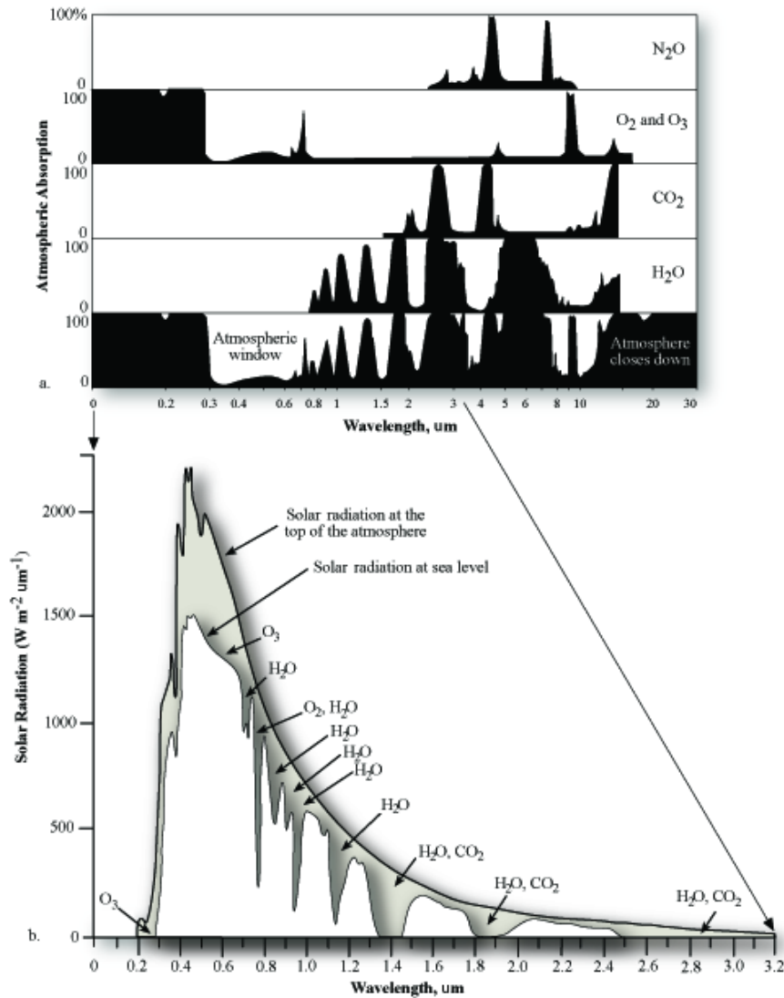
Figure 12. Absorption Bands
