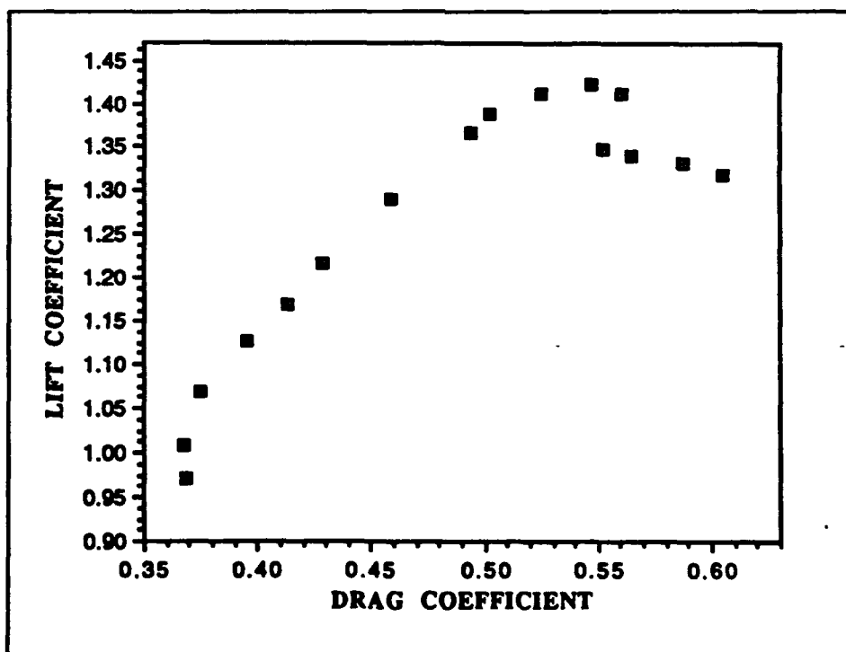
Figure 17. Lift vs. Drag Coefficient; AOA 22
