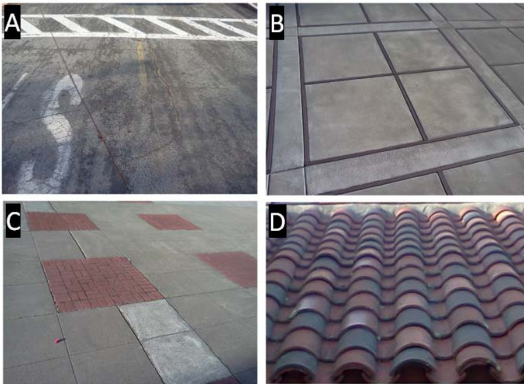
Figure 16. Various urban materials at NPS showing spectral variability within the FOV of a typical pistol grip foreoptic. Using the contact probe, each individual component is sampled. (A) Heavily worn asphalt with road paint (B) Two types of concrete with plastic border (C) Concrete with brick squares (D) Various clay roof tiles.
