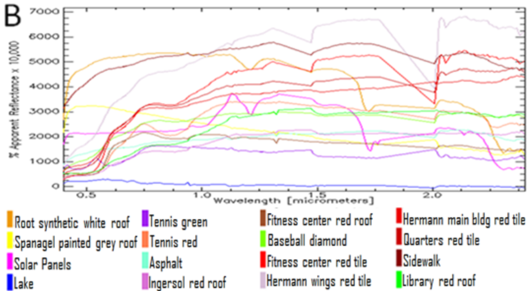
Figure 37. (A) Spectral Angle Mapper (SAM) classification of the AVIRIS data using image derived endmembers. Pixels were clumped and sieved to better visualize the data. (B) Endmember spectra are plotted below in Figure 37B with corresponding color scheme.
