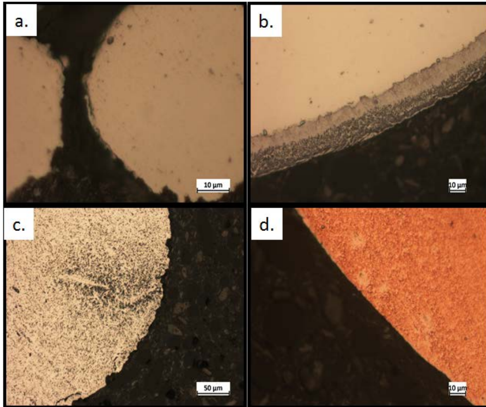
Figure 44. Optical images of (a.) Sample 12 (nickel), (b.) Sample 15 (stainless steel), (c) Sample 16 (tungsten), and (d) Sample 11 (copper).
