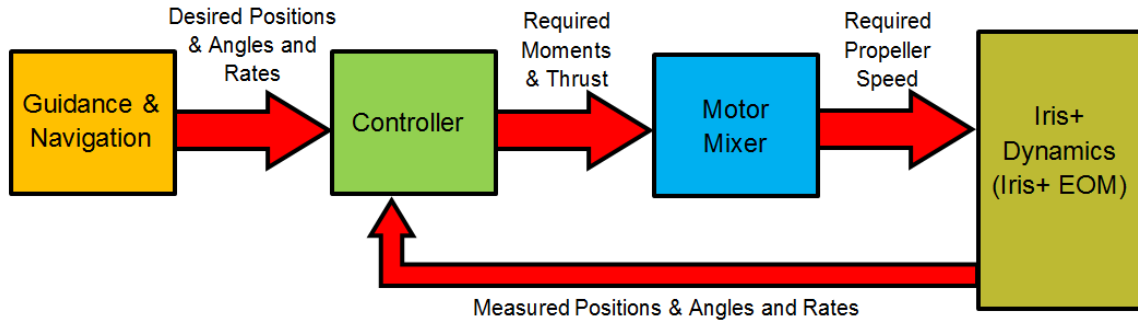
Figure 23 Block Diagram of Quadrotor Control Model.
