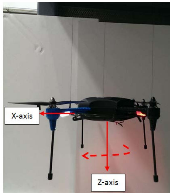
Figure 18 Measurement of Mass Moment of Inertia along z-axis.
