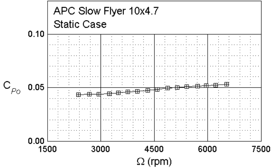
Figure 22 Power Coefficient vs Propeller Speed Plot (from [26]).
