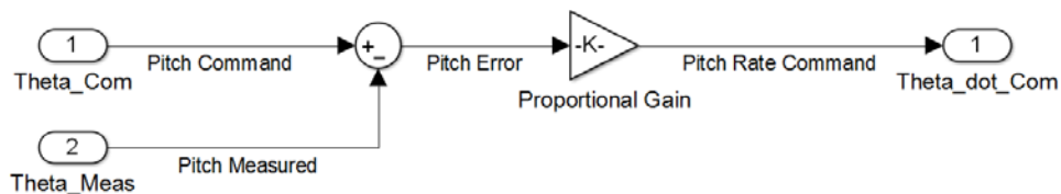
Figure 28 Pitch Channel Controller.
