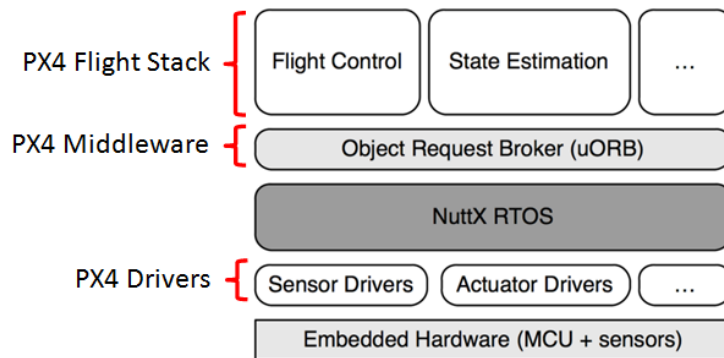
Figure 4 PX4 Flight Control Framework (after [2]).
