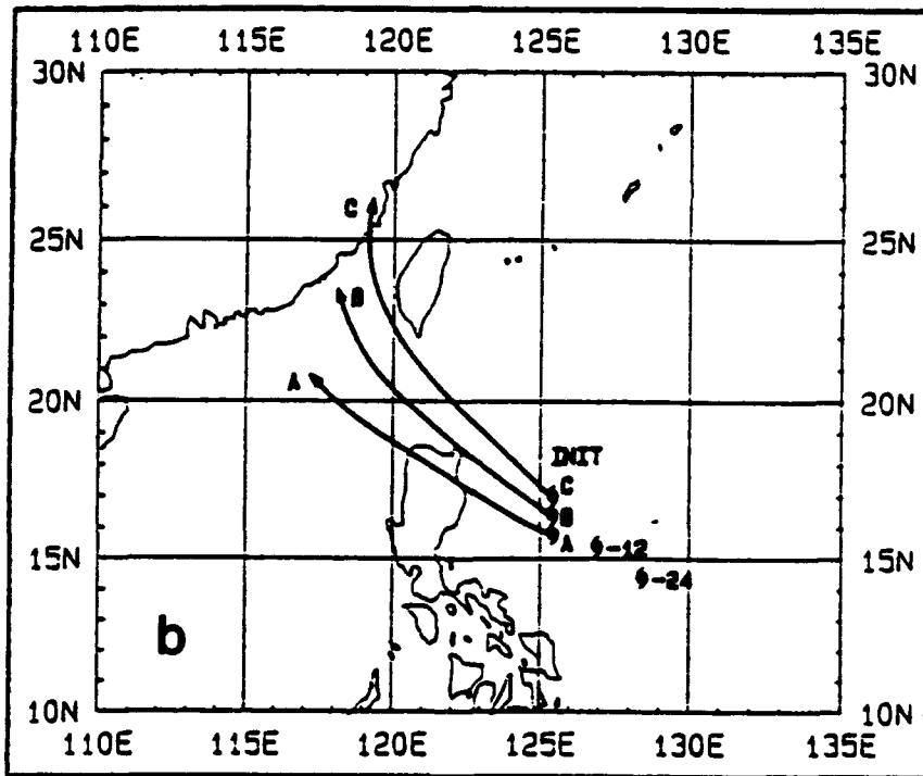
Fig. 5.5. Sensitivity of WPCLPR model to (a) initial longitude and (b) changes in past motion. (Englebretson, 1992)
