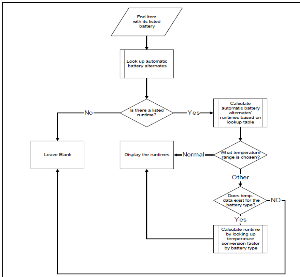
Figure 22. POWER 1.3e flowchart. Data from POWER 1.3e.
