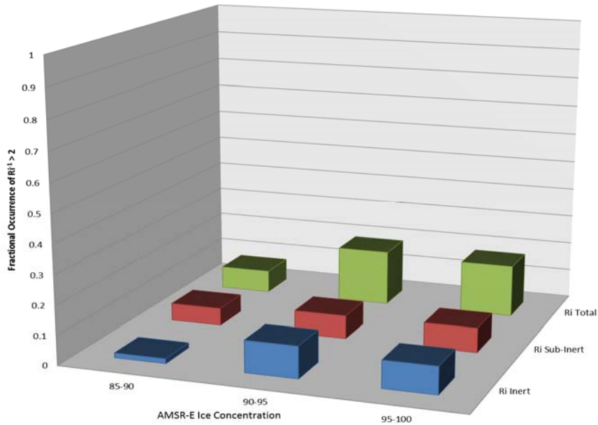
Figure 36. Top panel: Ri^{-1} > 2 compared to SSM/I sea ice concentrations for the Transpolar Drift. Bottom panel: Ri^{-1} > 2 compared to AMSR-E sea ice concentrations for the Transpolar Drift. ('Ri Total' calculated from subinertial and inertial velocities in green. 'Ri Sub-Inert' calculated from subinertial velocities in red. 'Ri Inert' calculated from inertial velocities in blue)
