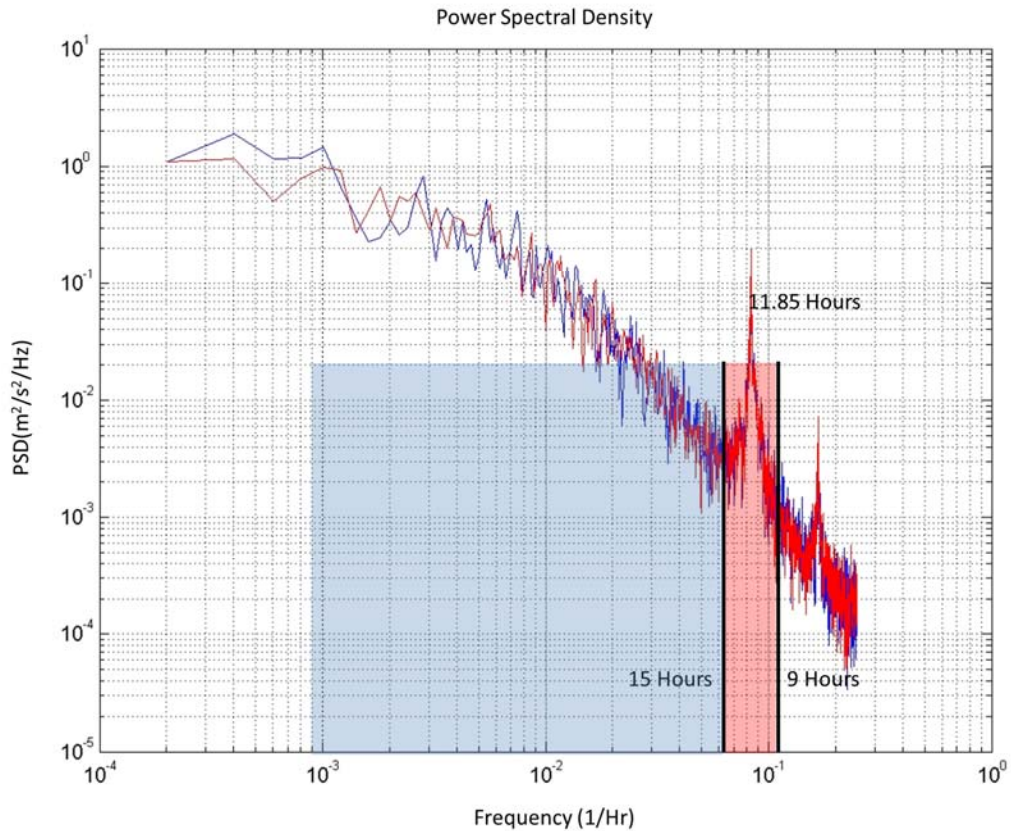
Figure 11. Example spectra of AOFB ADCP, used to determine cutoff times at 9 hours and 15 hour respectively. Inertial frequency band shaded in red. Subinertial frequency band shaded in blue. These two bands sum up to make ‘total velocity’.
