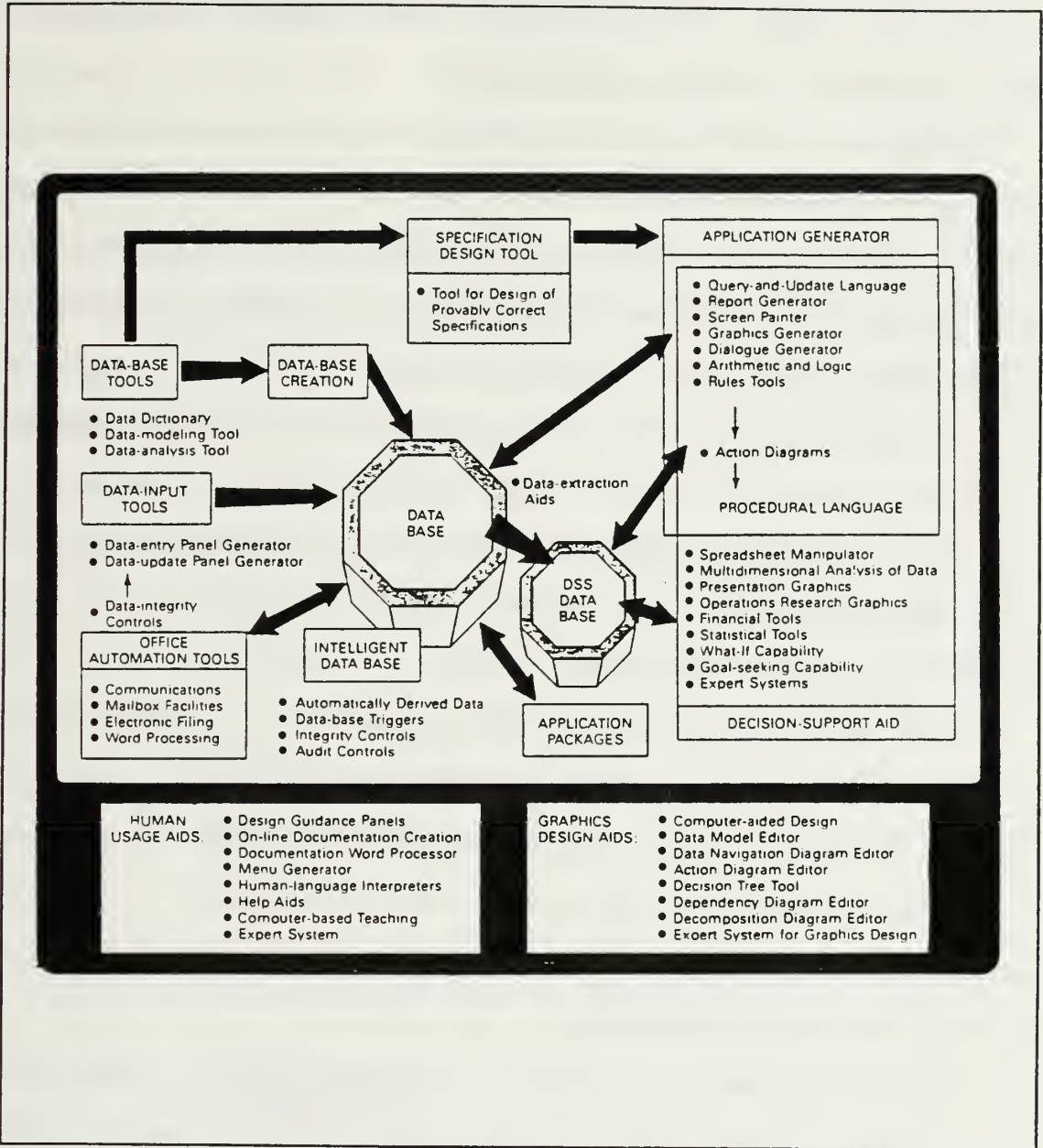
Figure 3.1 An Ideal Fourth Generation Language Facility (Martin, 1985, p. 369)
