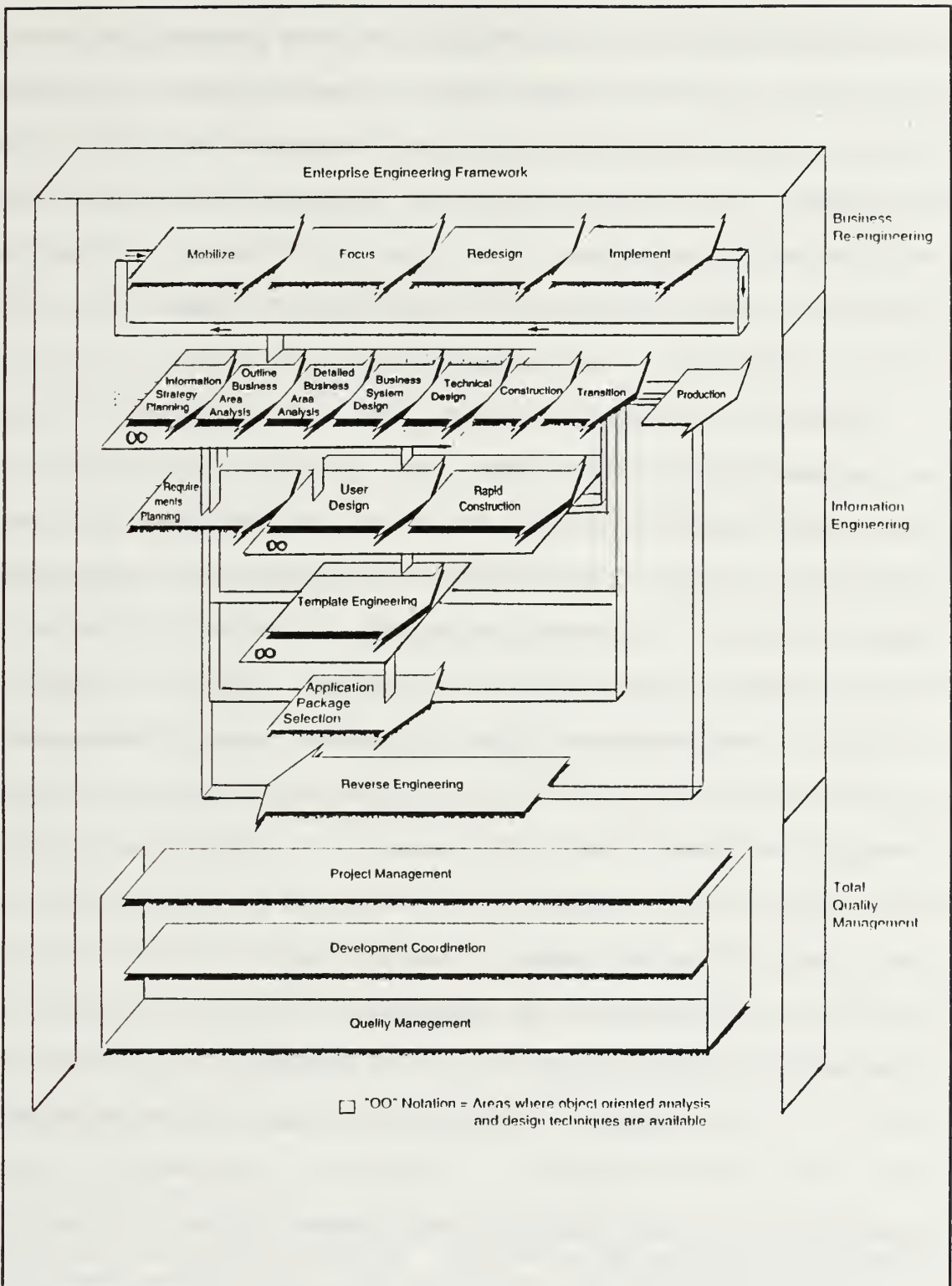
Figure 2.4 Enterprise Engineering Framework (James Martin & Co., 1992, p. 2)
