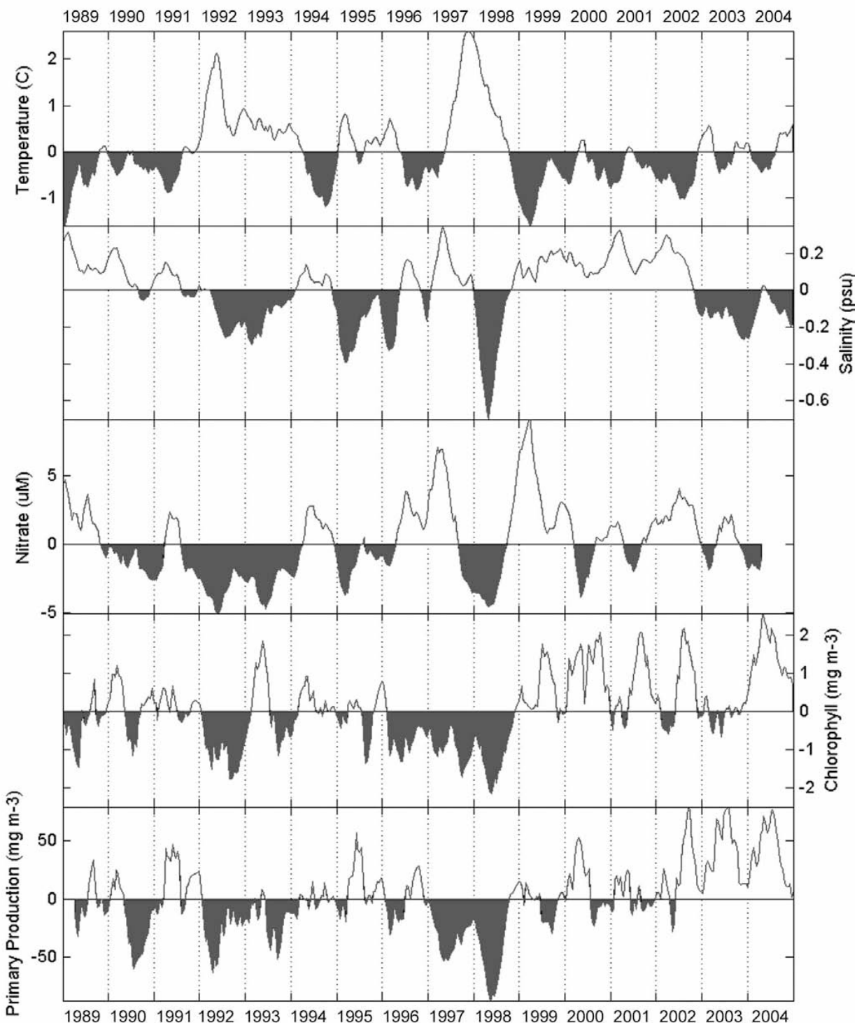
Figure 12. Anomaly plot of sea surface temperature, salinity, nitrate, chlorophyll, and primary production collected as part of the Monterey Ocean Timeseries Observatory (MOTO) program maintained by MBARI. Temperature, salinity, and nitrate were near-normal in 2004, but chlorophyll and primary production were high. As part of MOTO, three to four stations in Monterey Bay and the contiguous waters of the California Current System are sampled every three weeks. The data from all stations are averaged and the averages used to calculate a mean annual cycle. The annual mean cycle is subtracted from a smoothed time series of the data and the anomalies presented in the figure.
