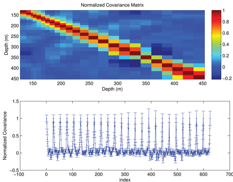
FIG. 15. Normalized depth covariance matrix of spicy sound speed fluctuations are shown in the upper panel. The lower panel shows the same matrix but the matrix has been unwrapped and error bars are shown.
