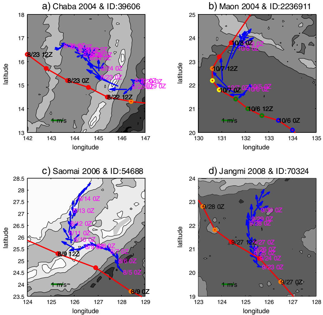
Fig. 3. Four storms' paths and observed current vectors, both in 6-hourly interval.
