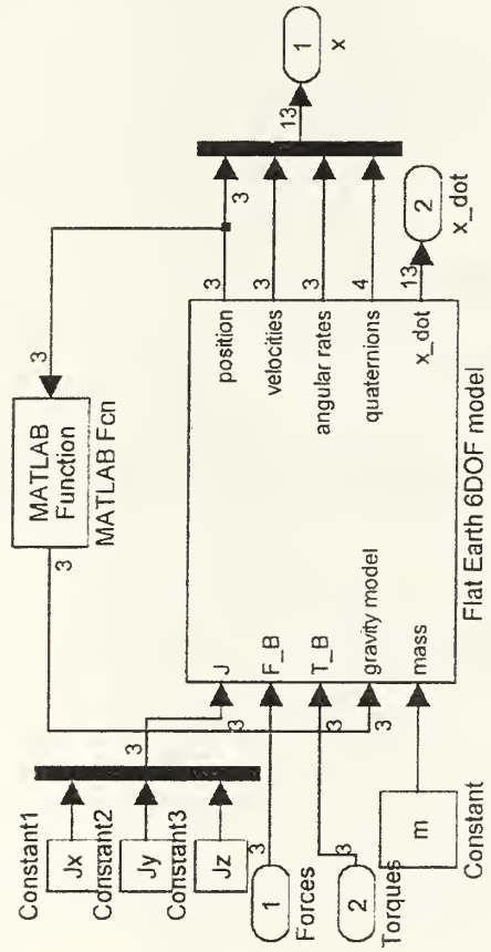
Flat Earth 6DOF Dynamics from Stevens & Lewis "Aircraft Control and Simulation"
