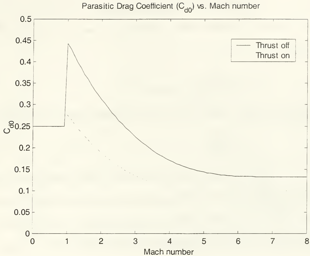
Figure 2.6. Variation of parasitic drag coefficient with Mach number.
