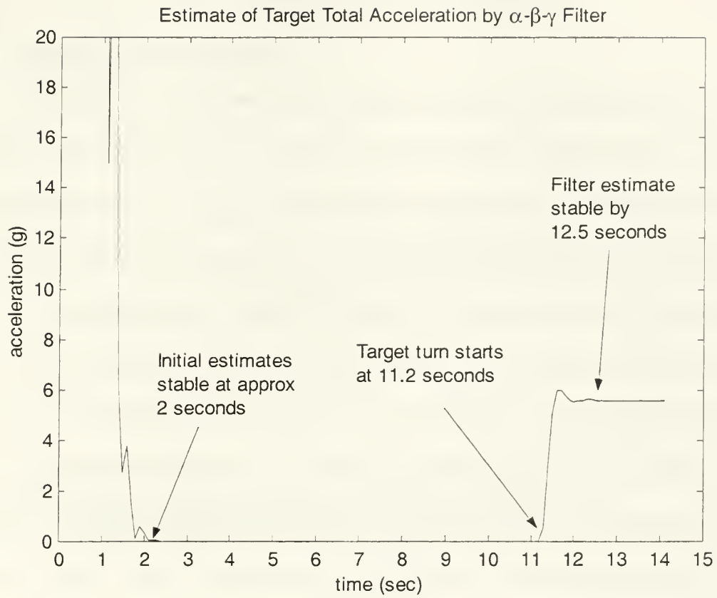
Figure 2.9. \alpha - \beta - \gamma Filter Performance.
