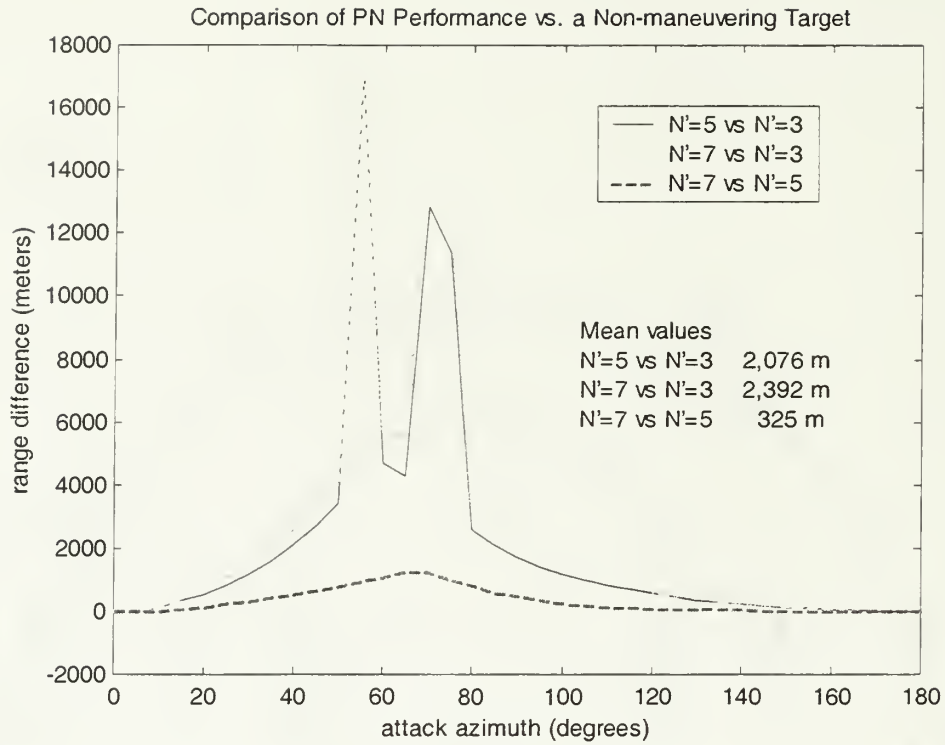
Figure 4.3. PN law performance vs. non-maneuvering target.
