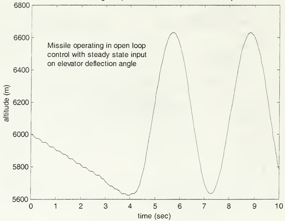
Missile Altitude vs. Time 2.25 degree up elevator, 1000 m/s initial velocity
