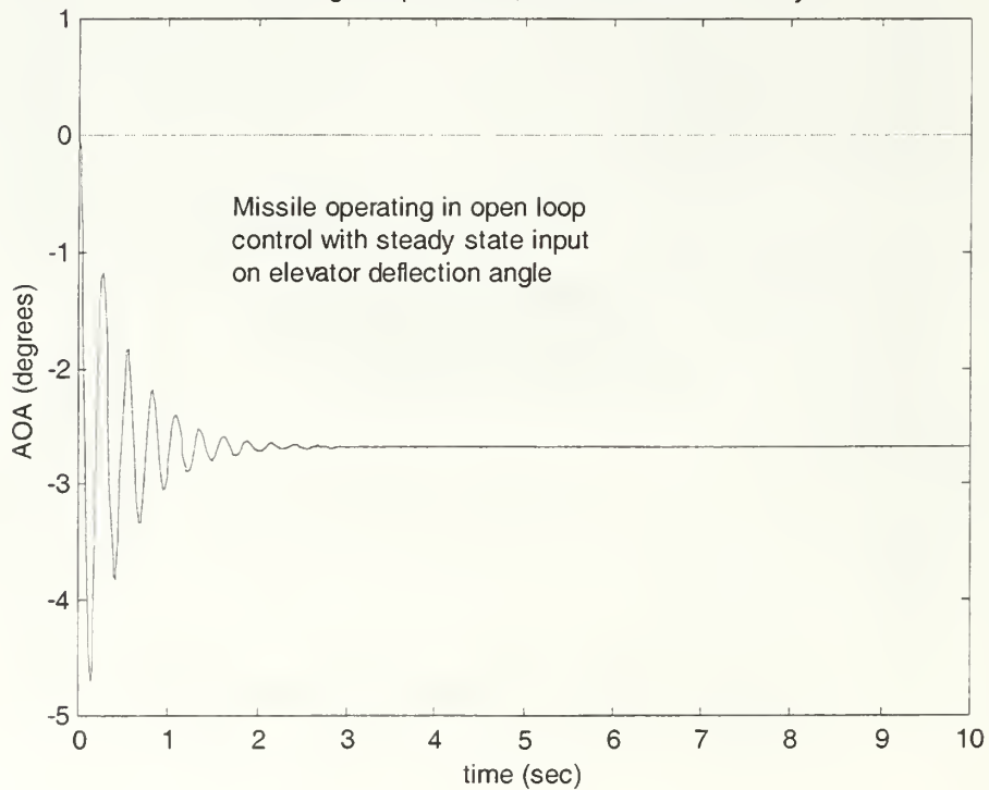
Angle of Attack Response 2.25 degree up elevator, 1000 m/s initial velocity
