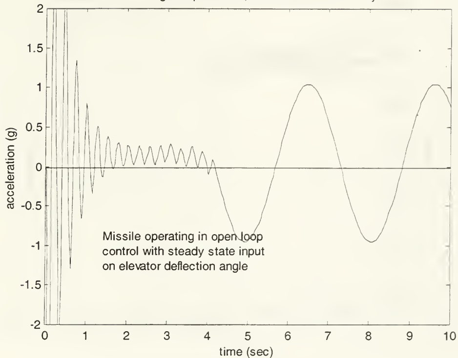
Vertical Acceleration Response 2.25 degree up elevator, 1000 m/s initial velocity
