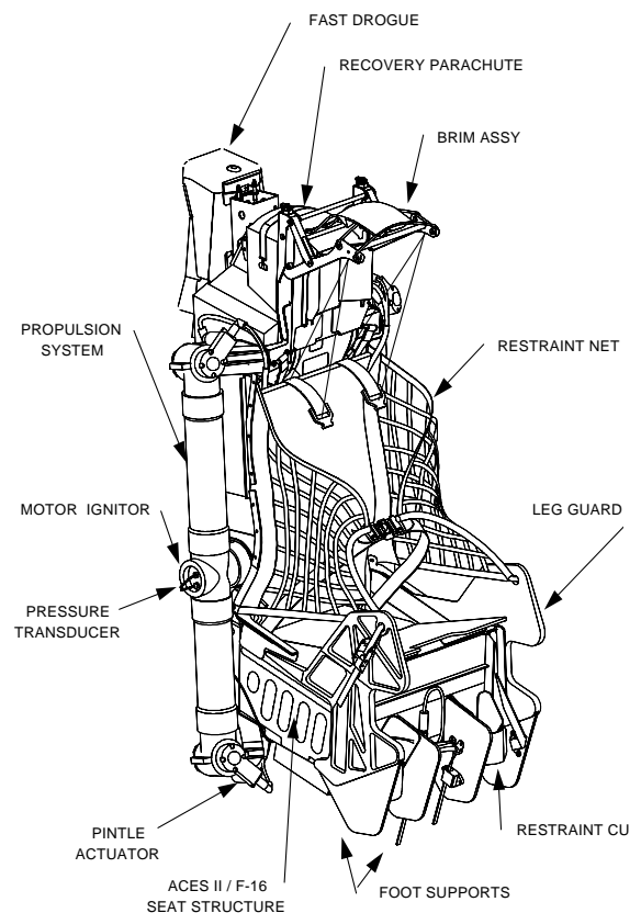
Figure 9.12 Demonstration Seat
