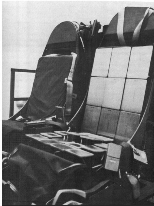
Figure 3. G Seat (seat cover removed)
