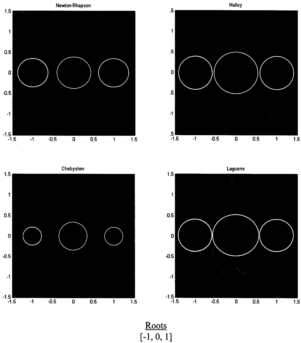
Figure 4.4. Equally Spaced Roots – 3 rd Order
