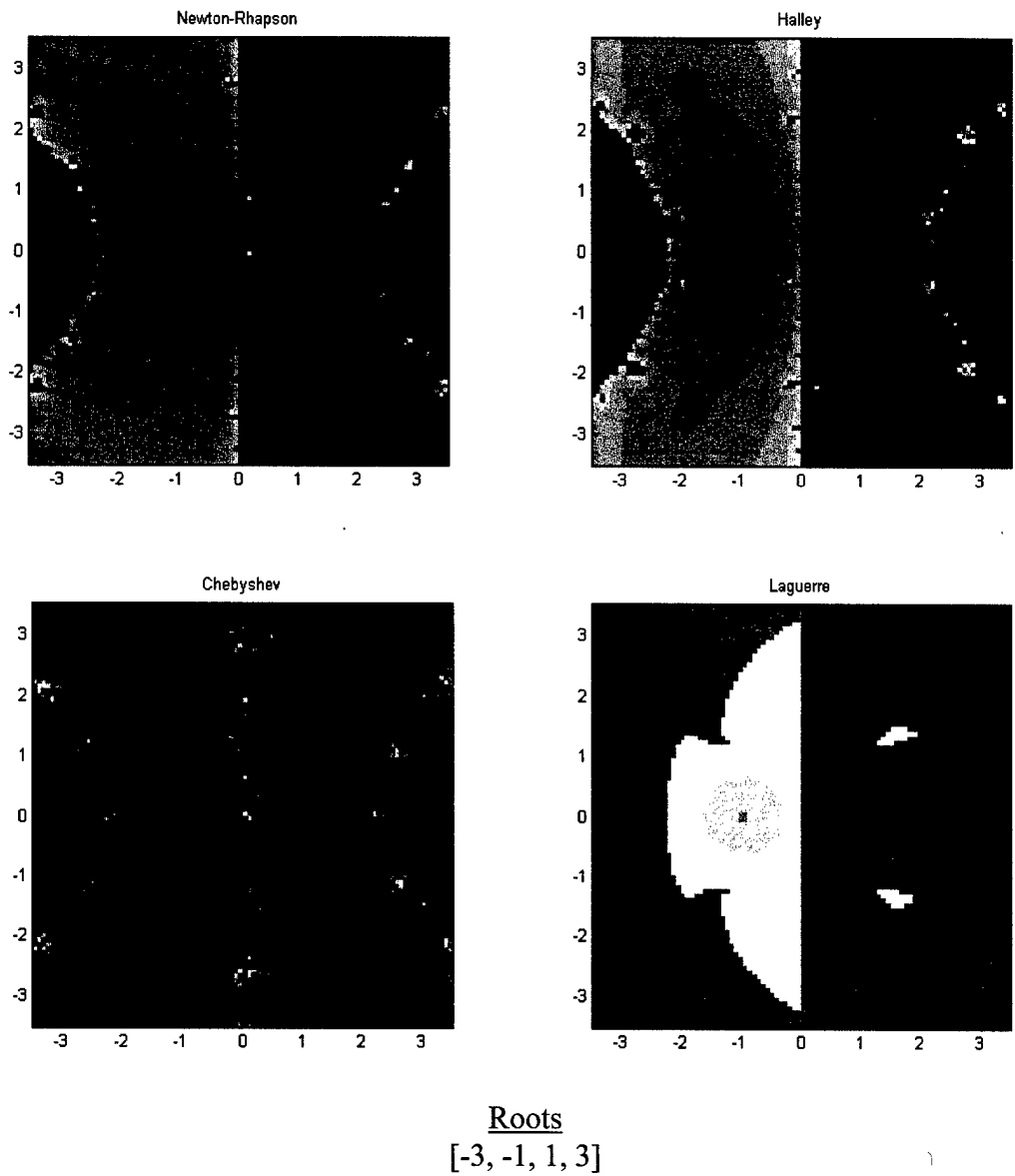
Figure 4.5. Equally Spaced Roots – 4 th Order
