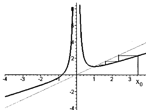
Figure 3.2. Newton-Rhapson Method
