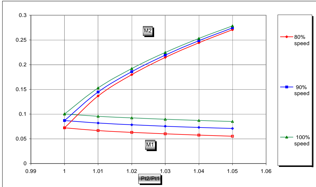
Figure 7. Mach number variation with pressure distortion parameter \pi (\alpha=0.08, \nu=1.05)
