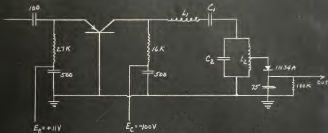
FIG. 21. Circuit of 23mc amplifier used for testing high frequency response of transistors
