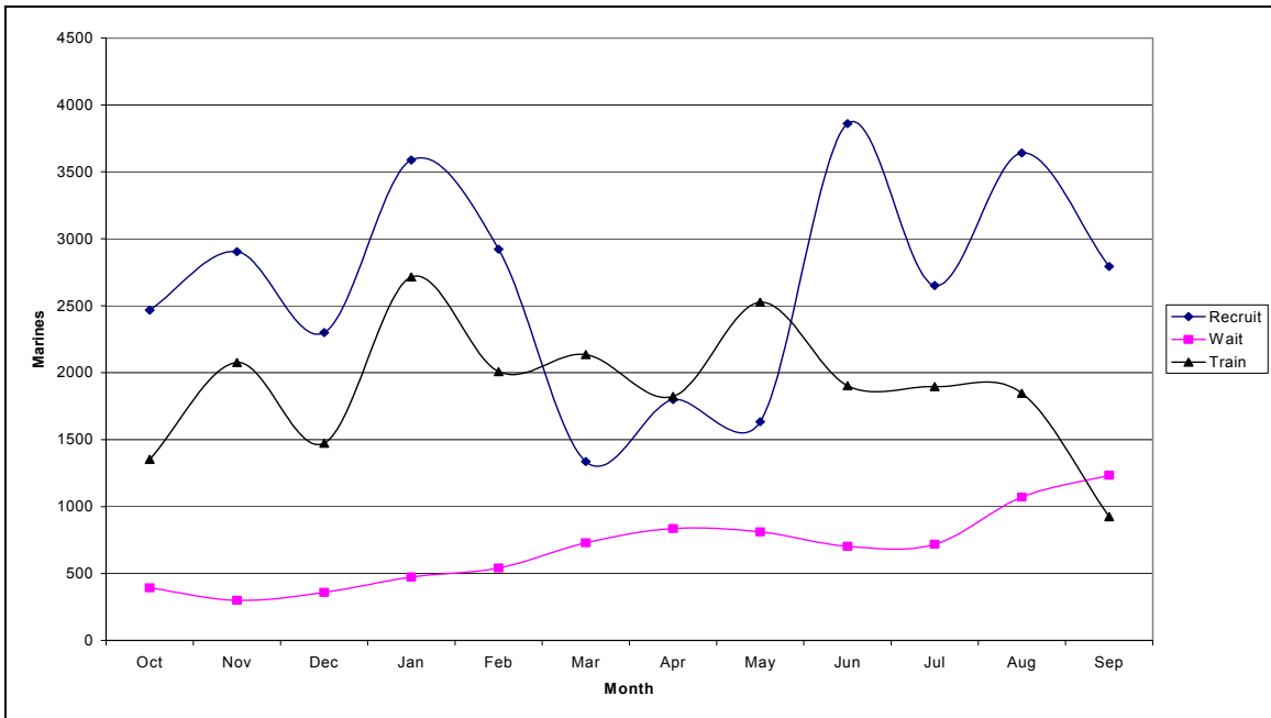
Figure 9. LRAMS Flow Relations. The number of Marines recruited effects the numbers training and waiting after dampening and time delay. For example, the January recruiting surge causes a less dramatic training surge in May. Recruiting surges are greatly dampened in training response and numbers waiting for training four months later. The plotted values are summations of the variables by month for fiscal year 2001.
