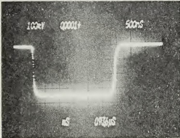
Figure 86 - A STATION TRANSMITTED RANGE PULSE
