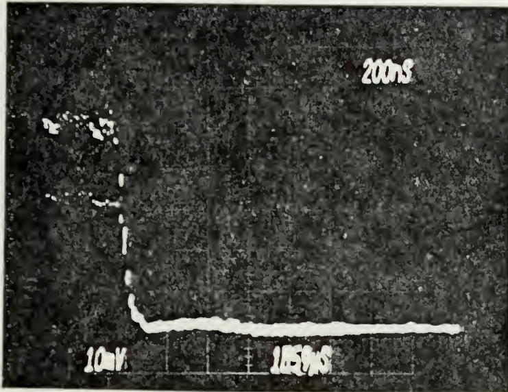
Figure 91 - RANGE PULSE DETECTED AT THE A STATION ANTENNA CONFIGURATION A-18 INCHES, RANGE 298 M
