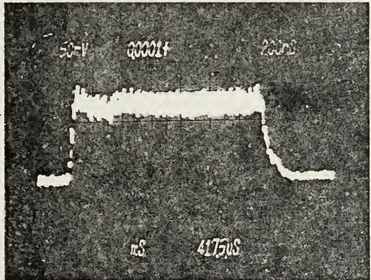
Figure 35 - EXPANDED RANGE PULSES
