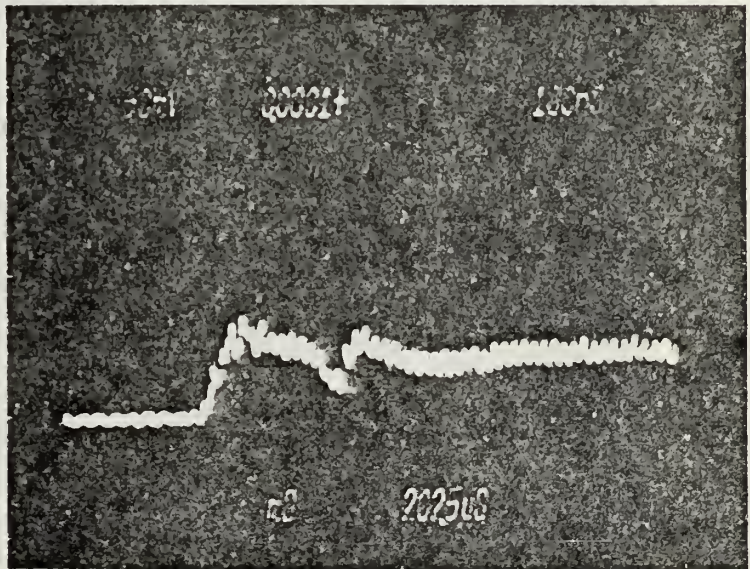
Figure 62 - SEVERE RANGE PULSE DISTORTION
