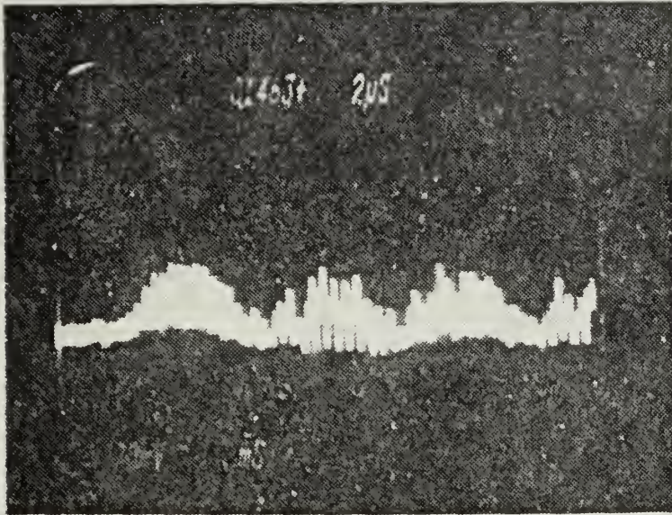
Figure 66 - DISTORTED SCOM MESSAGE BITS
