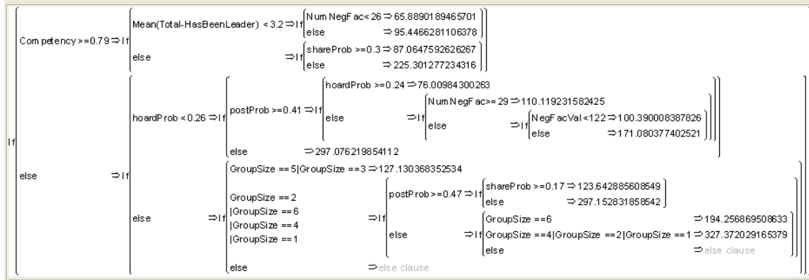
Figure 27. Prediction Rules From Partition Model
