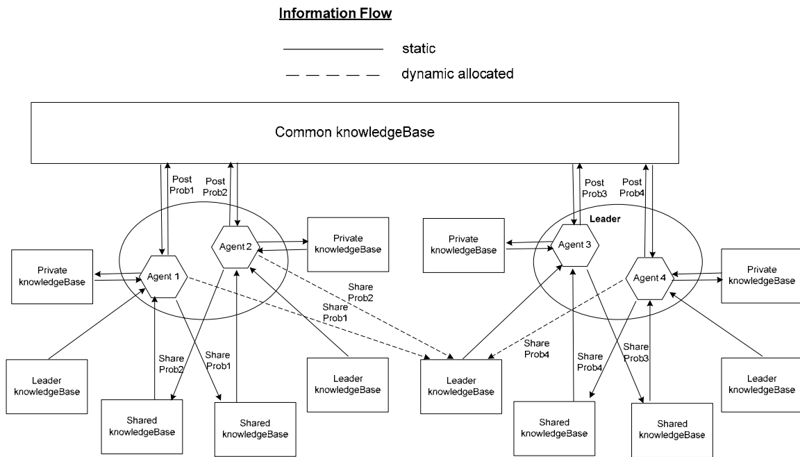
Figure 6. Information Flow Diagram in the Edge Model
