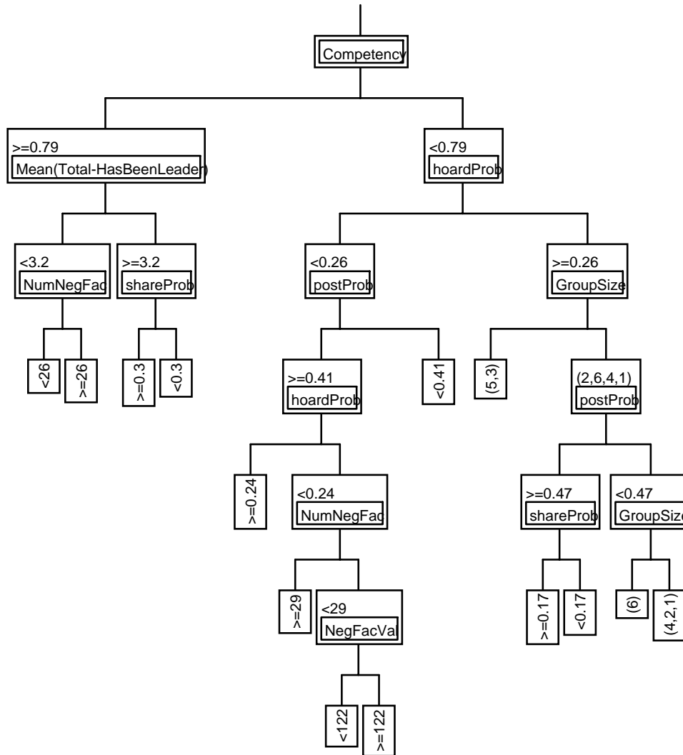
Figure 26. Partition Small Tree view
