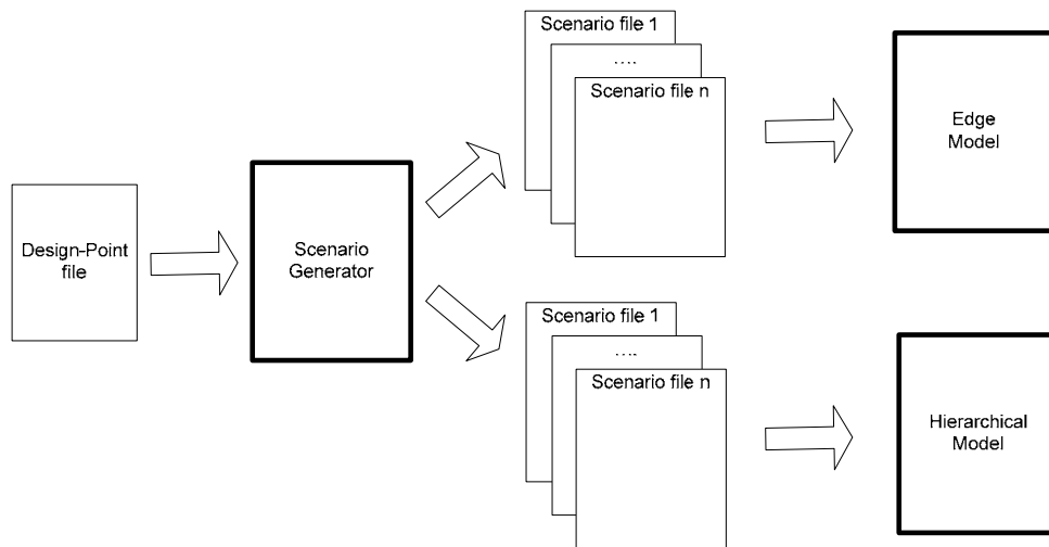
Figure 3. Scenario Generator and Scenario Files
