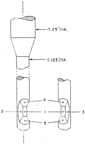
Figure 7. Five-hole probe schematic
