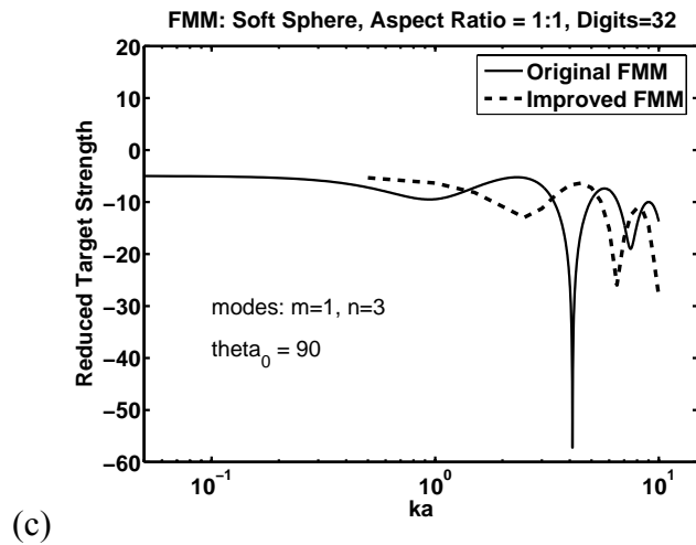
Figure 8. Modes m=1, n=1 ; m=1, n=2 ; and m=1, n=3 for the original FMM and improved FMM with digits=32 for a soft sphere. At digits=32 , the improved FMM runs at twice the precision of the original FMM.
