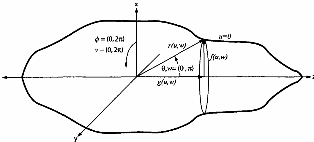
Figure 2. Geometry for an irregular, axisymmetric, finite-length body of revolution. In this case, the body is symmetric about the z-axis. This figure shows the geometry for both spherical coordinates and an orthogonal, conformally mapped coordinate system. (From Reeder and Stanton, 2004)
