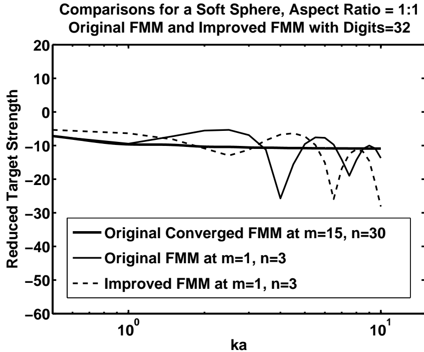
Figure 14. Comparison of mode m=1, n=3 of the original FMM and of the improved FMM at digits=32 to the converged solution of the original FMM. The first null space is reached at ka=3.8 for the original model, while the improved FMM shifts the first null to ka=6.5 .
