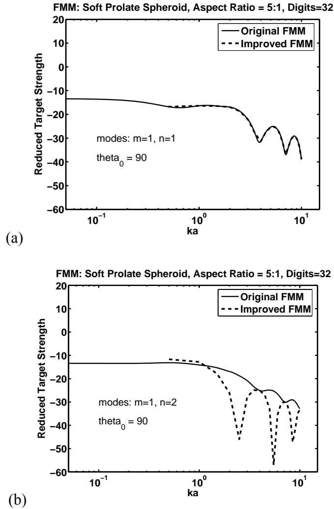
Figure 9. Modes m=1, n=1 and m=1, n=2 for the original FMM and improved FMM with digits=32 for a prolate spheroid with AR=5:1 . These plots show distinct differences between the two models for these modes. The identical curves in window (a) give confidence that VPA and other techniques were implemented correctly. Precision of digits=32 is approximately double the precision of the original FMM.
