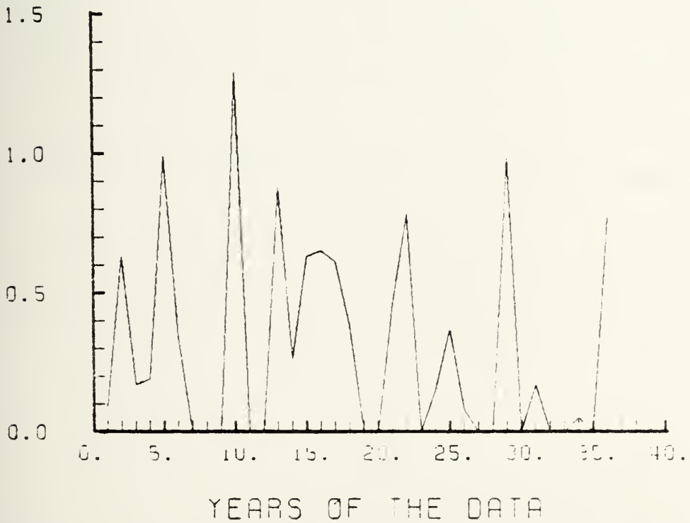
Figure 58. Weekly rainfall in inches for weeks A3 and A4
