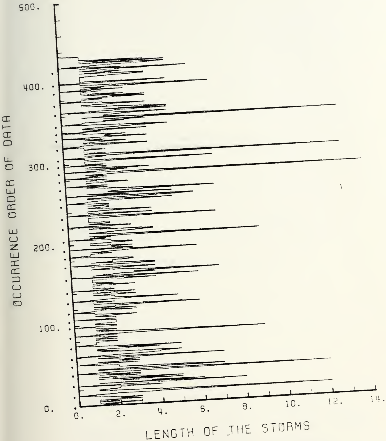
Figure 3. Time series plot of the LS for December-February.
