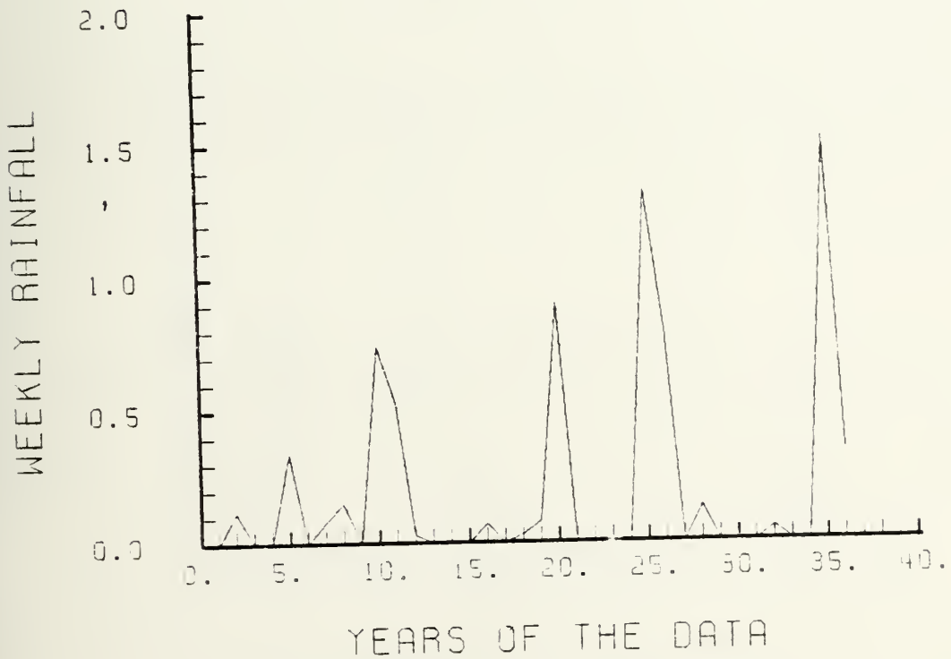
Figure 44. Weekly rainfall in inches for weeks 01 and 02
