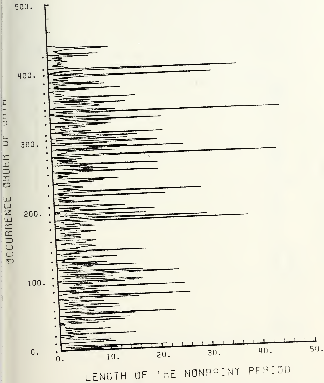
Figure 5. Time series plot of the LN for December-February.
