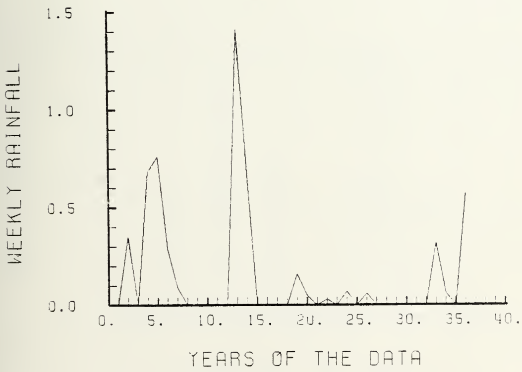
Figure 45. Weekly rainfall in inches for weeks 03 and 04
