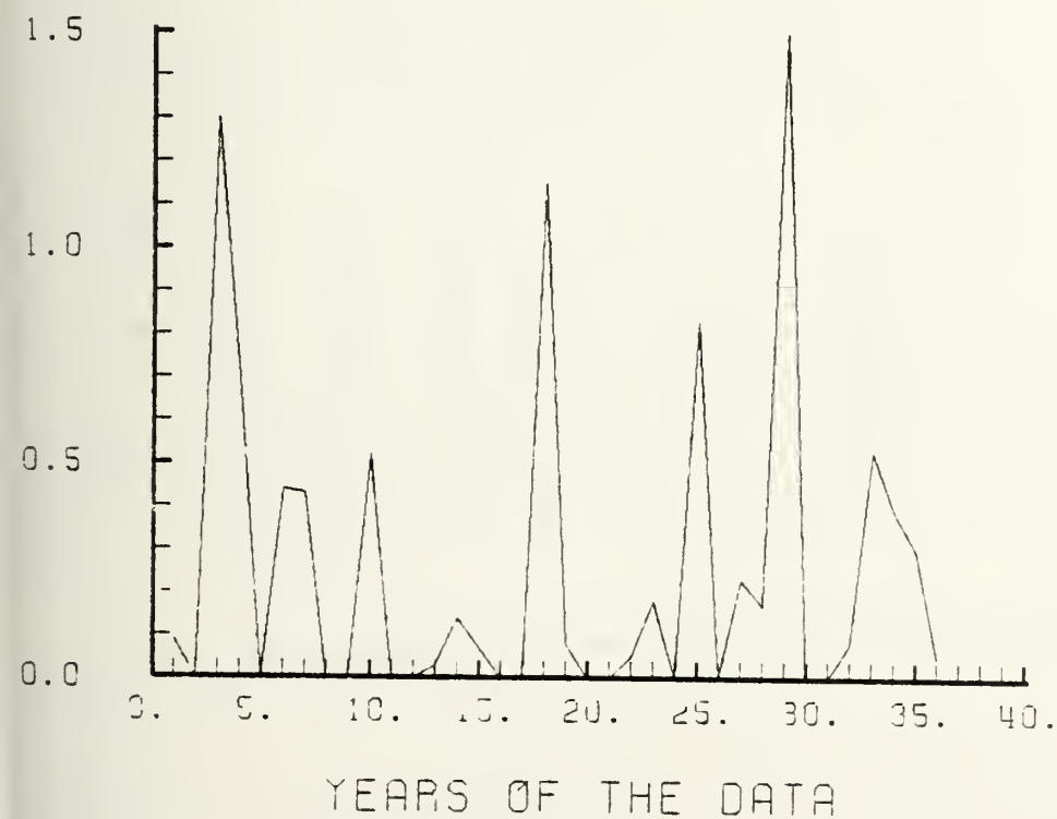
Figure 57. Weekly rainfall in inches for weeks A1 and A2
