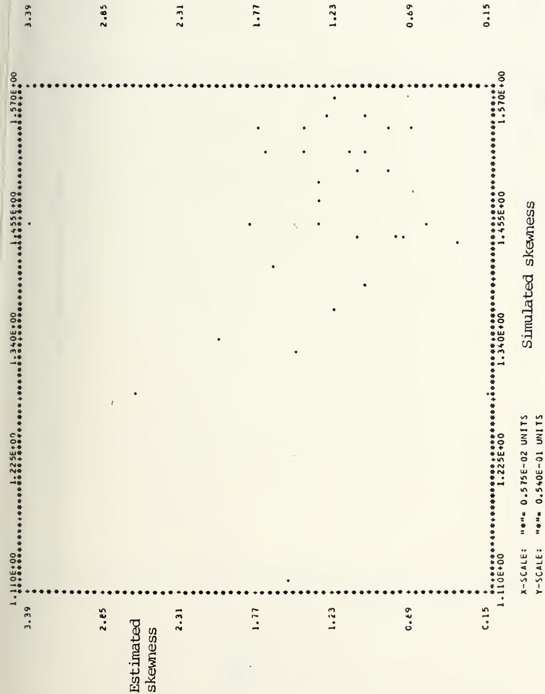
Figure 21. Plot of estimated skewness against simulated skewness for the positive weekly rainfall
