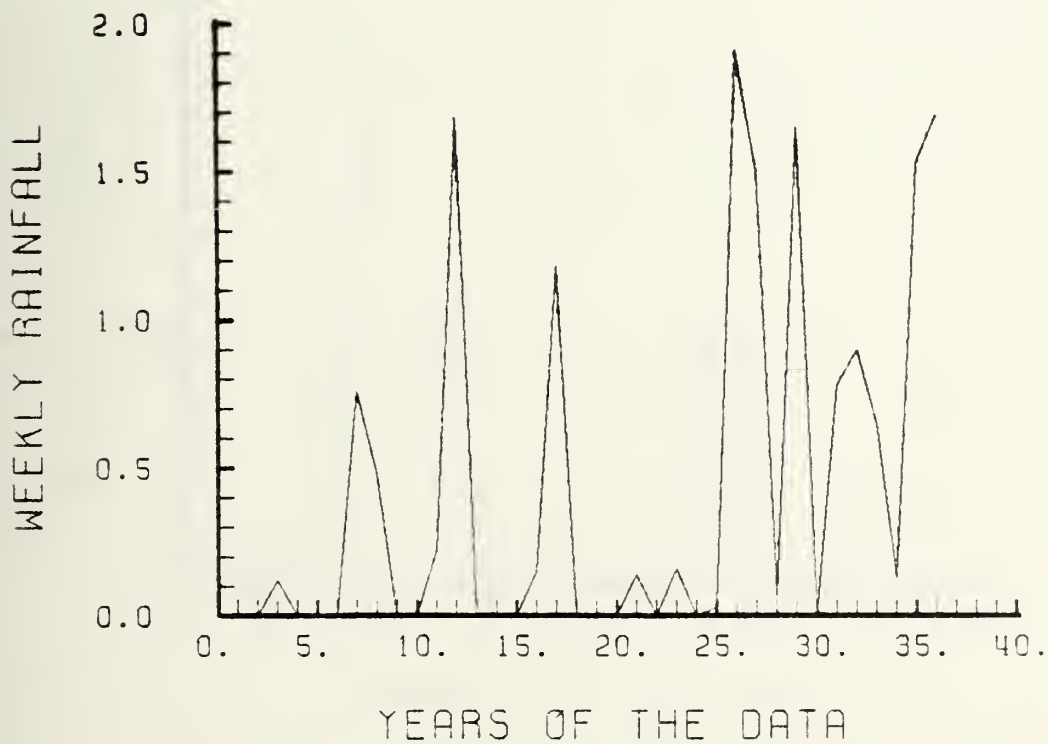
Figure 46. Weekly rainfall in inches for weeks 0N and 0N1
