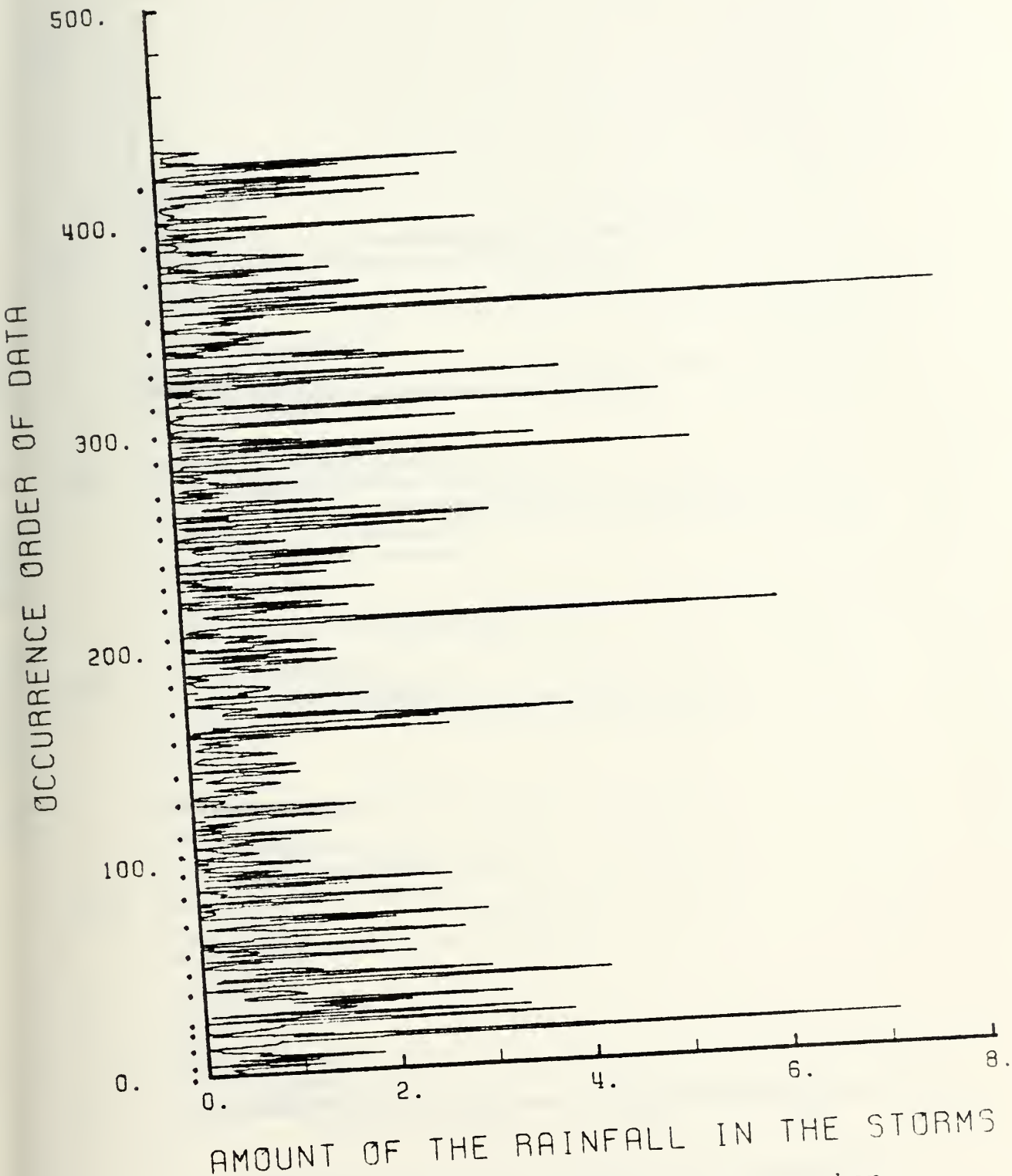
Figure 4. Time series plot of the AR for December-February.
