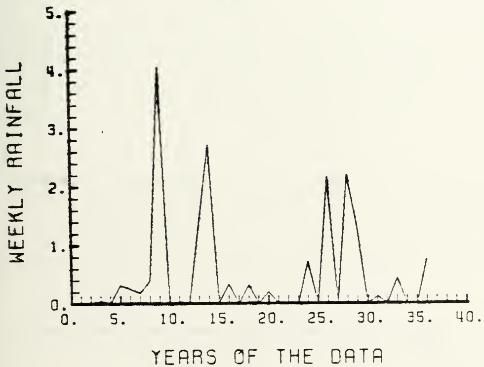
Figure 47. Weekly rainfall in inches for weeks N2 and N3
