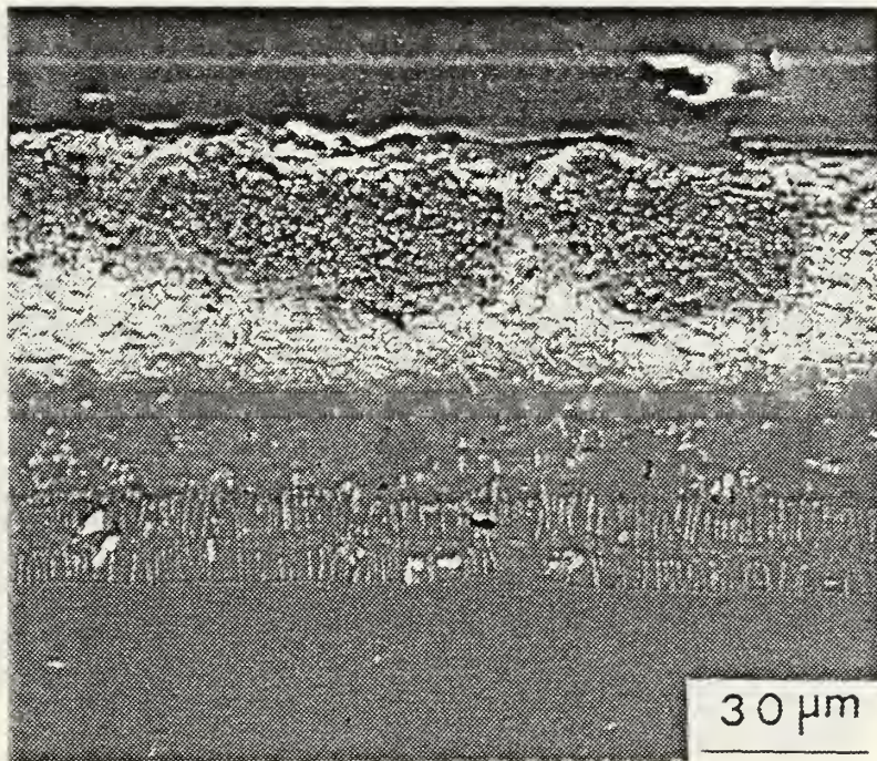
Figure B.10b HTLA Platinum-Aluminide / IN-100 (LTHC-100 hrs).
