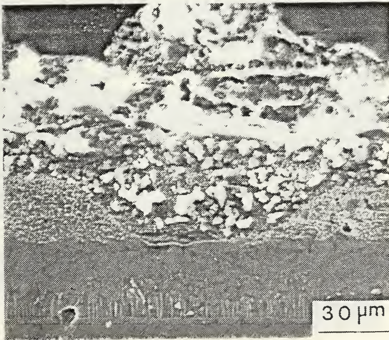
Figure B.14b Process B / IN-100 (LTHC-100 hrs).
