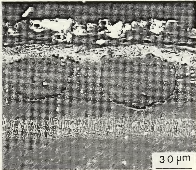
Figure B.2b LPHA Platinum-Aluminide / IN-738 (LTHC-100 hrs).
