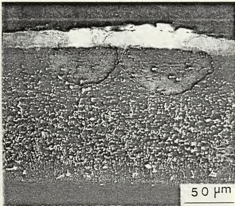
Figure B.8b Process D / IN-738 (LTHC-100 hrs).
