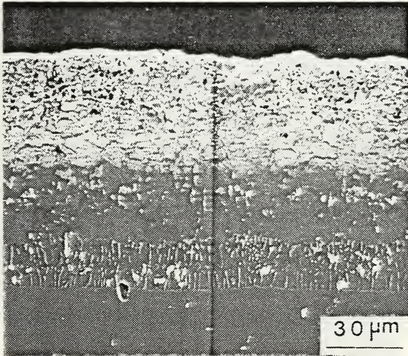
Figure B.10a HTLA Platinum-Aluminide / IN-100 (as-received).
