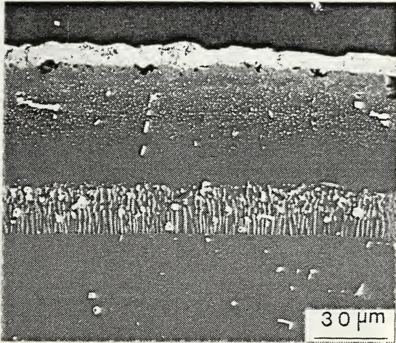
Figure B.2a LPHA Platinum-Aluminide / IN-738 (as-received).
