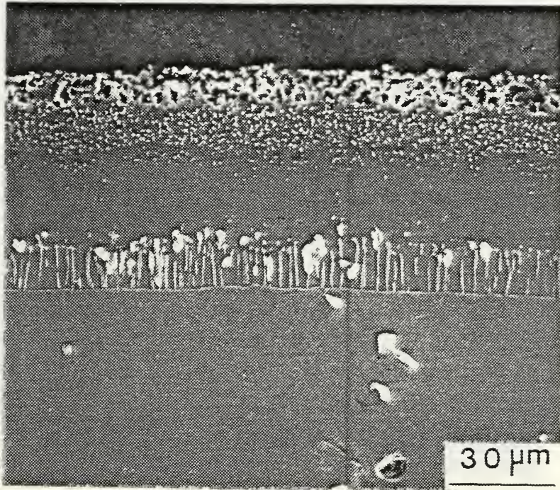
Figure B.12a LTHA Chromium-Aluminide / IN-100 (as-received).
