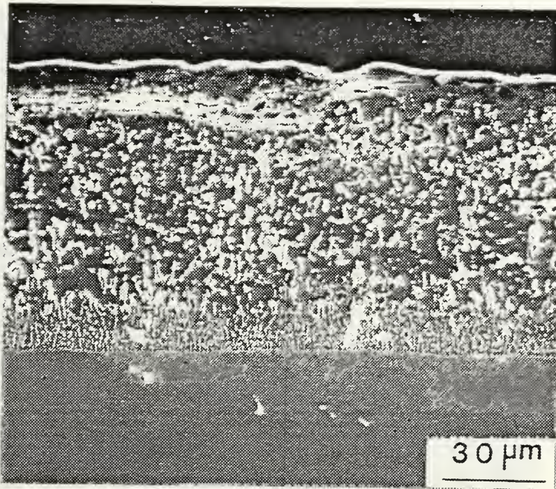
Figure B.6a HTLA Chromium-Aluminide / IN-738 (as-received).
