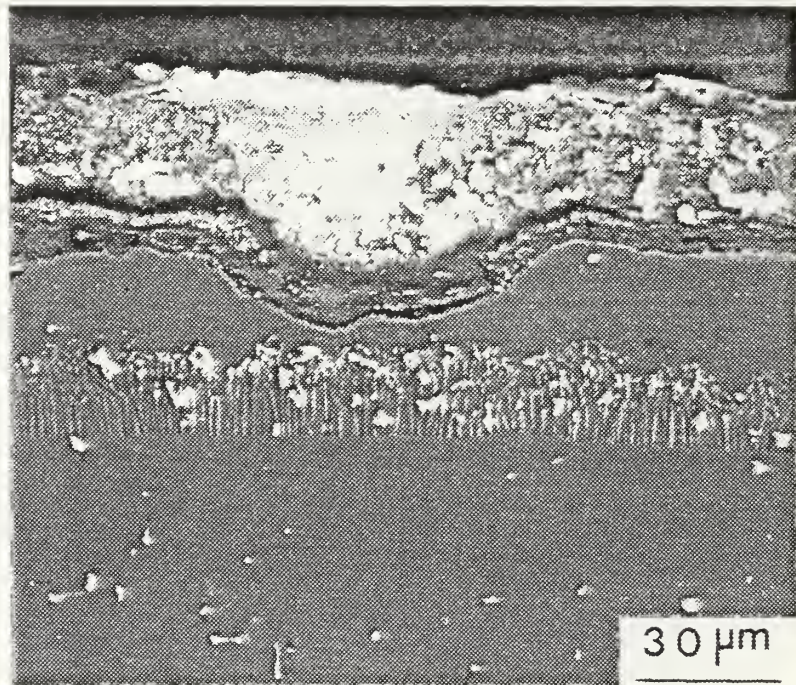
Figure B.7b Process B / IN-738 (LTHC-100 hrs).
