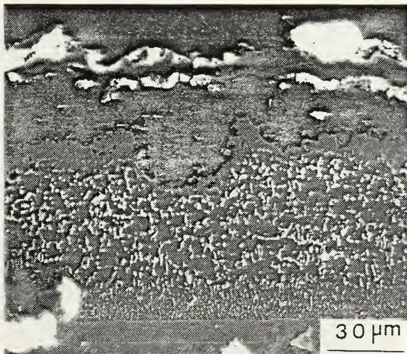
Figure B.6b HTLA Chromium-Aluminide / IN-738 (LTHC-100 hrs).
