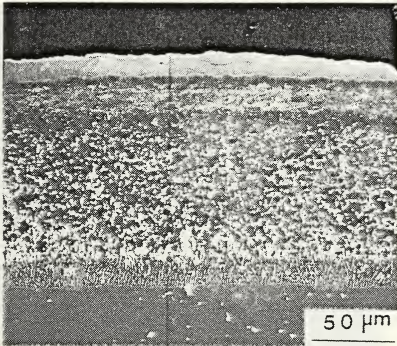
Figure B.8a Process D / IN-738 (as-received).
