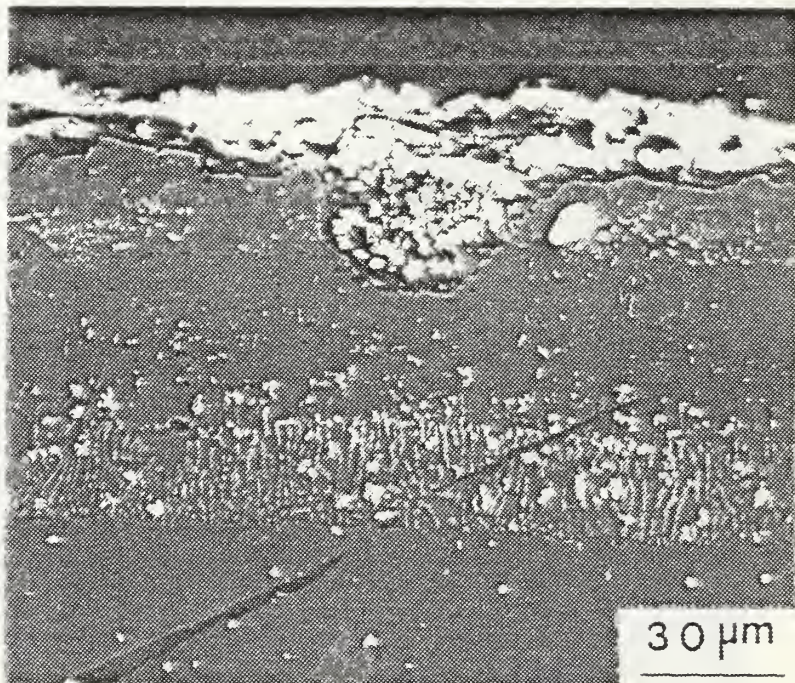
Figure B.3b HTLA Platinum-Aluminide / IN-738 (LTHC-100 hrs).
