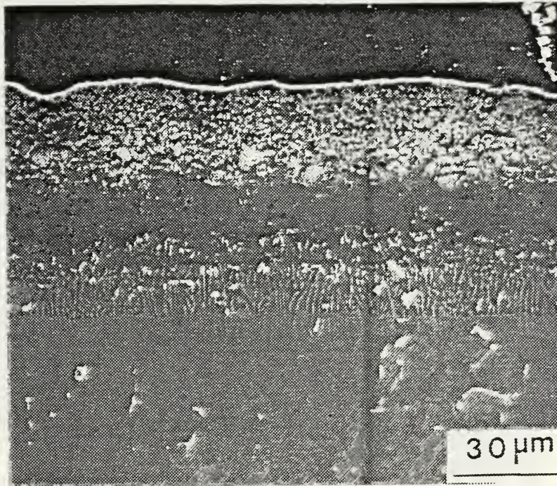
Figure B.4a Process A / IN-738 (as-received).
