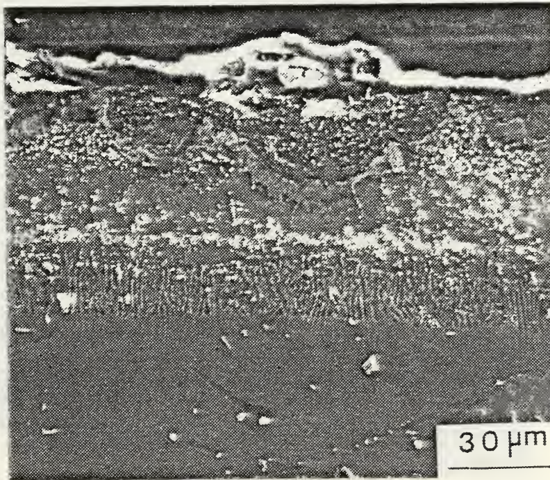
Figure B.4b Process A / IN-738 (LTHC-100 hrs).
