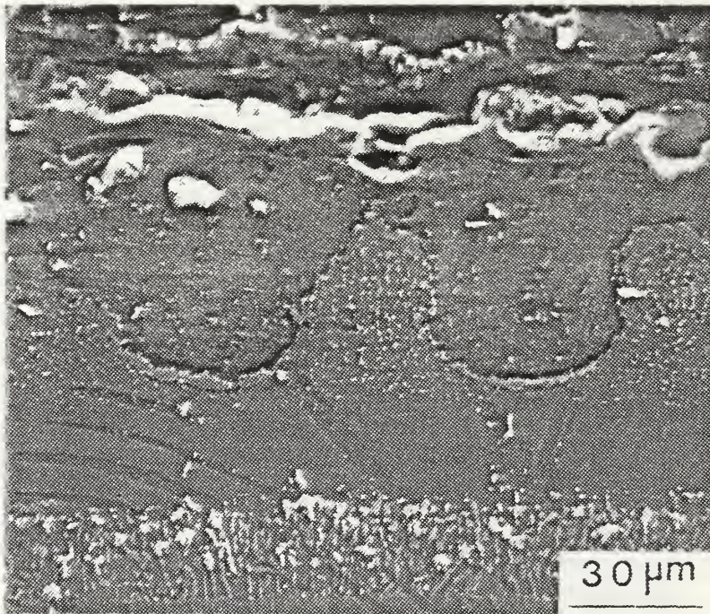
Figure B.5b LTHA Chromium-Aluminide / IN-738 (LTHC-100 hrs).
