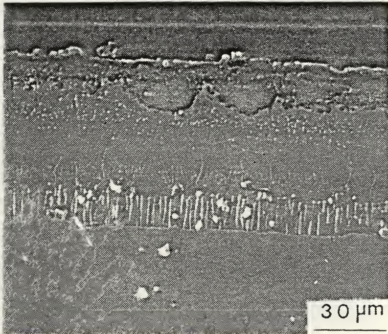
Figure B.12b LTHA Chromium-Aluminide / IN-100 (LTHC-100 hrs).
