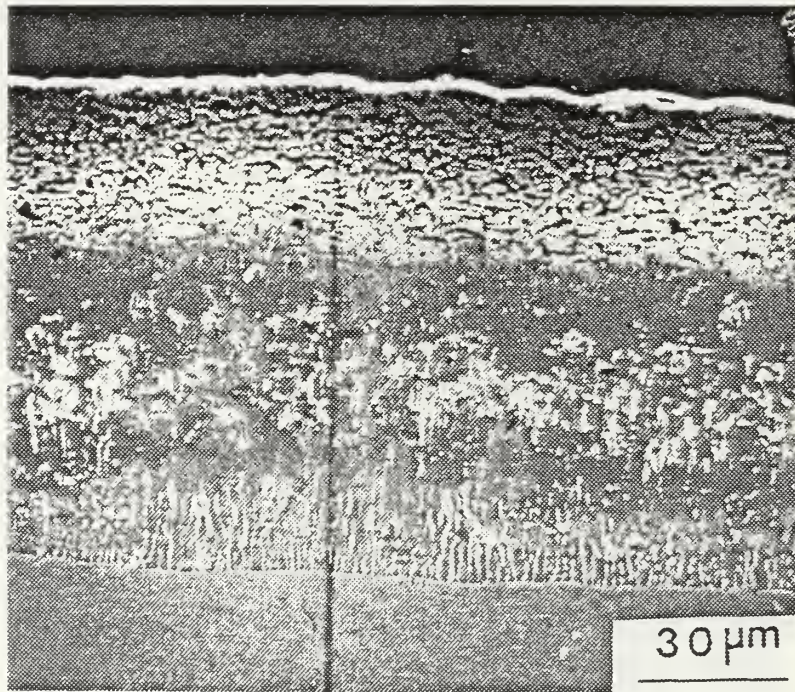
Figure B.11a Process A / IN-100 (as-received).
