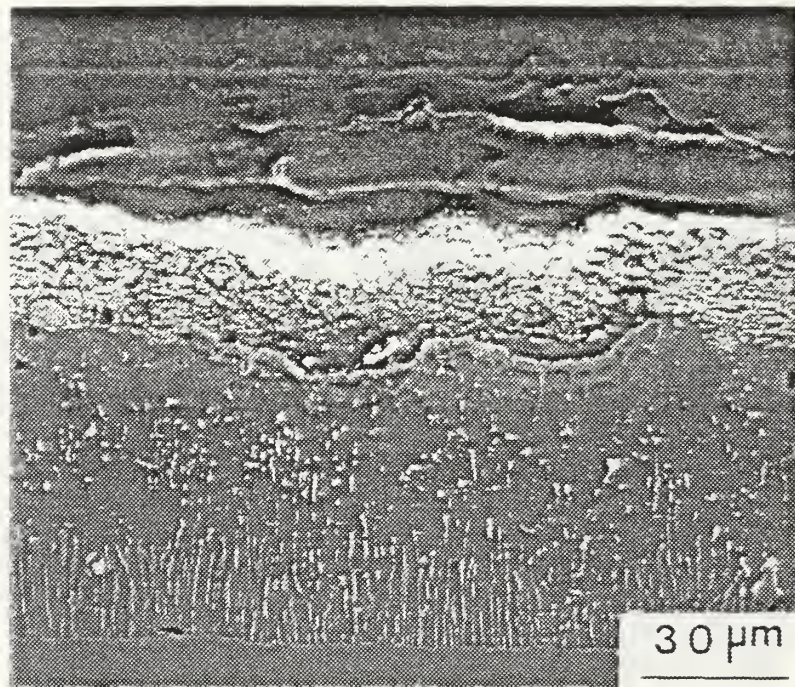
Figure B.11b Process A / IN-100 (LTHC-100 hrs).
