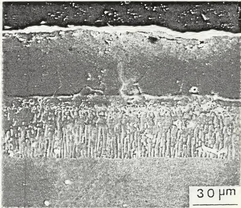
Figure B.15a Process D / IN-100 (as-received).
