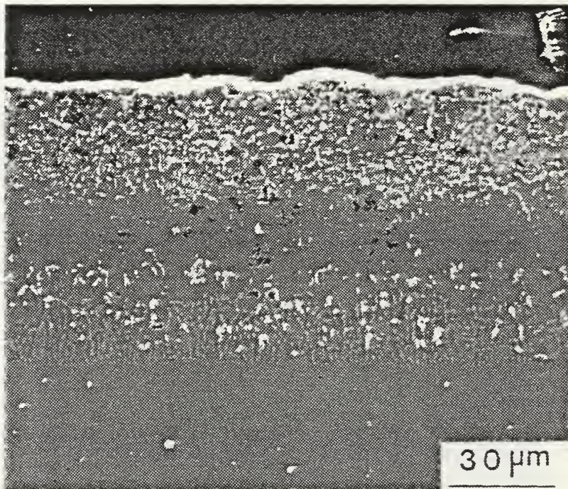
Figure B.3a HTLA Platinum-Aluminide / IN-738 (as-received).
