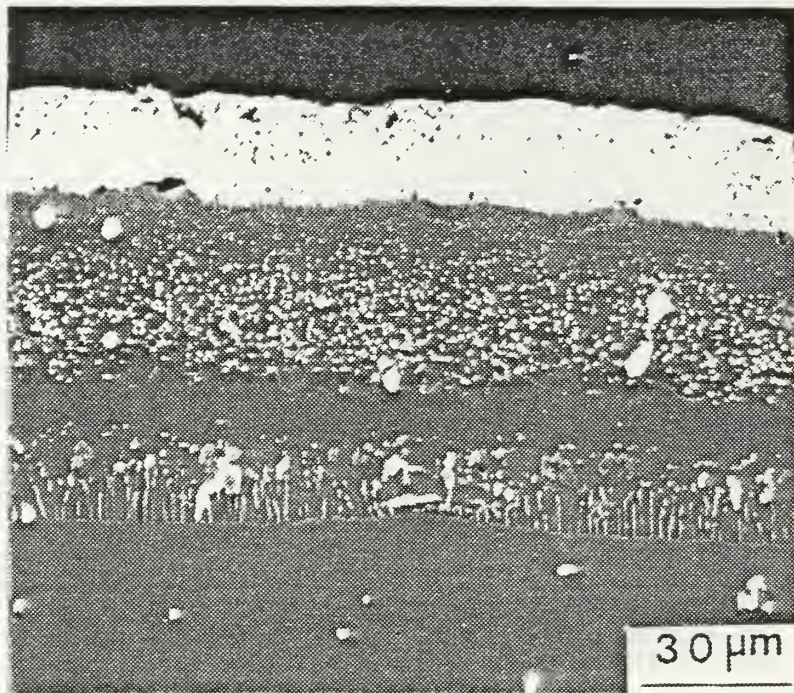
Figure B.9a LTHA Platinum-Aluminide / IN-100 (as-received).
