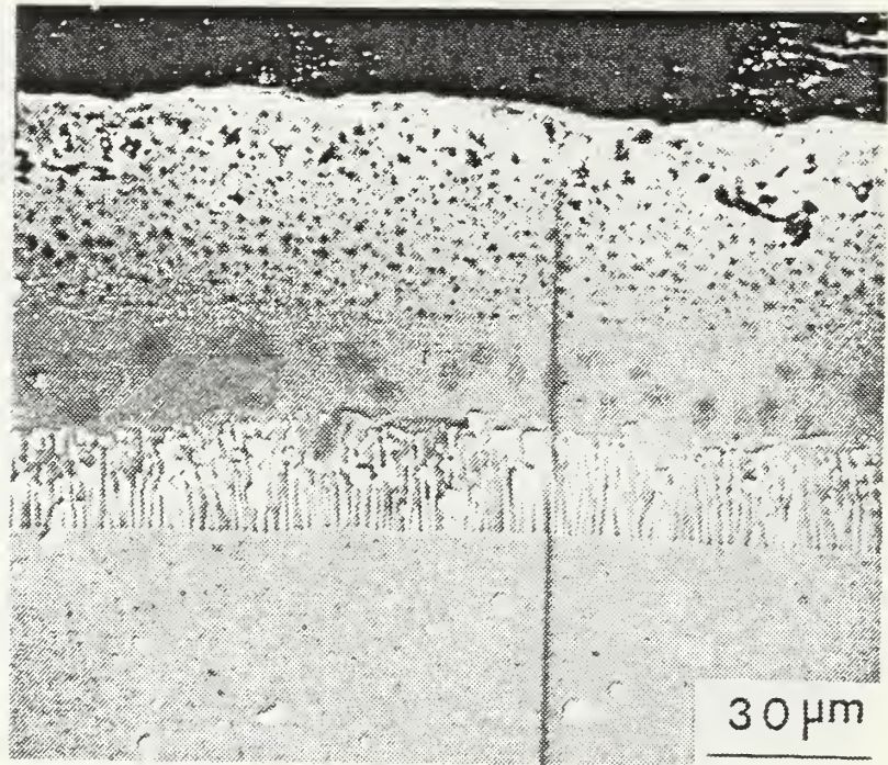
Figure B.7a Process B / IN-73B (as-received).
