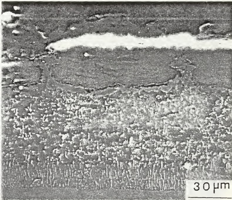
Figure B.13b HTLA Chromium-Aluminide / IN-100 (LTHC-100 hrs).
