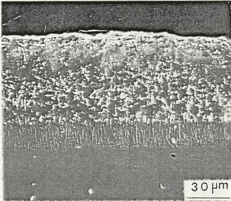
Figure B.13a HTLA Chromium-Aluminide / IN-100 (as-received).
