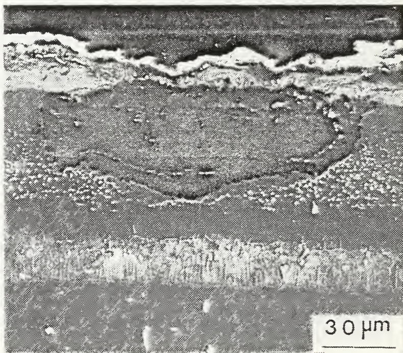
Figure B.9b LTHA Platinum-Aluminide / IN-100 (LTHC-100 hrs).
