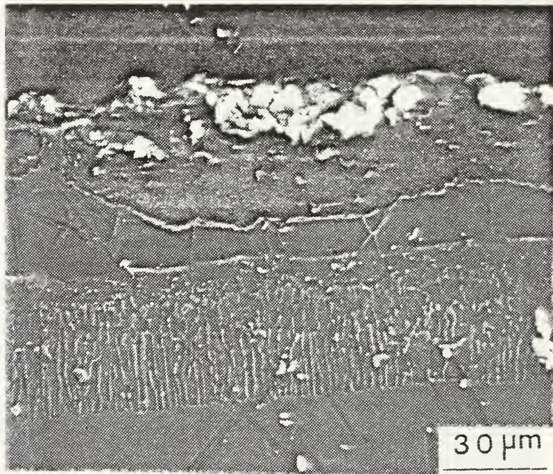
Figure B.15b Process D / IN-100 (LTHC-100 hrs).
