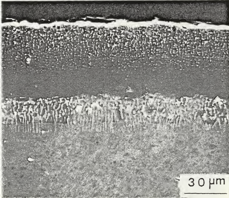
Figure B.5a LTHA Chromium-Aluminide / IN-738 (as-received).
