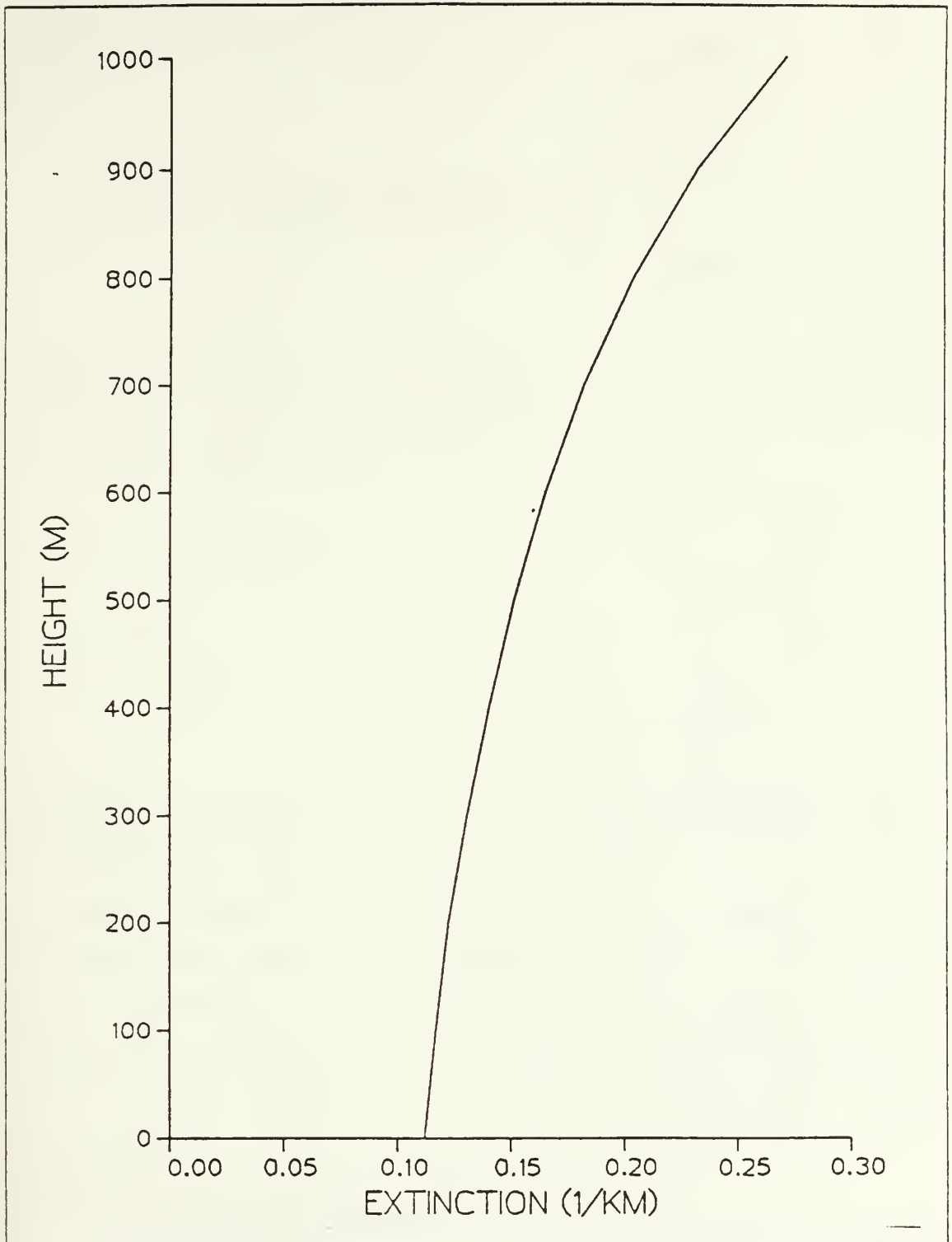
Fig. 3.2 Extinction corresponding to the relative humidity profile in Fig. 3.1.
