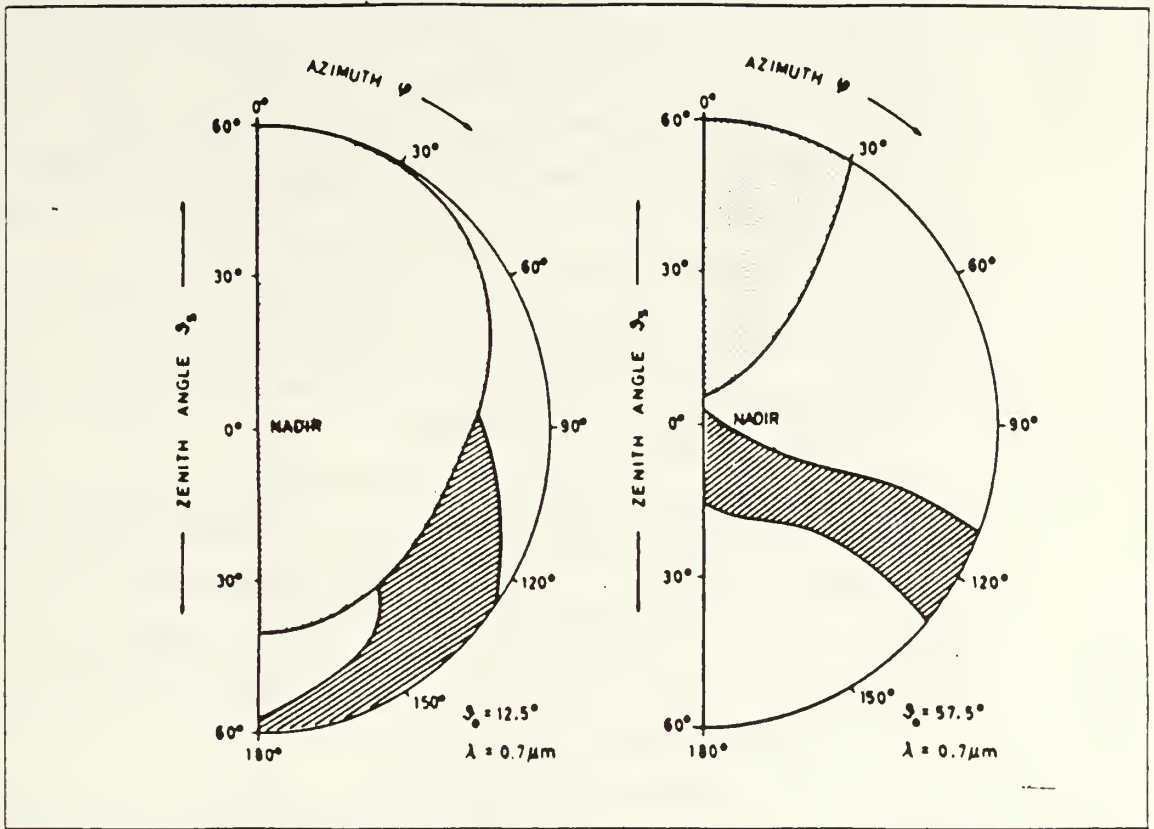
Fig. 2.1 Favorable viewing geometries for atmospheric turbidity with satellite zenith angles of 12.5^\circ (left), and 57.5^\circ (right). (Koepke and Quenzel, 1979).
