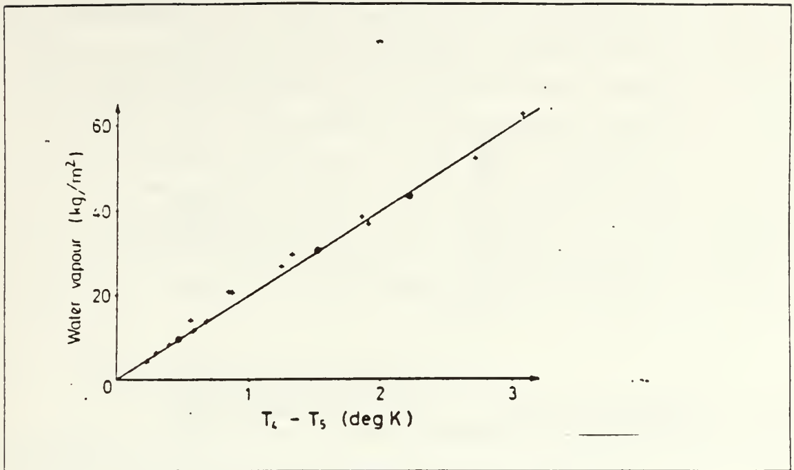
Fig. 2.7 Total atmospheric water vapor ( \text{kg/m}^2 ) as a function of brightness temperature difference (K) from Dalu (1986).
