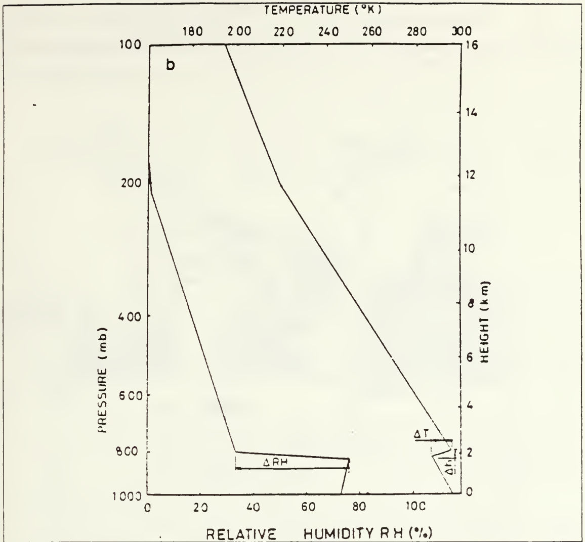
Fig. 2.11 An example of a temperature and relative humidity profile for a typical subsidence inversion. Modified from Nieman (1977).
