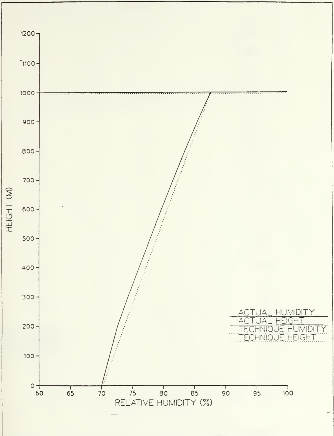
Fig. 4.2 Model and technique produced MABL depths and relative humidities. Model depth = 1000m.
