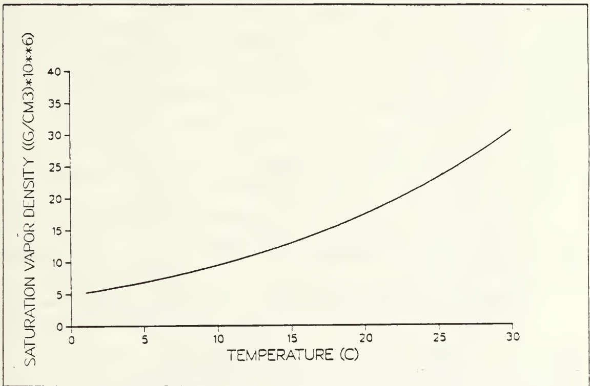
Fig. 2.10 Saturation vapor density ( \text{g/cm}^3 \cdot 10^6 ) as a function of temperature based on Bolton (1980).
