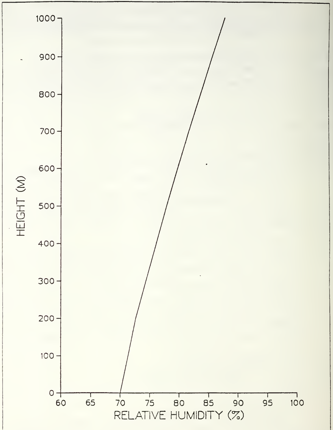
Fig. 3.1 Model relative humidity profile with RH(0) = 70\% and \Delta z = 1000m .
