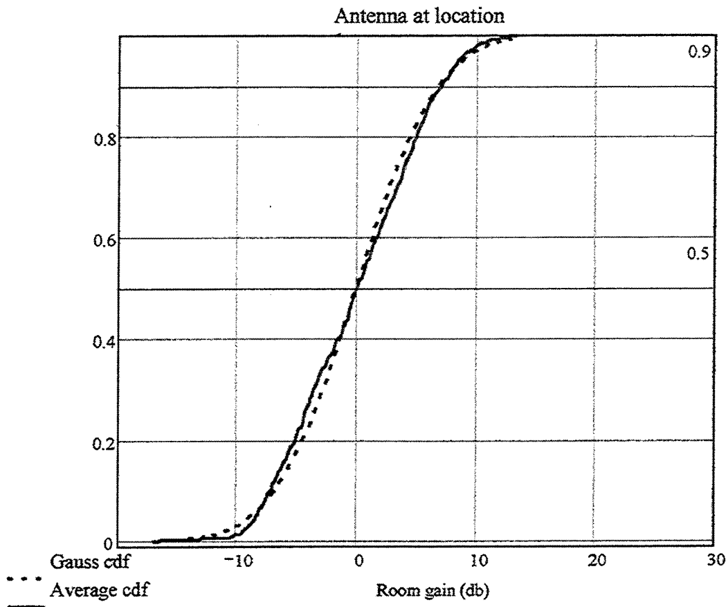
Figure 42. Cdf of the Excess Gain and Lognormal (Gaussian) Cdf, Antenna at Location 1
