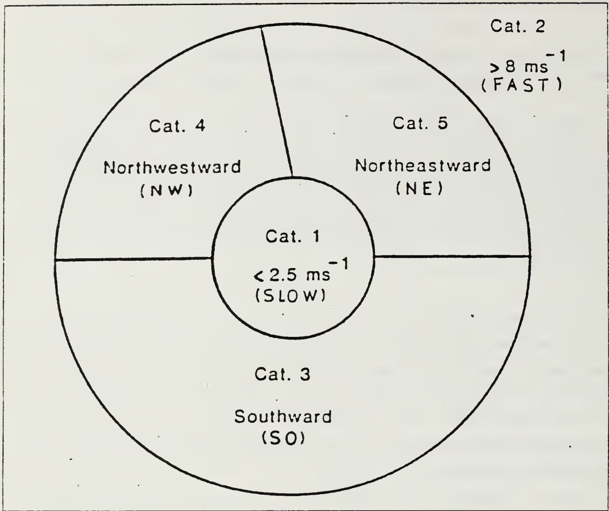
Figure 3.1. Schematic of the five past-motion categories based on the prior 12-h speed and direction classification by Elsberry and Peak (1986).
