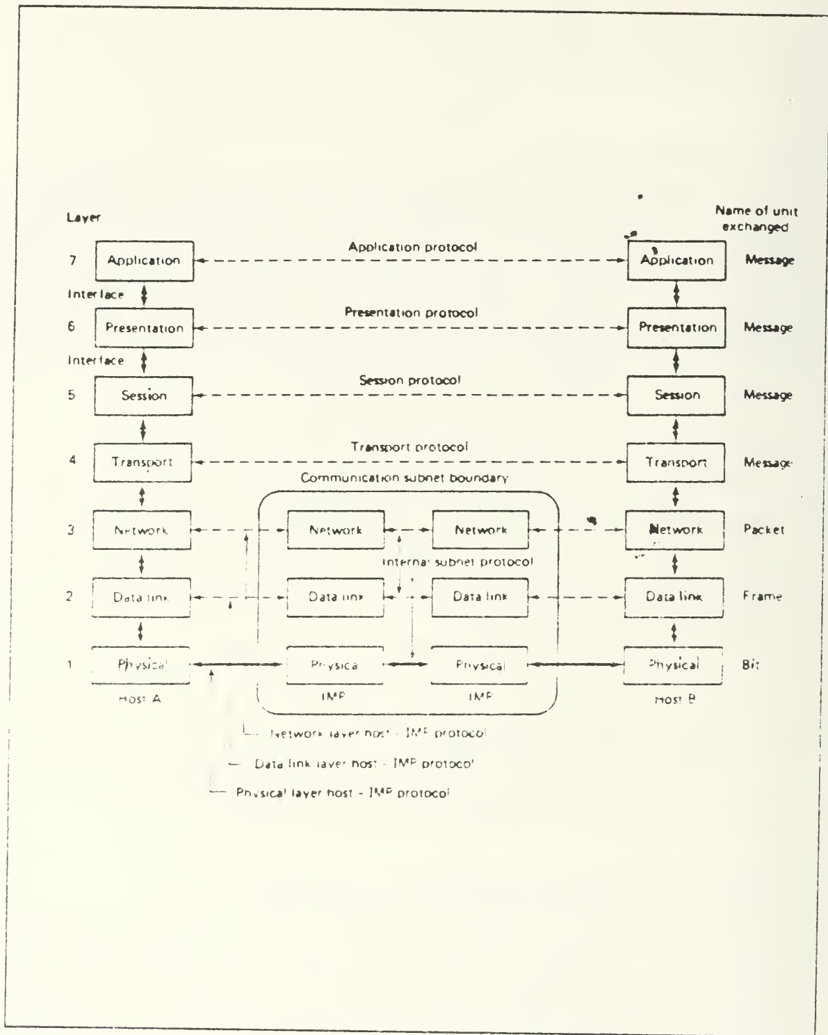
Figure 3. The Open Systems Interconnection Model for Standard Communication Protocols
