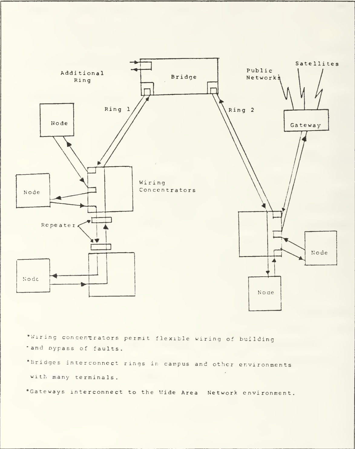
Figure 11. Token-Ring Architecture
