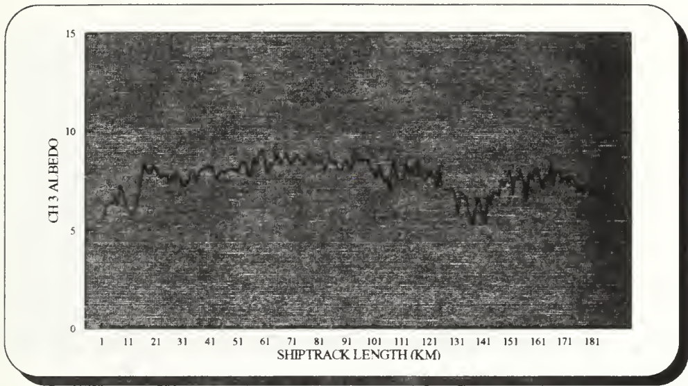
Fig 20. Shiptrack Algorithm Raw Data Plot: represents Arctic Shiptrack Case 1 Channel 3 Albedo; 1 indicates head of shiptrack
