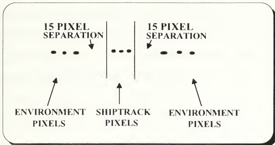
Fig. 1. Shiptrack Average Value Location: depicts the location of shiptrack and environment average pixel values
