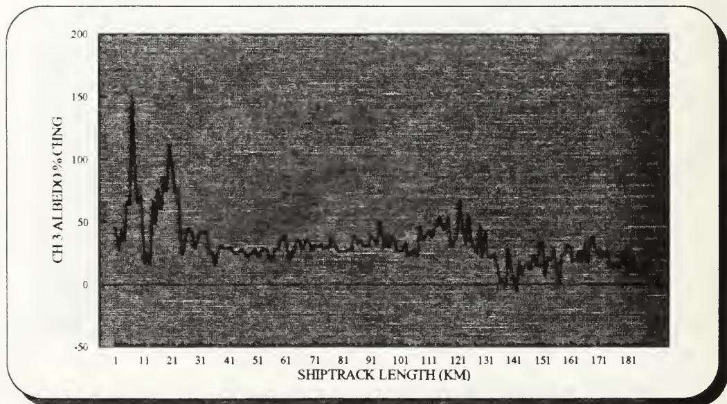
Fig 23. Shiptrack Algorithm Raw Data Plot: represents Arctic Shiptrack Case 1 Channel 3 Albedo Percent Change; 1 indicates head of shiptrack
