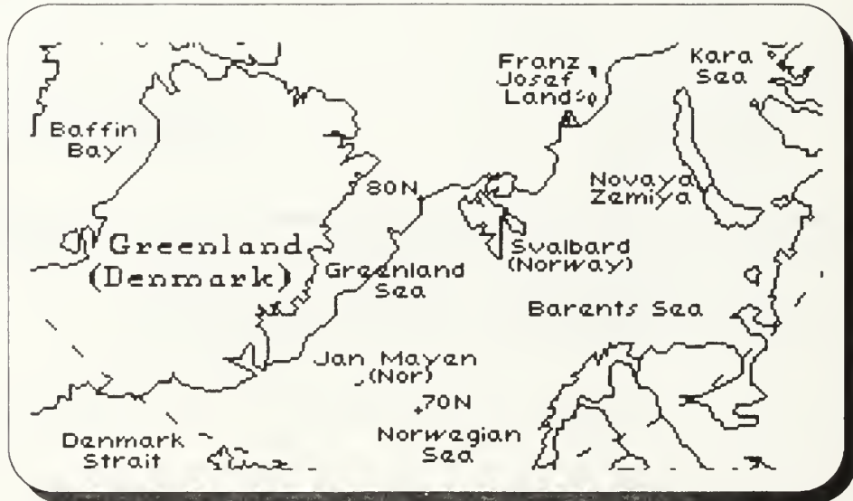
Fig. 3. Arctic Shiptrack Regional Location: dashed line indicates Arctic Circle; line east of Greenland is ice zone
