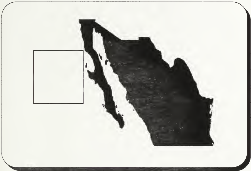
Fig. 13. Subtropic Shiptrack Region: box represents shiptrack analysis area
