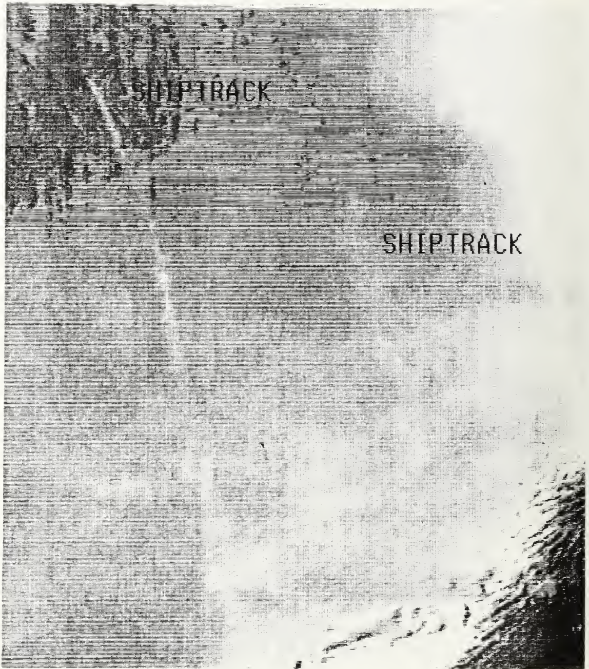
Fig. 14. Subtropic Shiptrack Cases 1 and 2: 13 July 1987 2314 UTC; Case 1 on left; Case 2 on right
