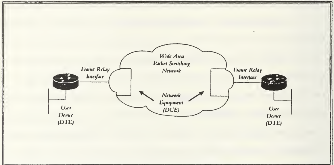
Figure 9. Router Interconnection Using Frame Relay
