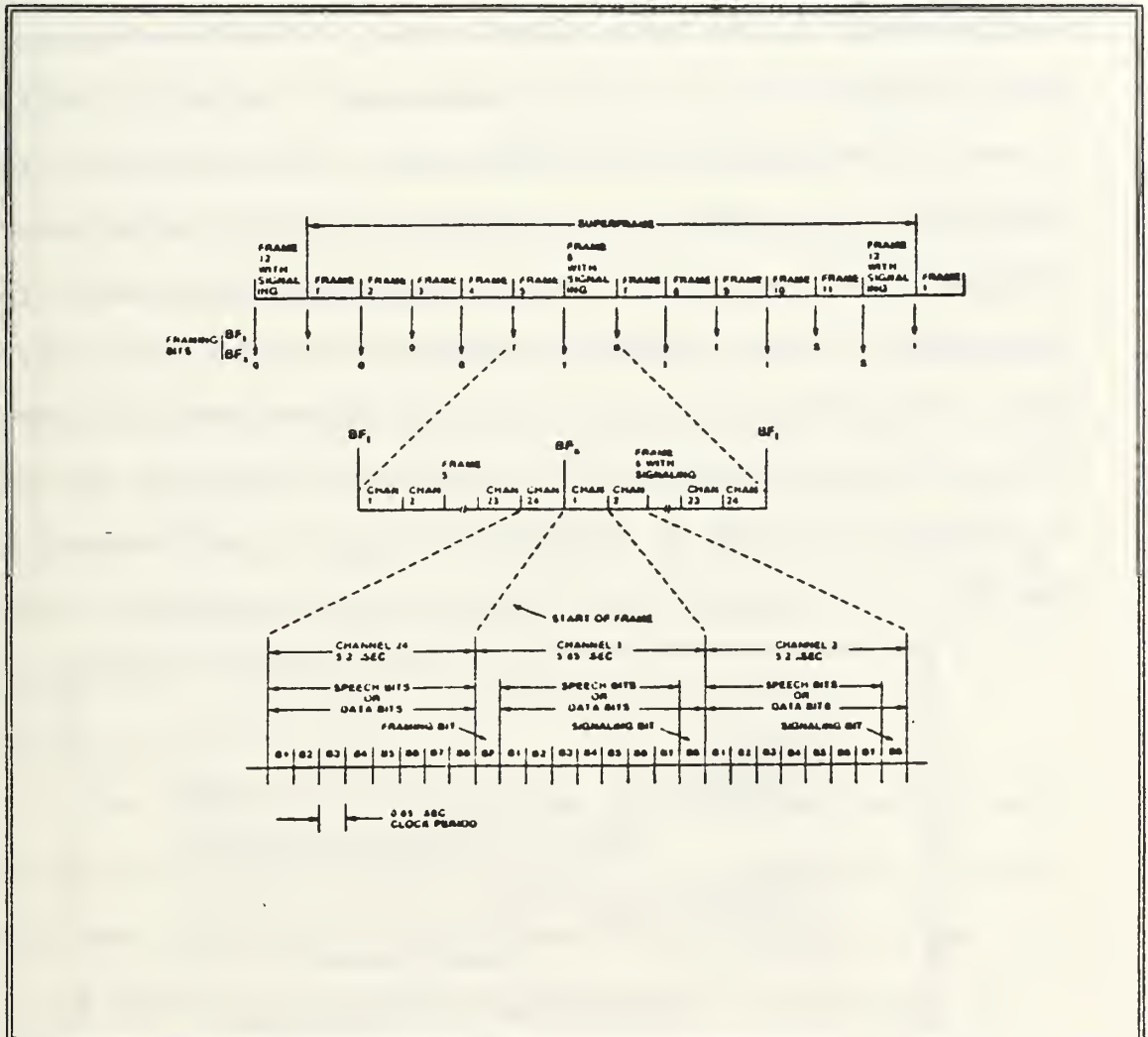
Figure 12. D4 Framing Pattern
