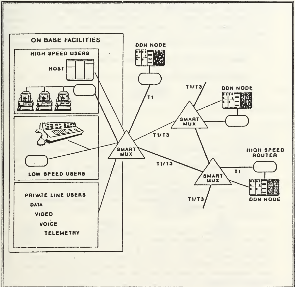
Figure 22. DISN Near-Term Nodal Configuration
