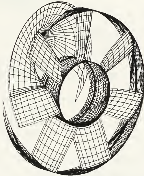
Figure 7-3: The original radial fan with cut-away duct. The trailing wake vortex system is shown emanating only from one blade to maintain clarity.
