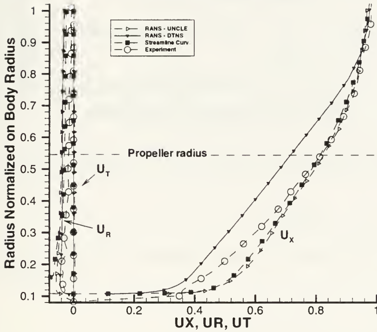
Comparison of Body 1 Nominal Inflow at Propeller Plane RANS,MTFLOW, EXPERIMENT
