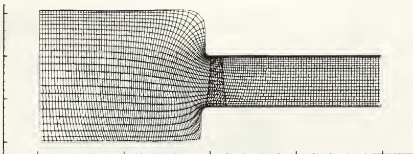
Figure 7-2: The flow grid used within MTFLOW. The long downstream extent is required by PBD to grow the trailing wake system. The upstream length of the domain is set by the requirement that the inviscid streamlines correctly match the constant inflow assumption.
