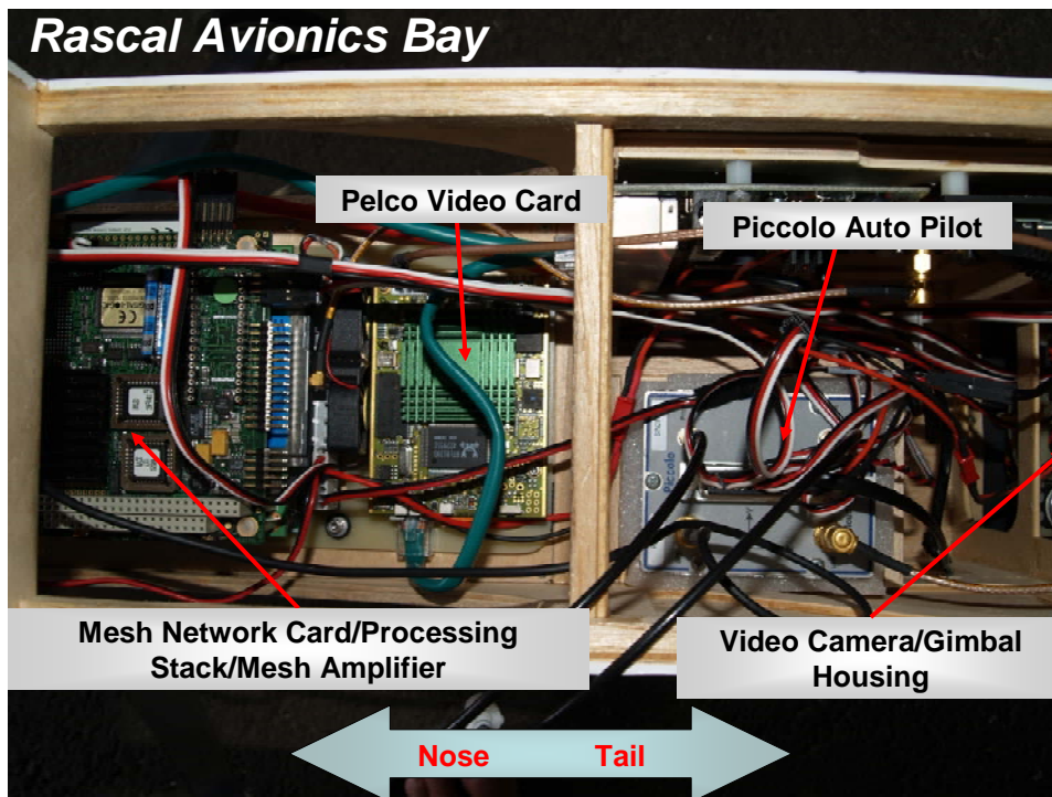
Figure 2. NPS UAS Avionics Bay
