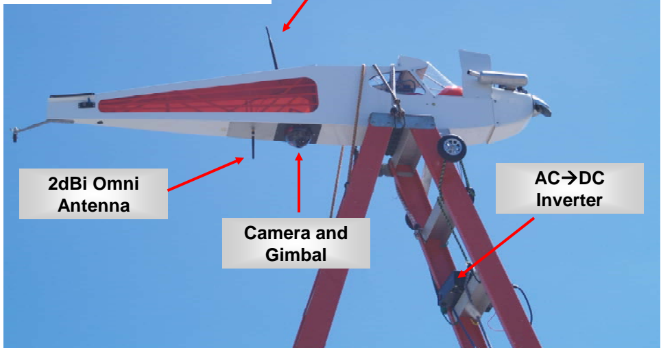
Figure 11. First Flight Test Set-Up—Rascal Set-Up
