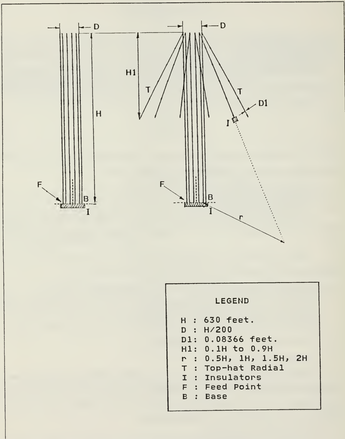
Figure 2. Monopole and Top-hat Antennas for NECGS computer models.
