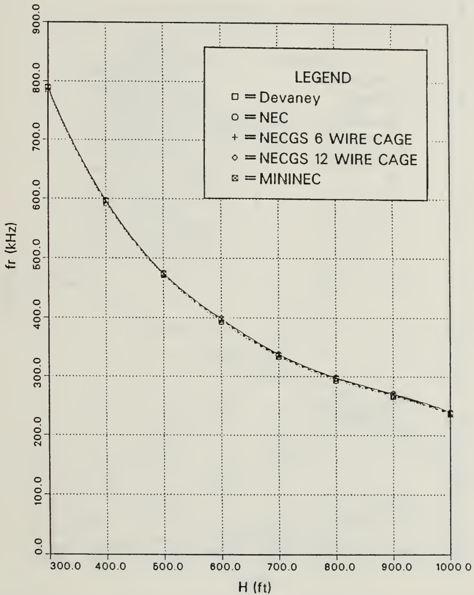
Figure 5. Variation of Resonant Frequency of Reference Monopole Antenna as a Function of Antenna Height.
