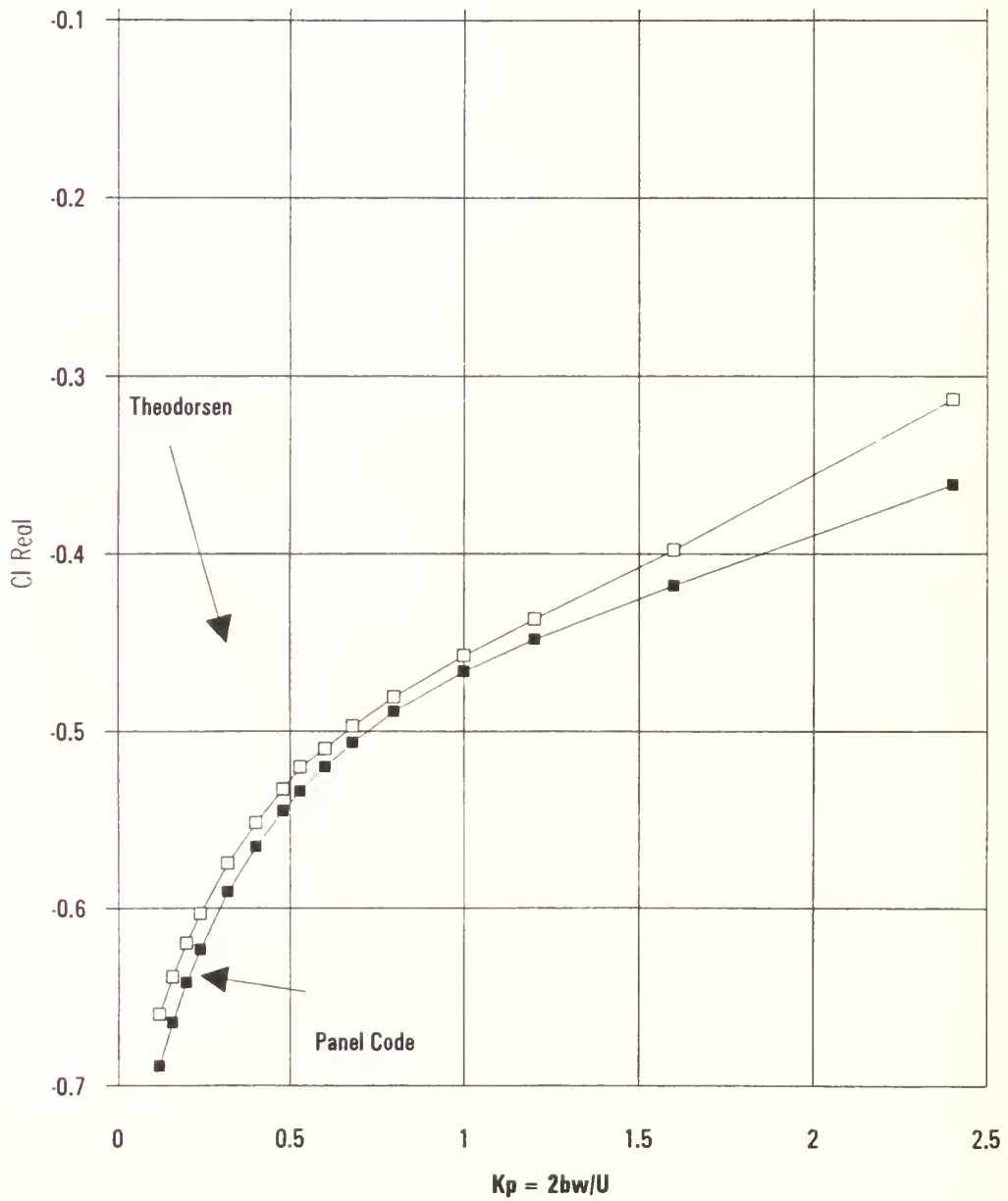
CI Real vs Kp Panel Code (Pitch, 6.7 deg, .37, NACA 0007, 75 panels top and bottom)
