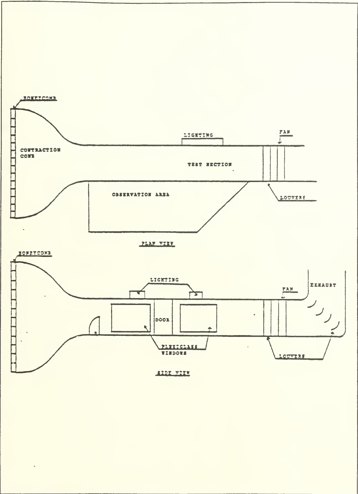
Figure 5.2 Tunnel Layout
