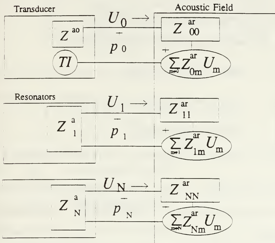
Figure 2-3 Network model of N interacting passive acoustic resonators and a transducer the previous two sections and allows for interactions between each element and every other element. The network equations are
