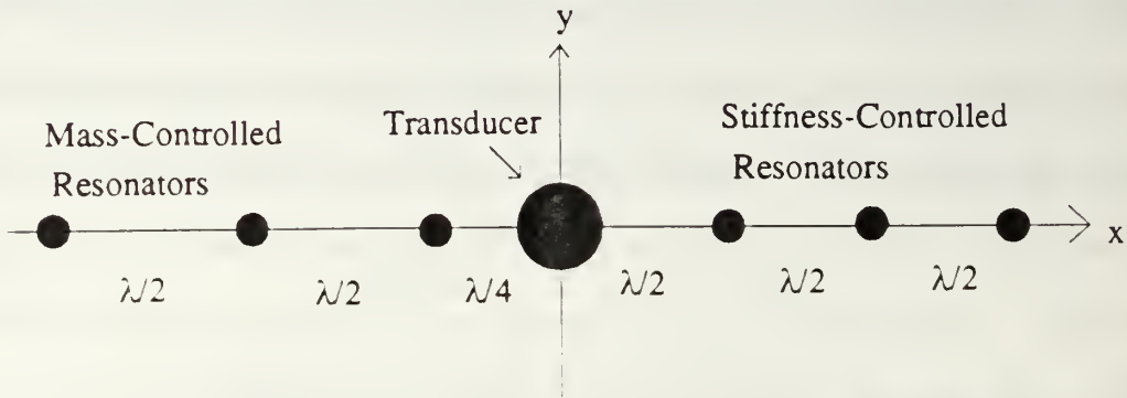
Figure 6-1 Diagram of the Yagi-Uda configuration (line type III) for six resonators.
