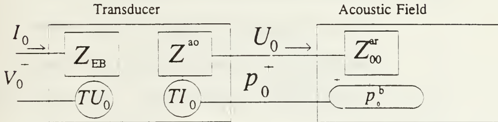
Figure 2-2 Lumped acoustic model of a transducer in an acoustic field.
