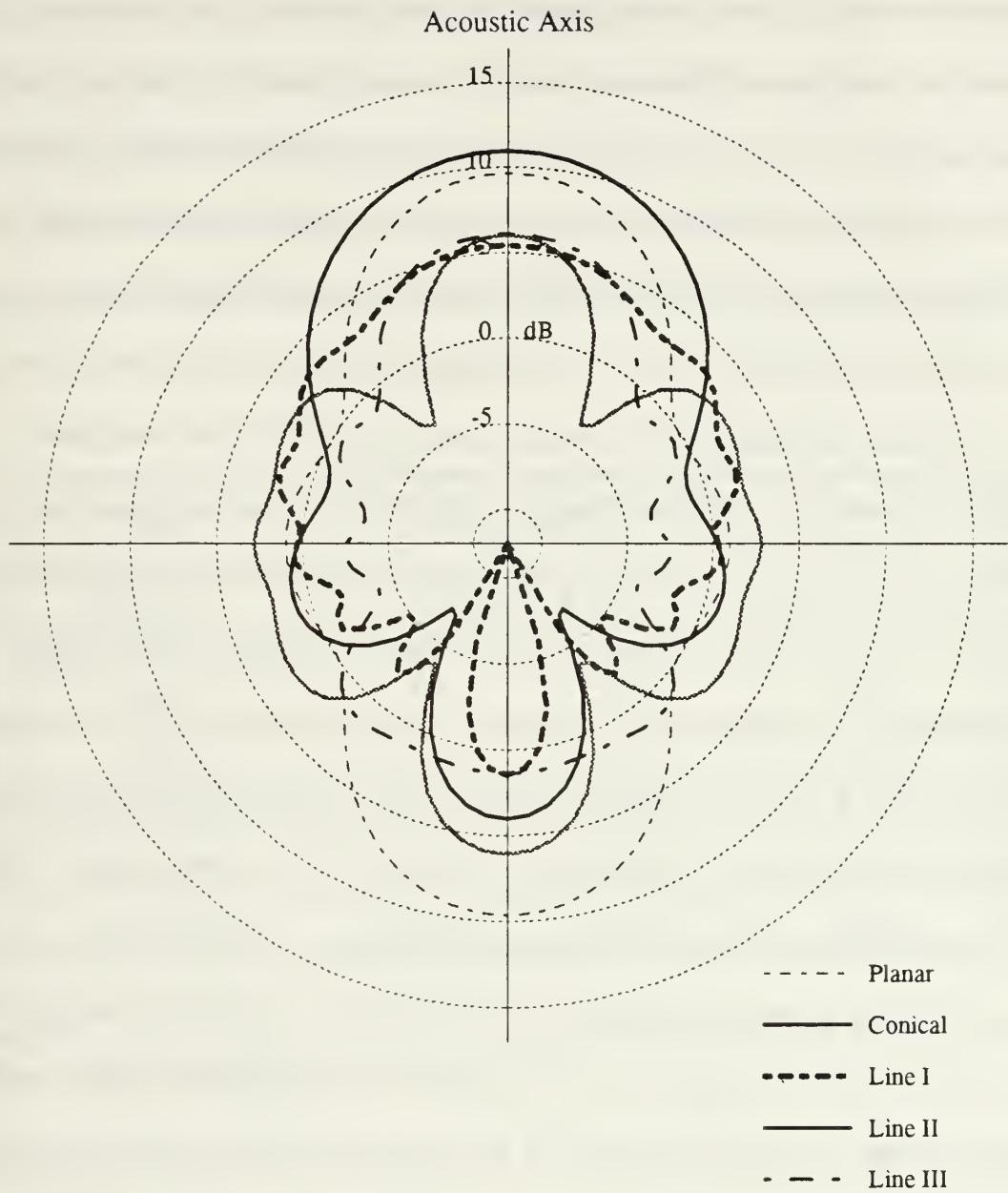
Figure 7-1 Polar plot of the far-field beam pattern for all configurations for six resonators.
