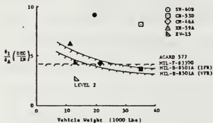
Hover roll response comparisons
