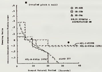
Hover longitudinal dynamic stability requirements
