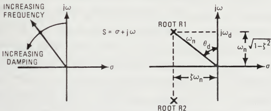
Figure 5-3 Effect of Root Location on Stability in the S Plane
