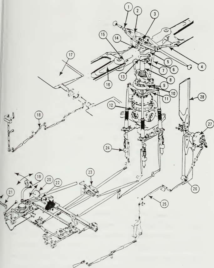
Figure 6-1 Mechanical Flight Control System From Reference 27
