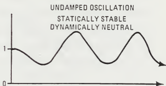
Figure 5-2 Illustration of Stability Options
