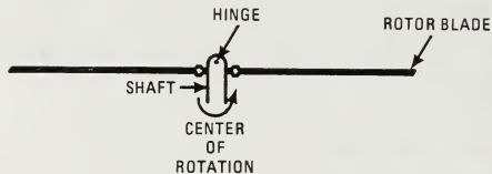
Figure 3-1 Sketch Showing Teetering Rotor Hub and Underslung Teetering Rotor System
