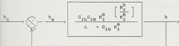
Figure 8-18 Simplified Block Diagram for Altitude Hold System
