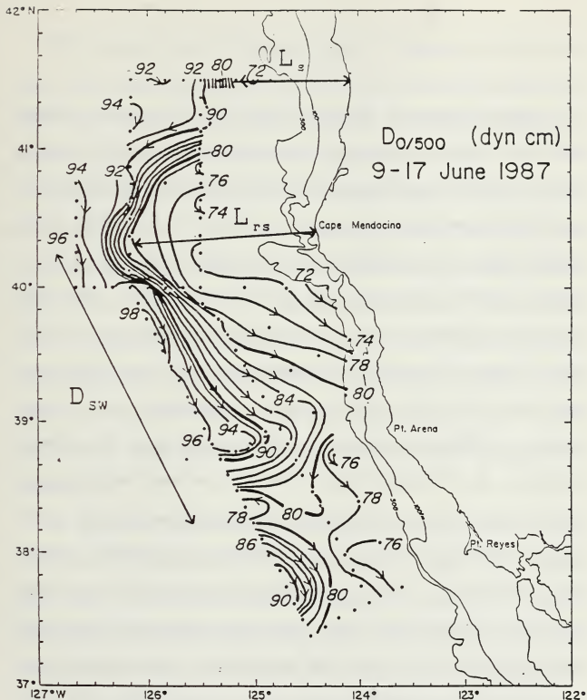
Figure 3.3 Map of dynamic height of the sea surface relative to 500 db for the June 1987 data. This shows the measurements for L_s , L_{rs} , and D_{sw} . [From "OSU Data Report for CTD Observations in the Coastal Transition Zone Off Northern California, 9-18 June 1987".]
