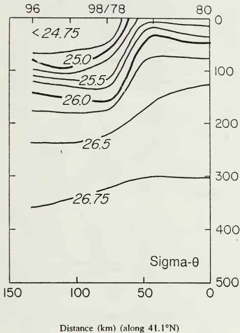
Figure 4.1 Cross section of sigma theta, May 87 (OSU) cruise, from which h_0 , and g' are measured to determine \theta . [From "OSU Data Report for CTD Observations in the Coastal Transition Zone Off Northern California, 24-26 May 1987".]
