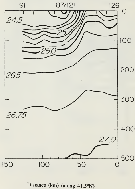
Figure 4.2 Cross section of sigma theta, June 87 (OSU) cruise, from which h_0 , and g' are measured to determine \theta . [From "OSU Data Report for CTD Observations in the Coastal Transition Zone Off Northern California, 9-18 June 1987".]
