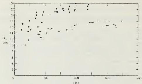
Figure A.1 Scatter plot showing how L_r , the distance of the head of the plume from the tank wall varies with time. (The solid dots represent \theta = 2.03 and the '+'s represent \theta = 36.43 ) [From Narimousa and Maxworthy (1985).]
