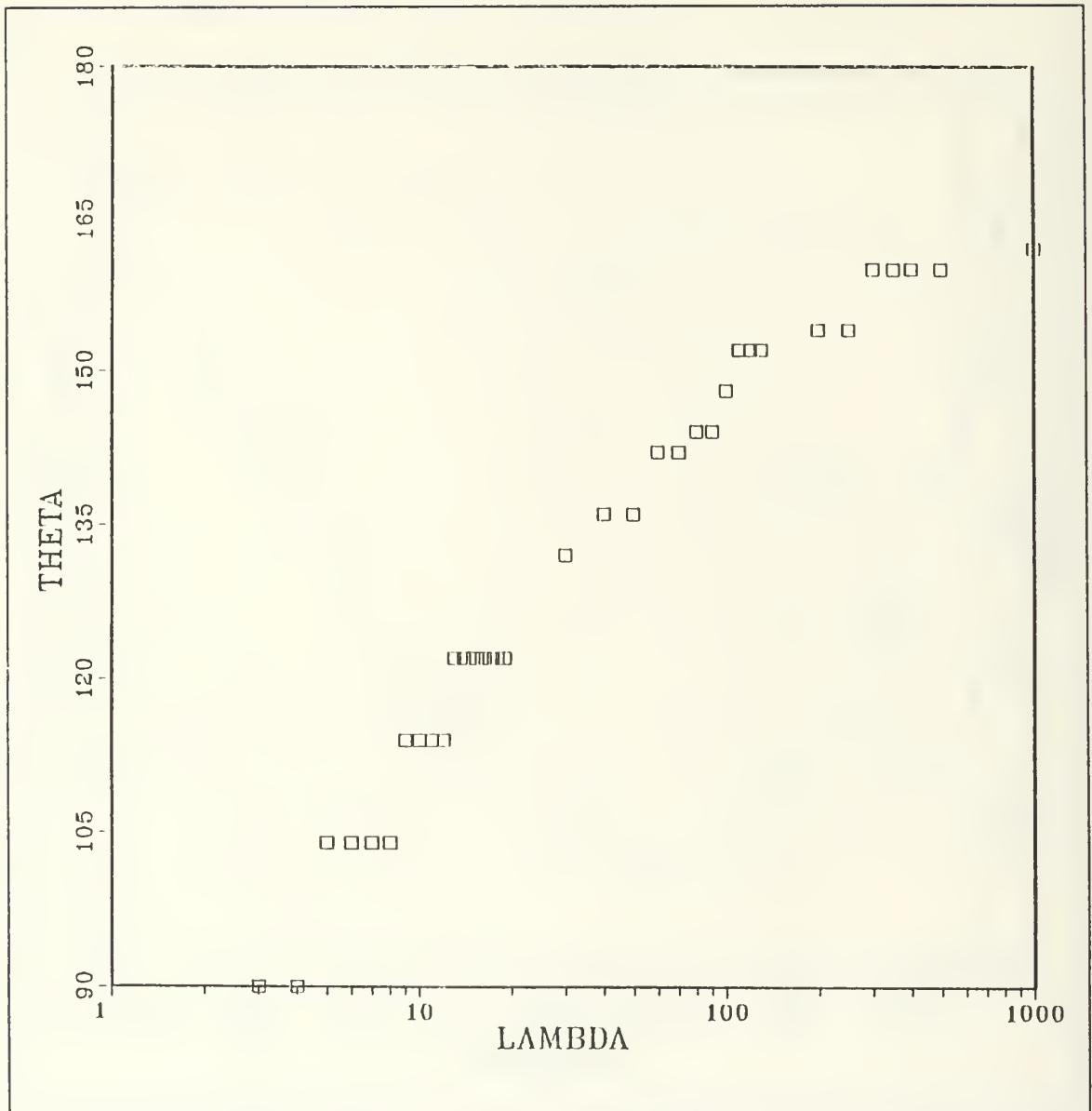
Figure 18. Semilog Plot Relating the Deadzone Angle to the Fuel/Time Tradeoff Parameter
