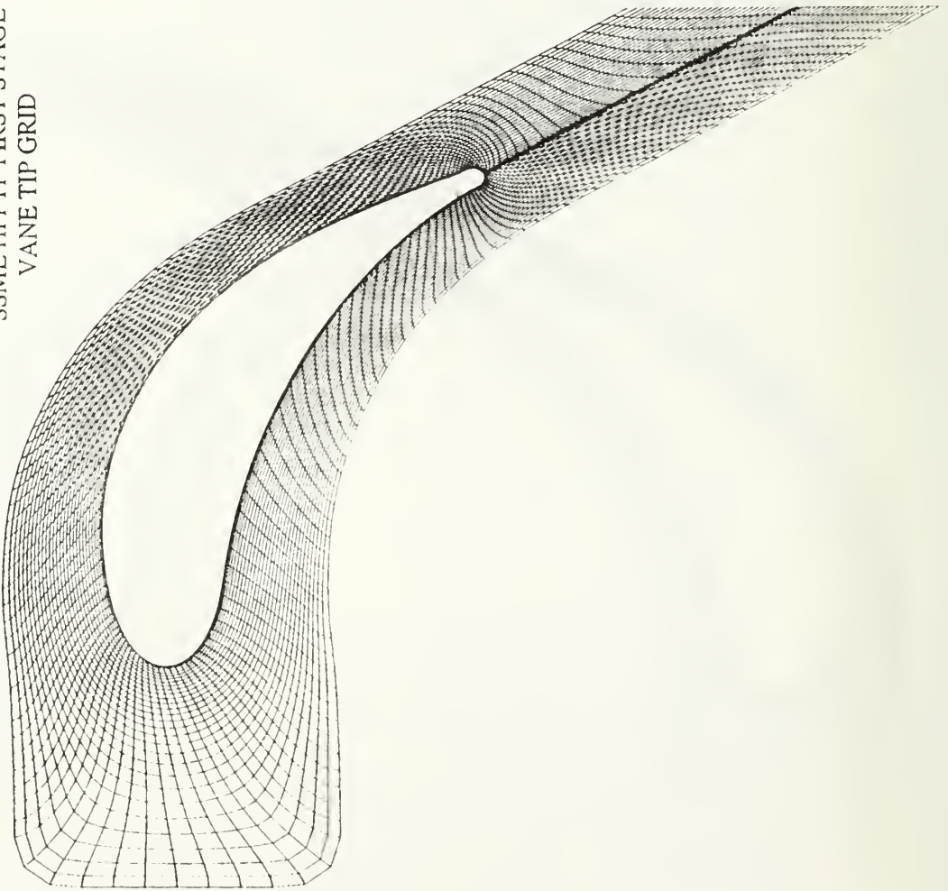
Figure 11. C-Grid at Stator Tip
