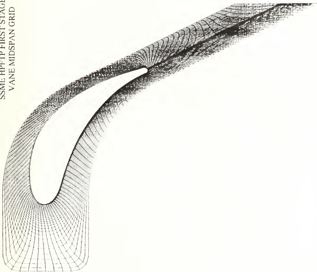
Figure 10. C-Grid at Stator Midspan
