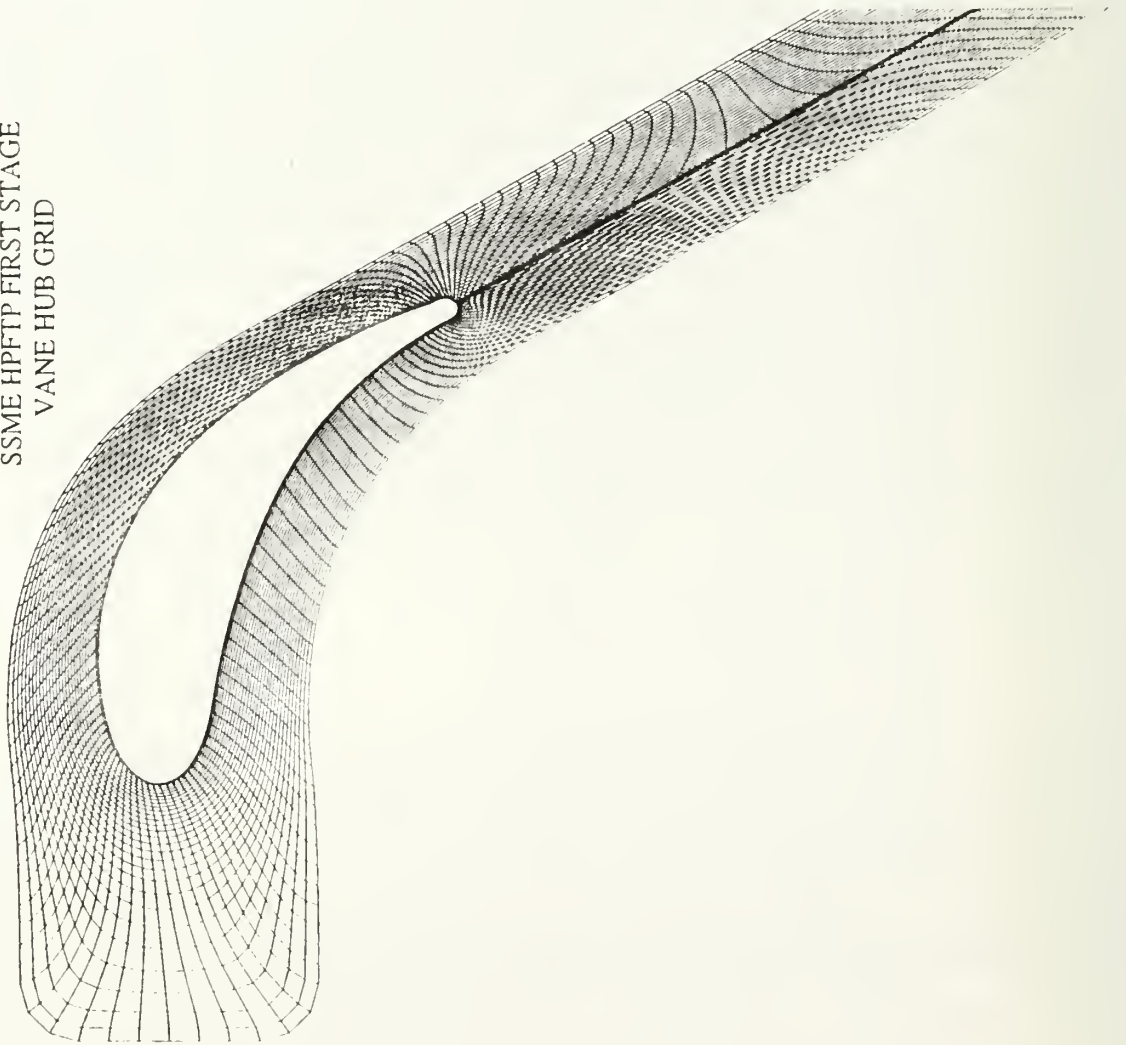
Figure 9. C-Grid at Stator Hub
