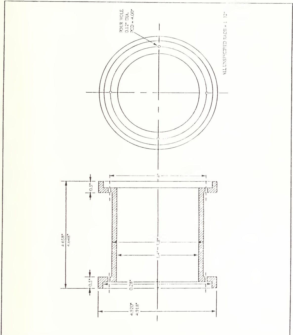
Figure A1. Bearing Outer Spacer
