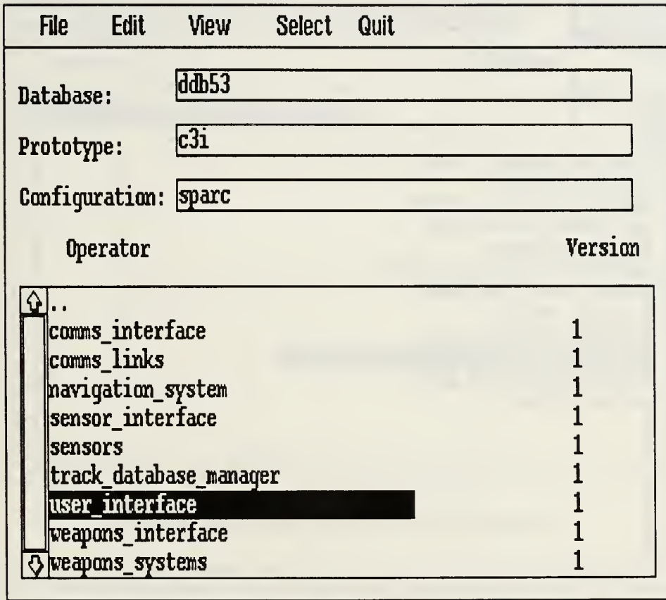
Figure 3. DDB User Interface (Search for Component)
