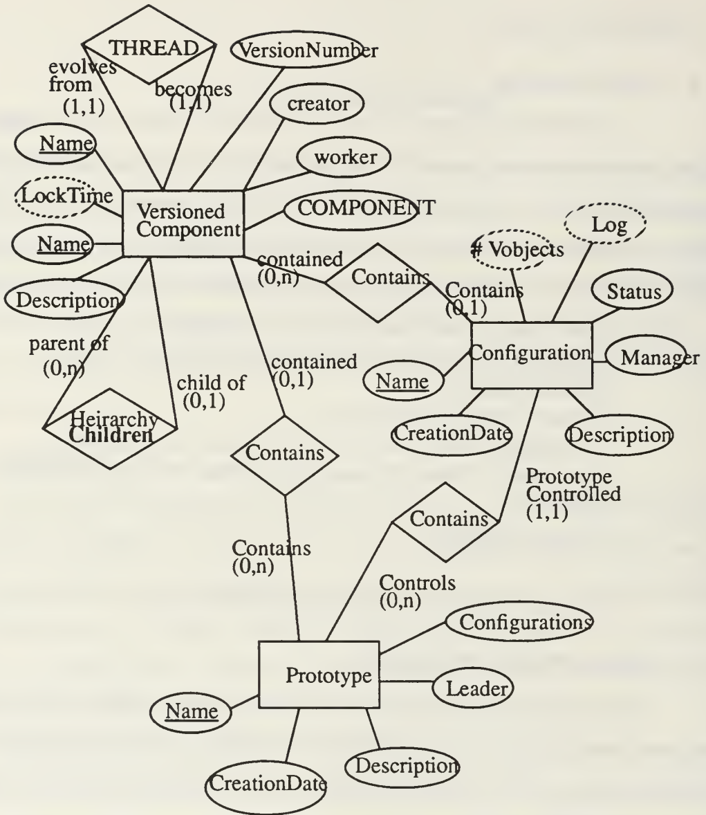
Figure 12. Design Database Entity Relationship Diagram
