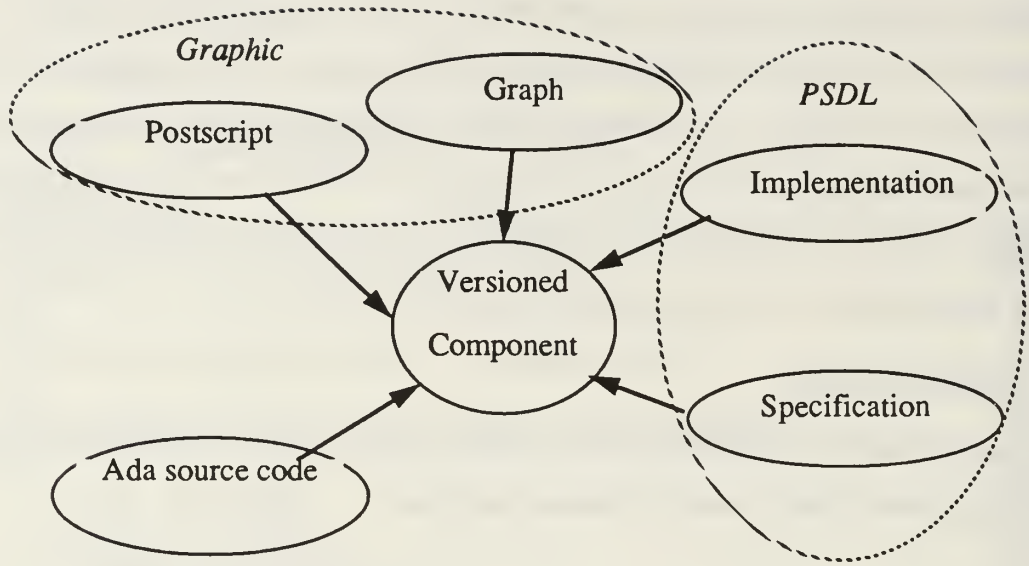
Figure 8. CAPS Files in Versioned Component
