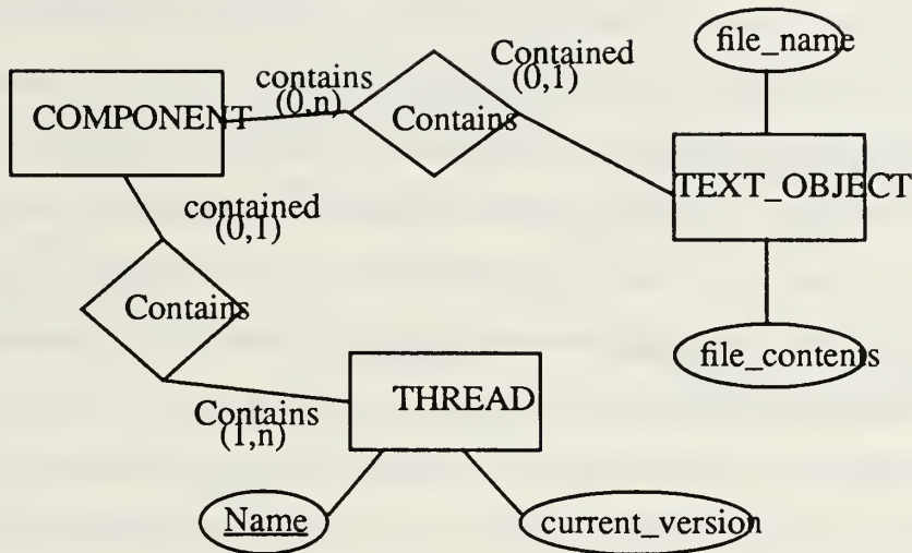
Figure 13. Design Database Entity Relationship Diagram
