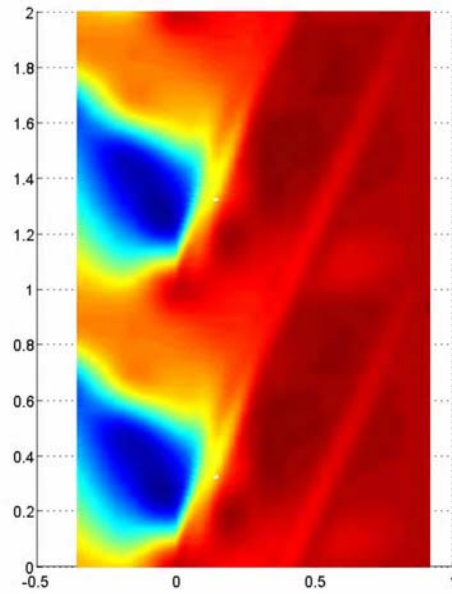
Figure 24. Pressure Contours 90% speed and a Pressure Ratio of 1.47
