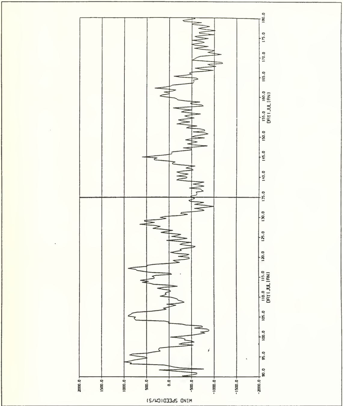
Figure 26. Expanded time series of meridional wind velocity (cm/s) for days 90-180 (31 Mar.-29 Jun.) 1987.
