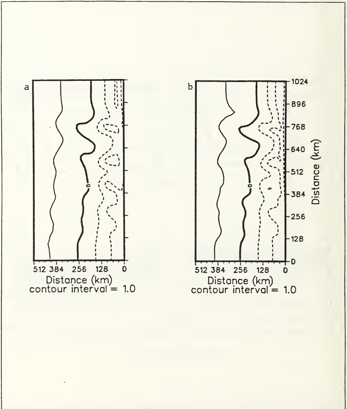
Figure 25. Surface isopleths of dynamic height (cm) relative to 2400 m for a) 2 Jan (day 2) and b) 22 Jan. (day 22) 1988. Dashed lines are negative contours.
