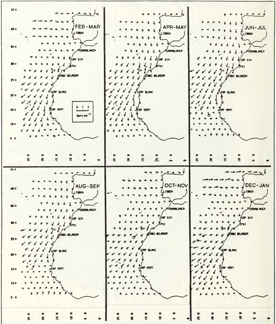
Figure 4. Seasonal variation of wind stress (dyne cm -2 ) over the northern reaches of the Canary Current (Bakun and Nelson, 1991)
