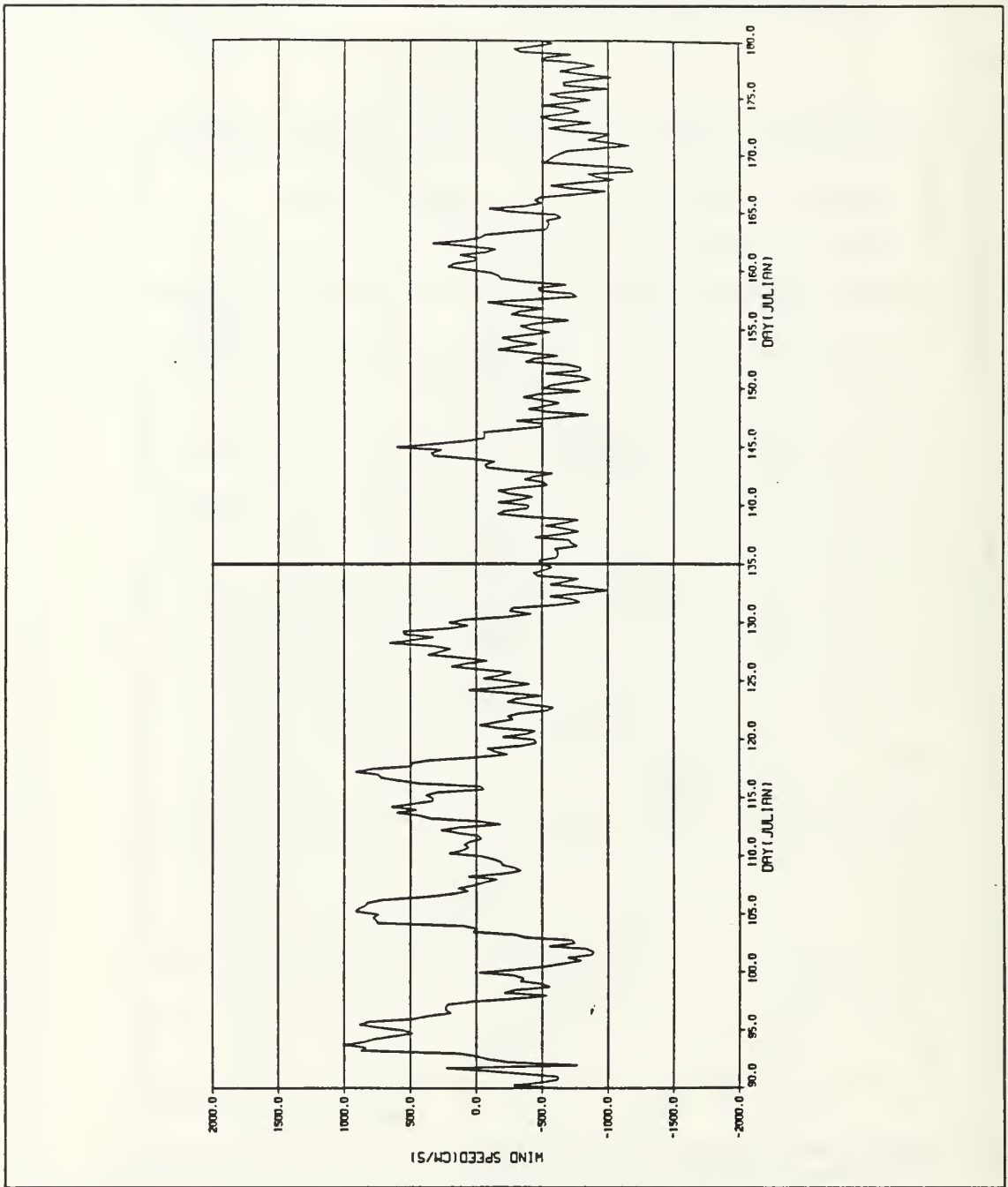
Figure 13. Expanded time series of meridional wind velocity (cm/s) for days 90-180 (31 Mar.-29 Jun.) 1987 at 39°N, 10°W.
