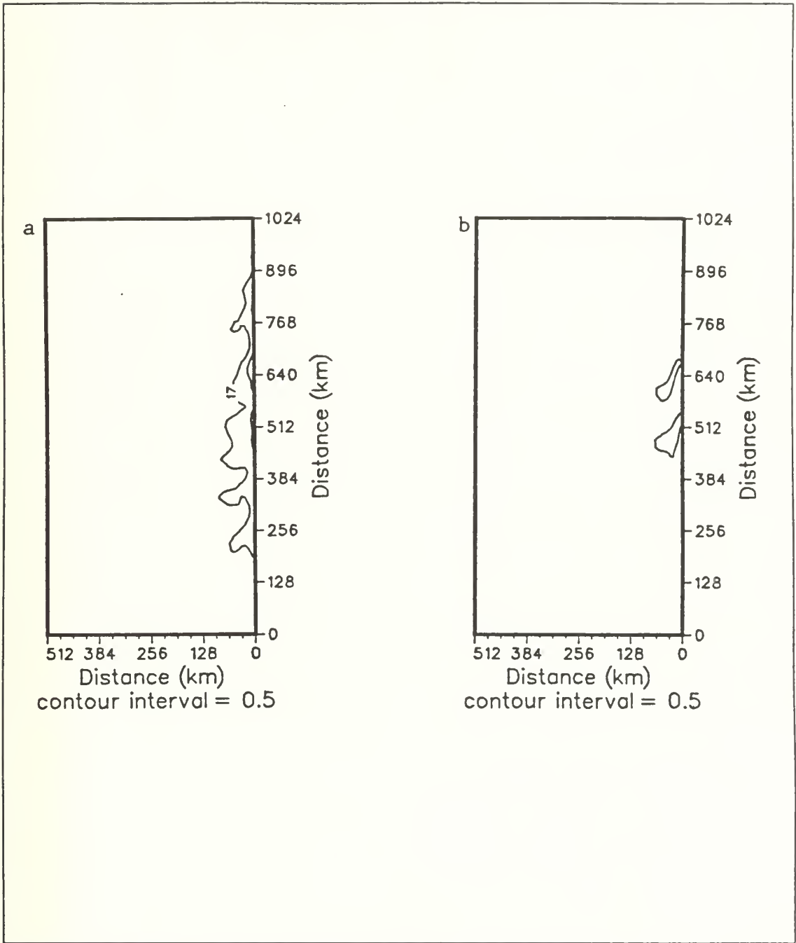
Figure 38. Surface isotherms ( ^{\circ}\text{C} ) for a) 26 Aug. (day 238) and b) 4 Oct. (day 277) 1987 (17 ^{\circ}\text{C} isotherm shown in b).
