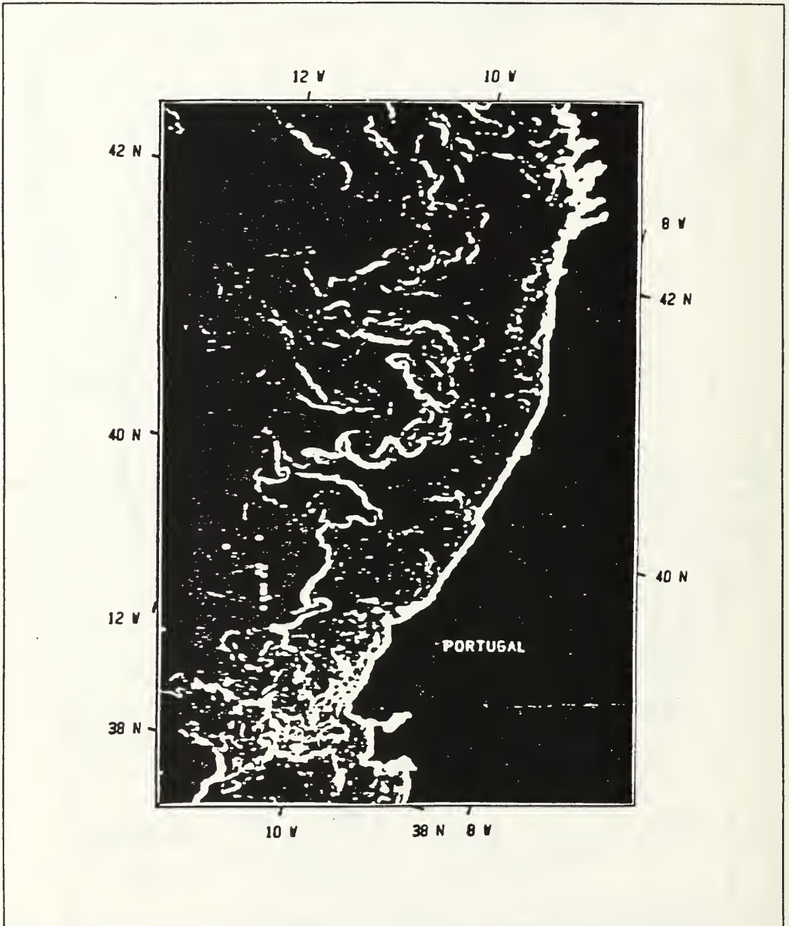
Figure 6. Sea surface temperature gradient patterns showing filament structure off Portugal in Sept. 1982 (Barton, 1986).
