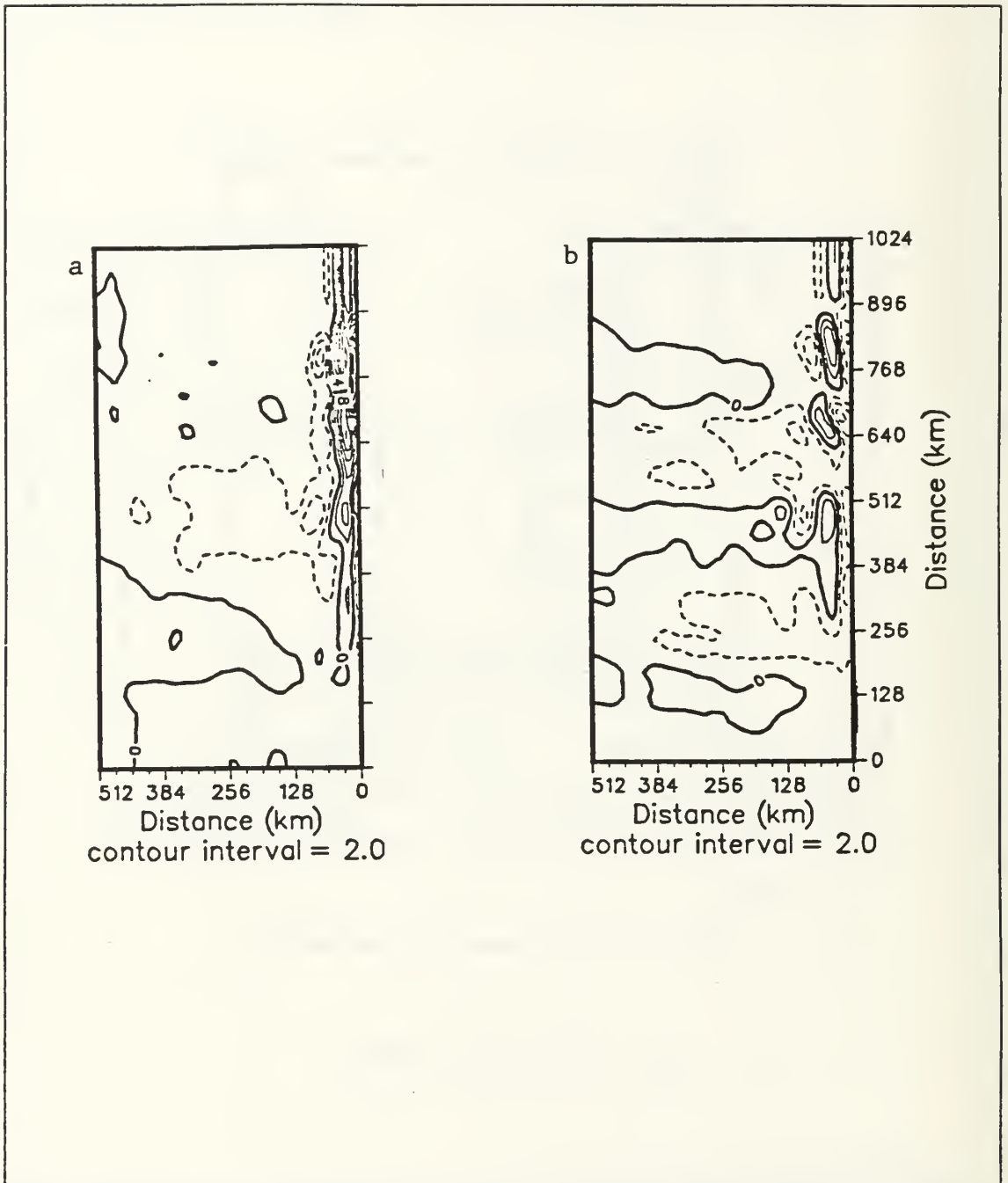
Figure 47. Isopleths of meridional velocity (cm/s) at 75 m depth for a) 12 Nov. and b) 7 Dec. 1988. Dashed lines are negative contours.
