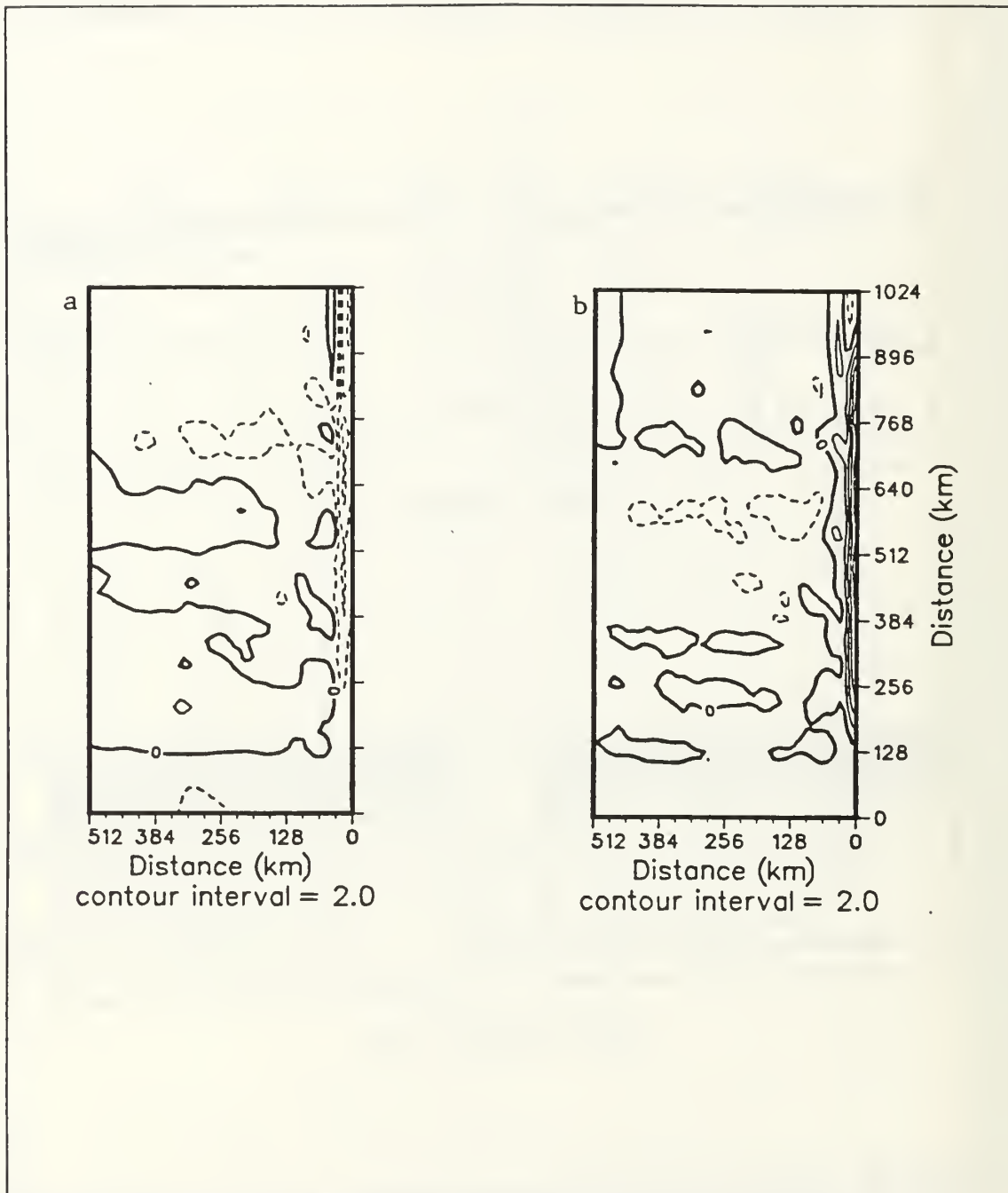
Figure 23. Isopleths of meridional velocity (cm/s) at 75 m depth for a) 23 Jan. (day 23) and b) 27 Jan. (day 27) 1988. Dashed lines are negative contours.
