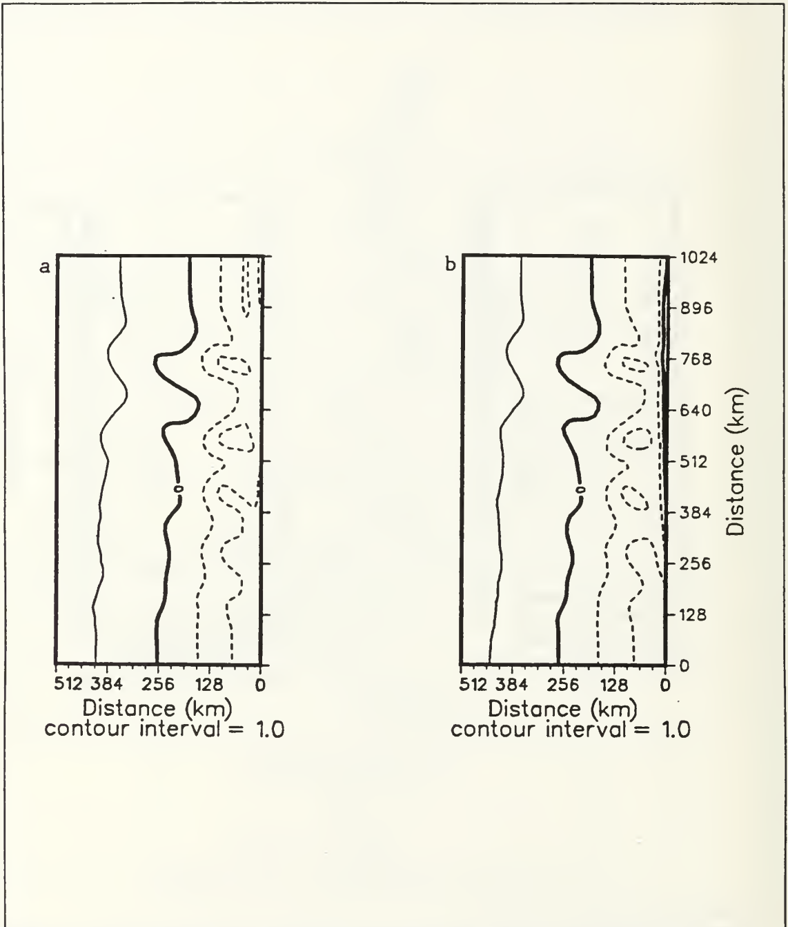
Figure 21. Surface isopleths of dynamic height (cm) relative to 2400 m for a) 4 Jan. (day 4) and b) 6 Jan. (day 6) 1988. Dashed lines are negative contours.
