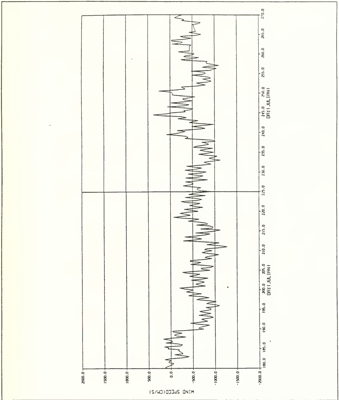
Figure 32. Expanded time series of meridional wind velocity (cm/s) for days 180-270 (28 Jun.-26 Sep.) 1988.
