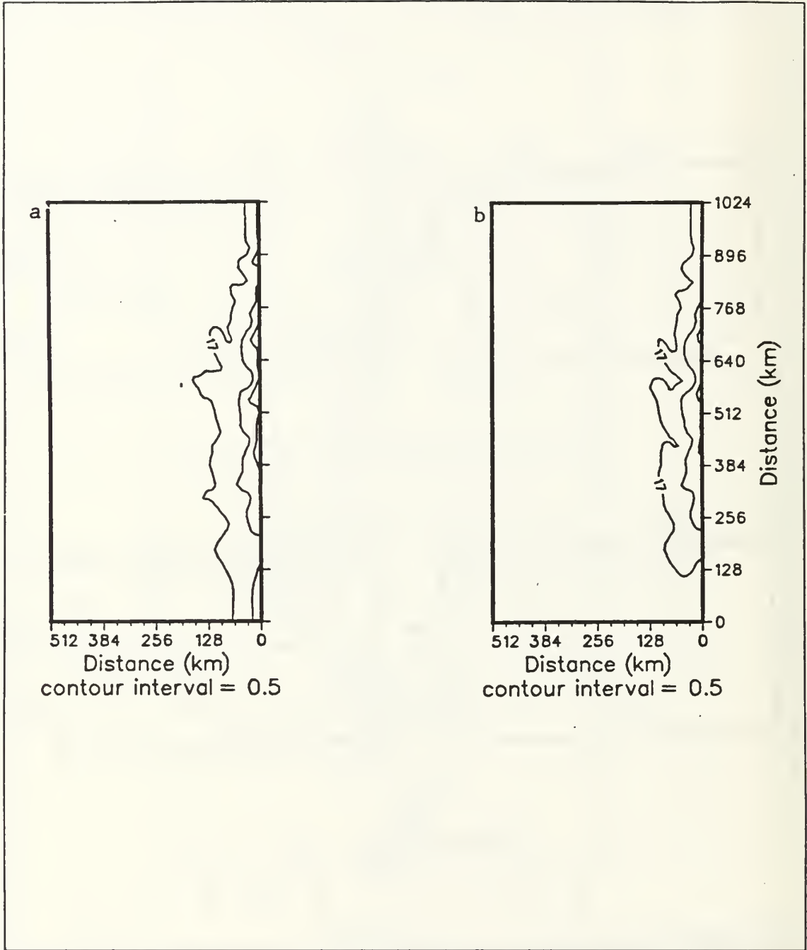
Figure 43. Surface isotherms ( ^{\circ}\text{C} ) for a) 1 Sep. and b) 29 Sep. 1988.
