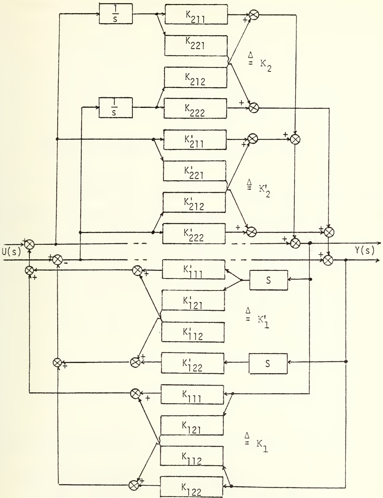
Figure 7. Simulation diagram for fourth order system with m = 2 for Caer matrix mixed form.
