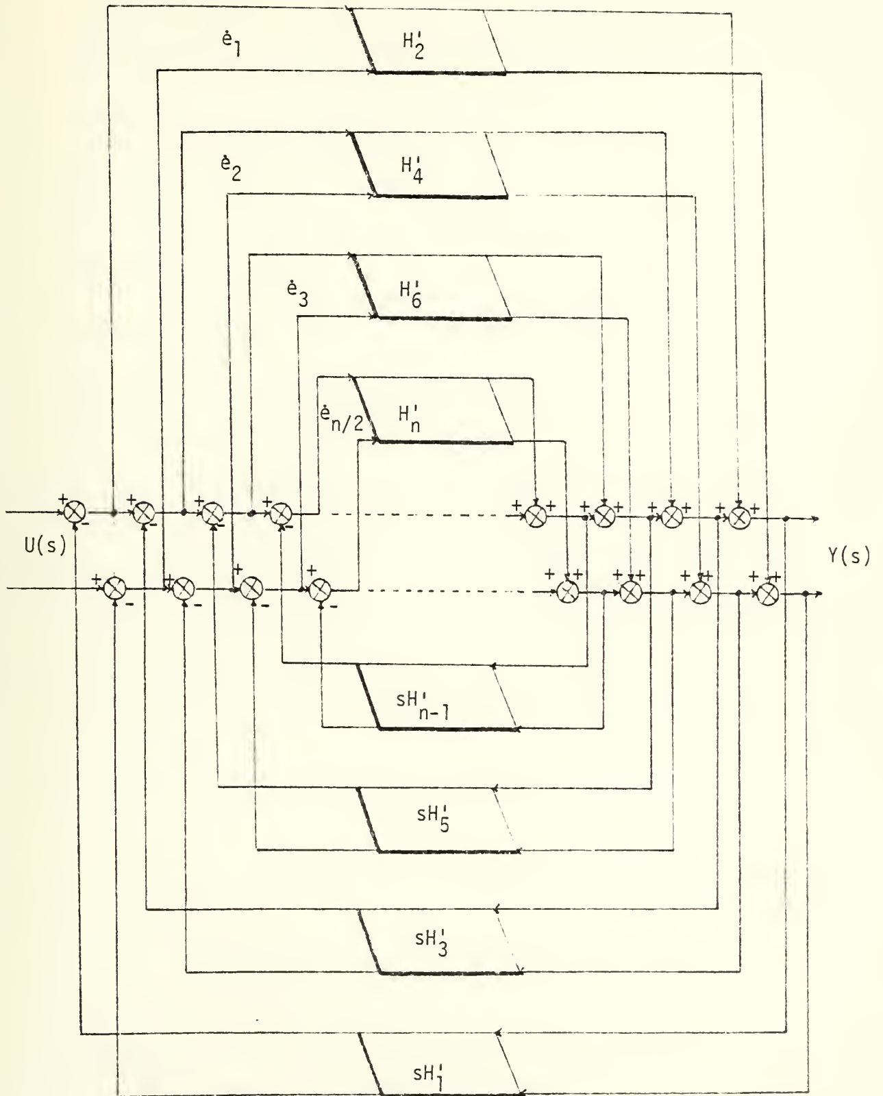
Figure 3. Matrix representation of a n th/2 order system by Causer first form with two inputs two outputs. ( n even)
