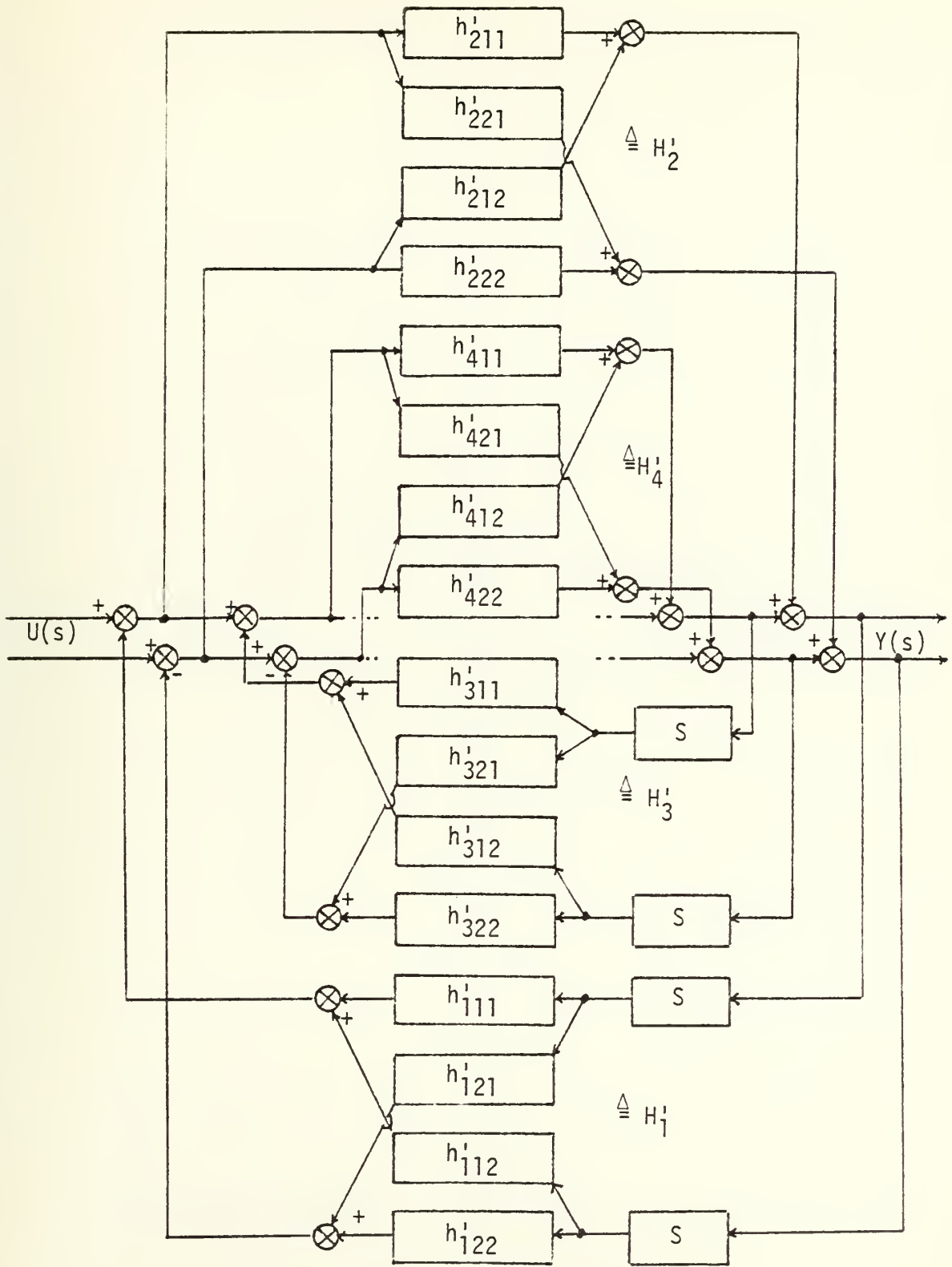
Figure 8. Simulation diagram for fourth order system with m = 2 for Cauchy matrix first form.
