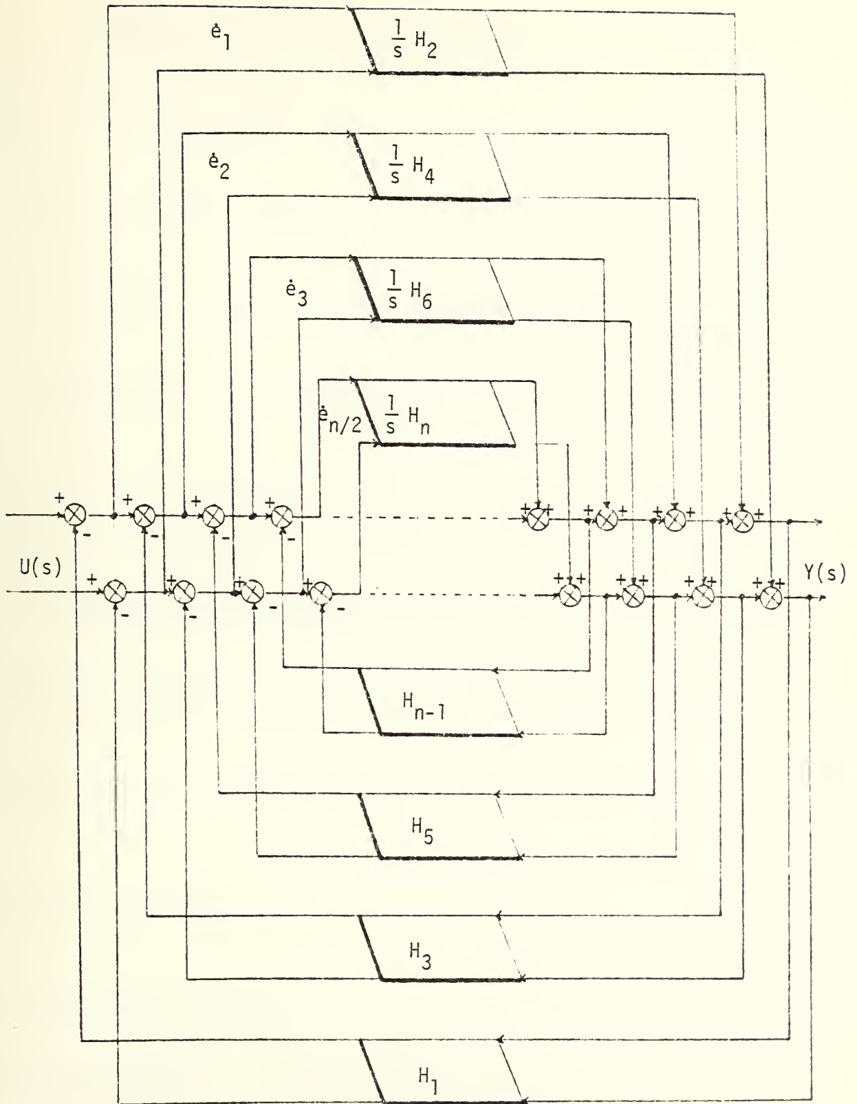
Figure 4. Matrix representation of a n/2 order system by Causer second form with two inputs two outputs. ( n even)
