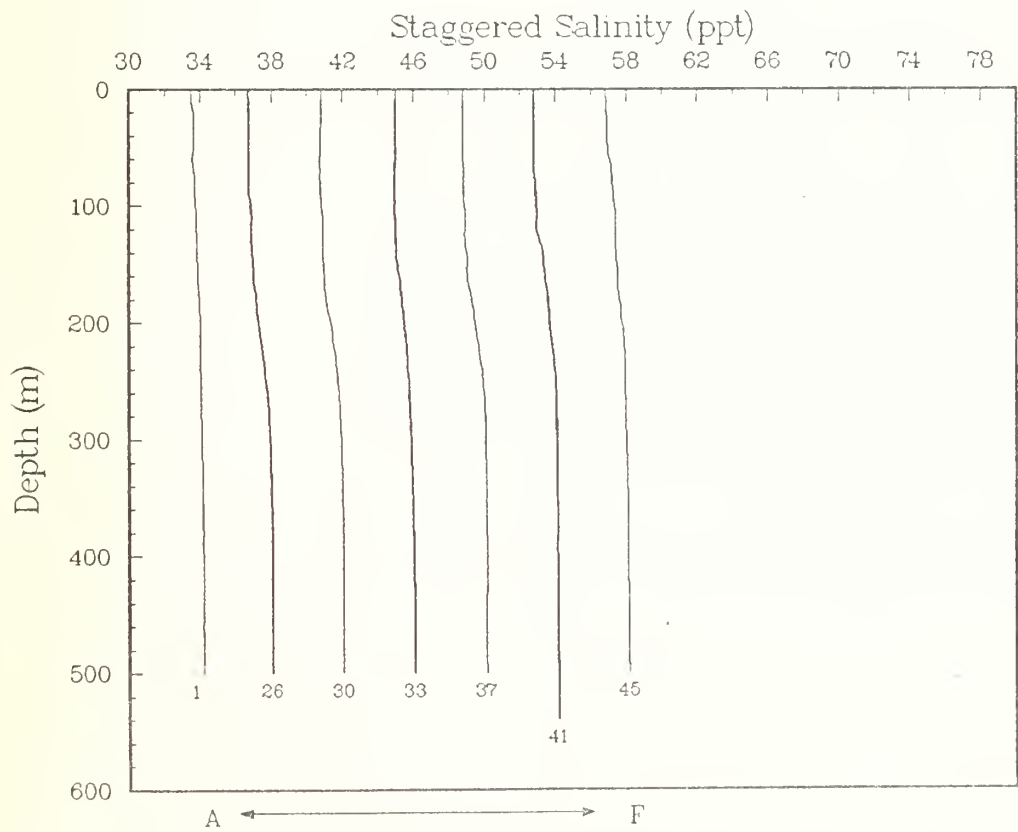
Figure 33(a): CTD temperature profiles, staggered by multiple of 2 deg C, and salinity profiles, staggered by multiples of 4 ppt. 10/1/02, Leg 211.
