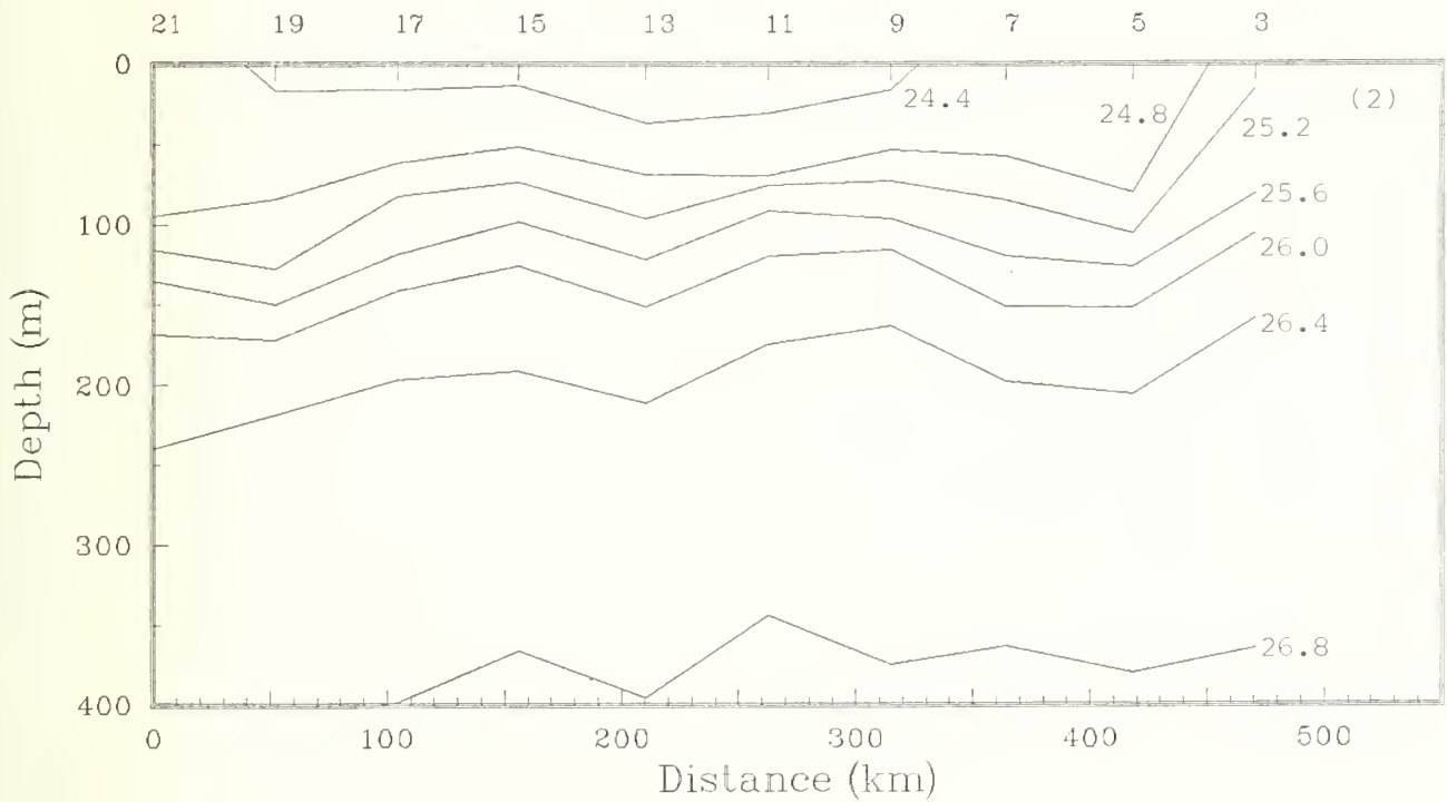
Figure 8(a): Isopleths of (1) temperature and salinity and (2) \sigma\text{-t} from the CTD's. (OPTOMA5, Leg D).
