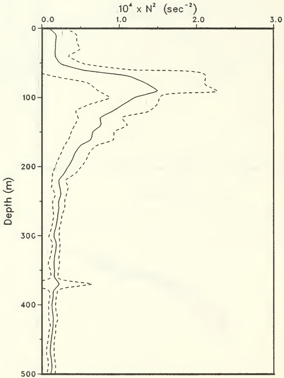
Figure 33: Mean N^2 profile (—), with + and - the standard deviation (---). The N^2 profile from \overline{T(z)} and \overline{S(z)} is also shown (....) (OPTOMA15, Leg DII).
