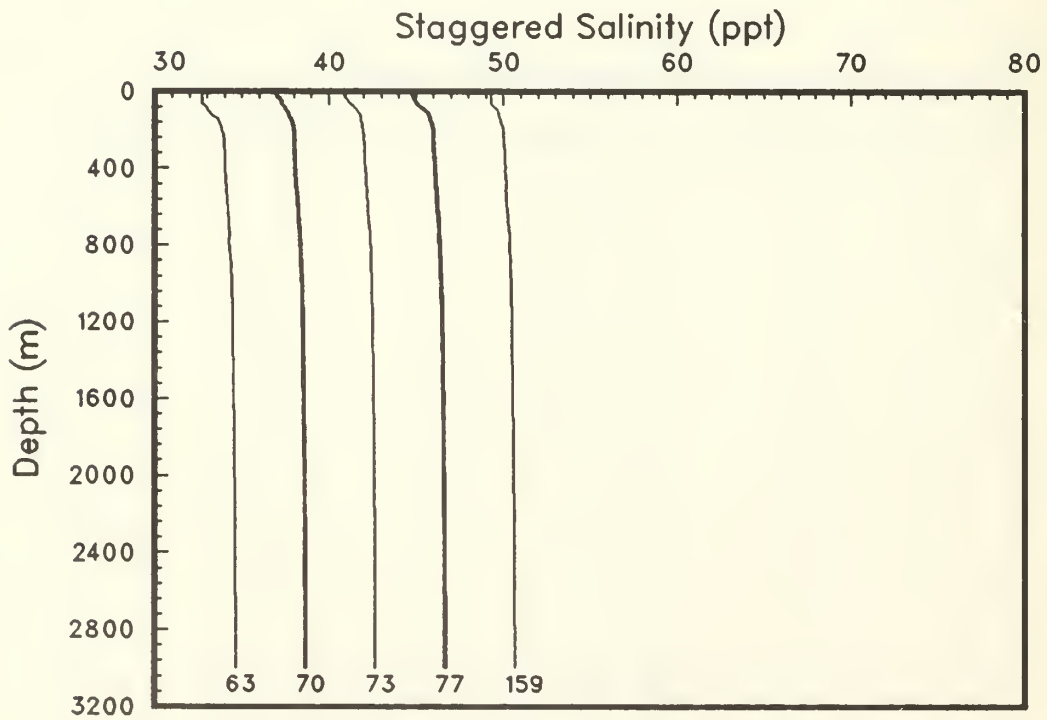
Figure 8: Casts deeper than 1600m (OPTOMA15, Leg DI).
