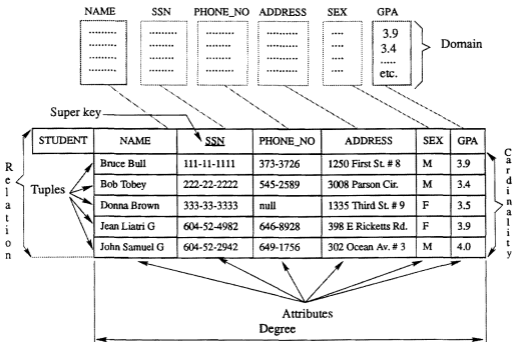
Figure 2.1: A Relation STUDENT Schema
