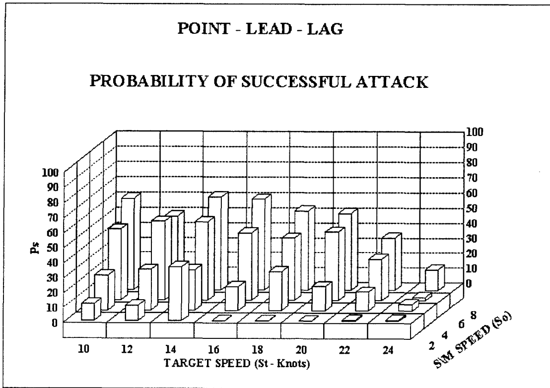
Figure 15. P_s vs S_t and S_o (P-LEAD-LAG)-(Bar Plot)
