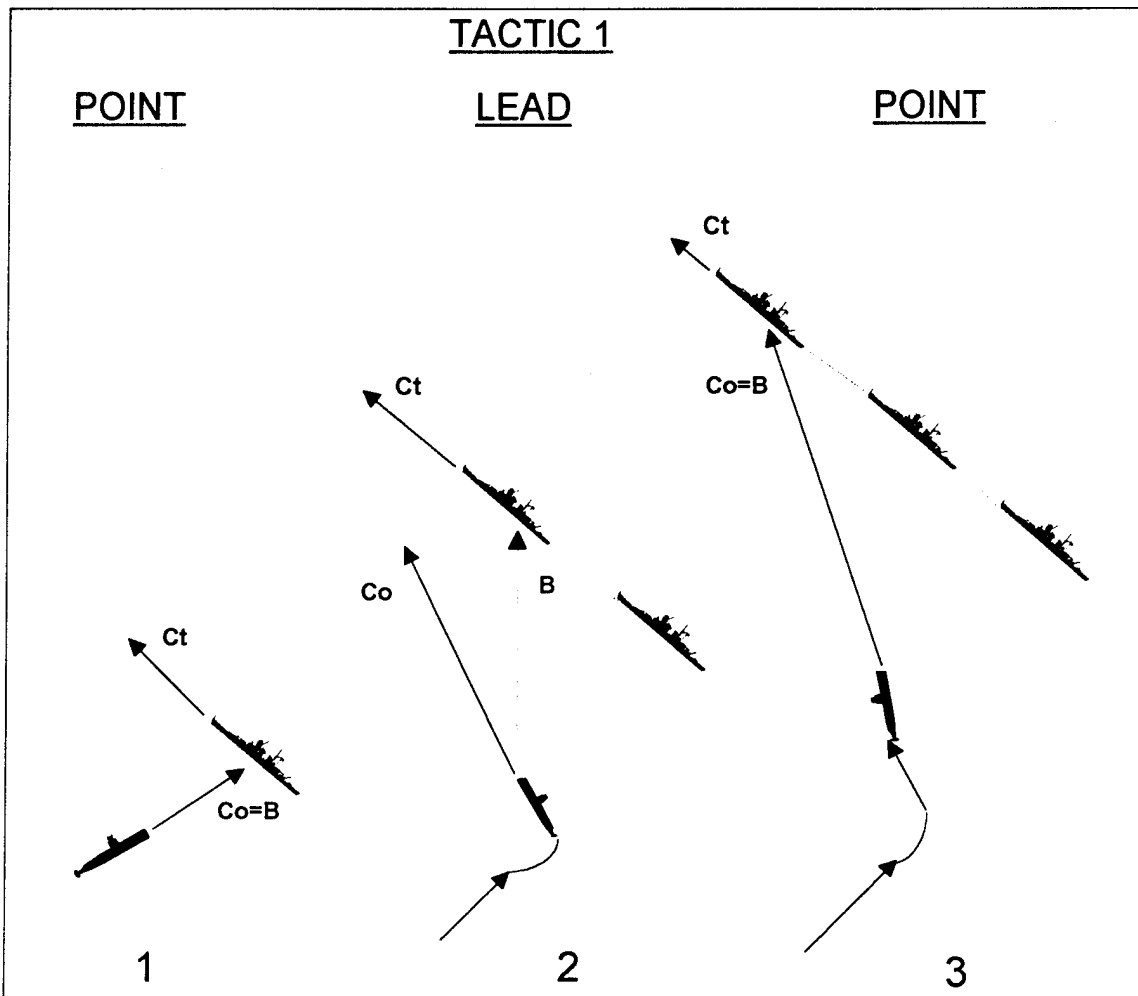
Figure 8. Geoplot (P-LEAD-P)
