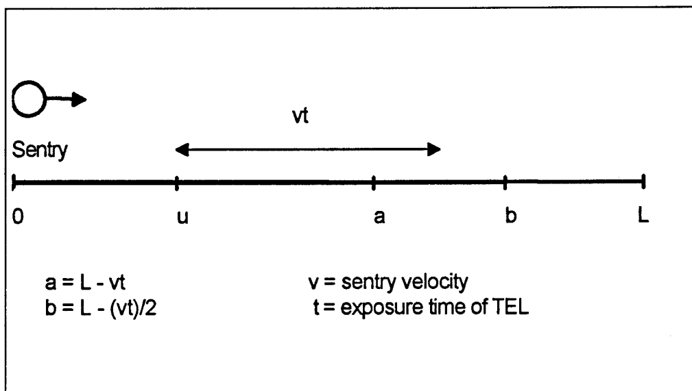
Figure 5: Schematic of the Road for the Sentry Search model
