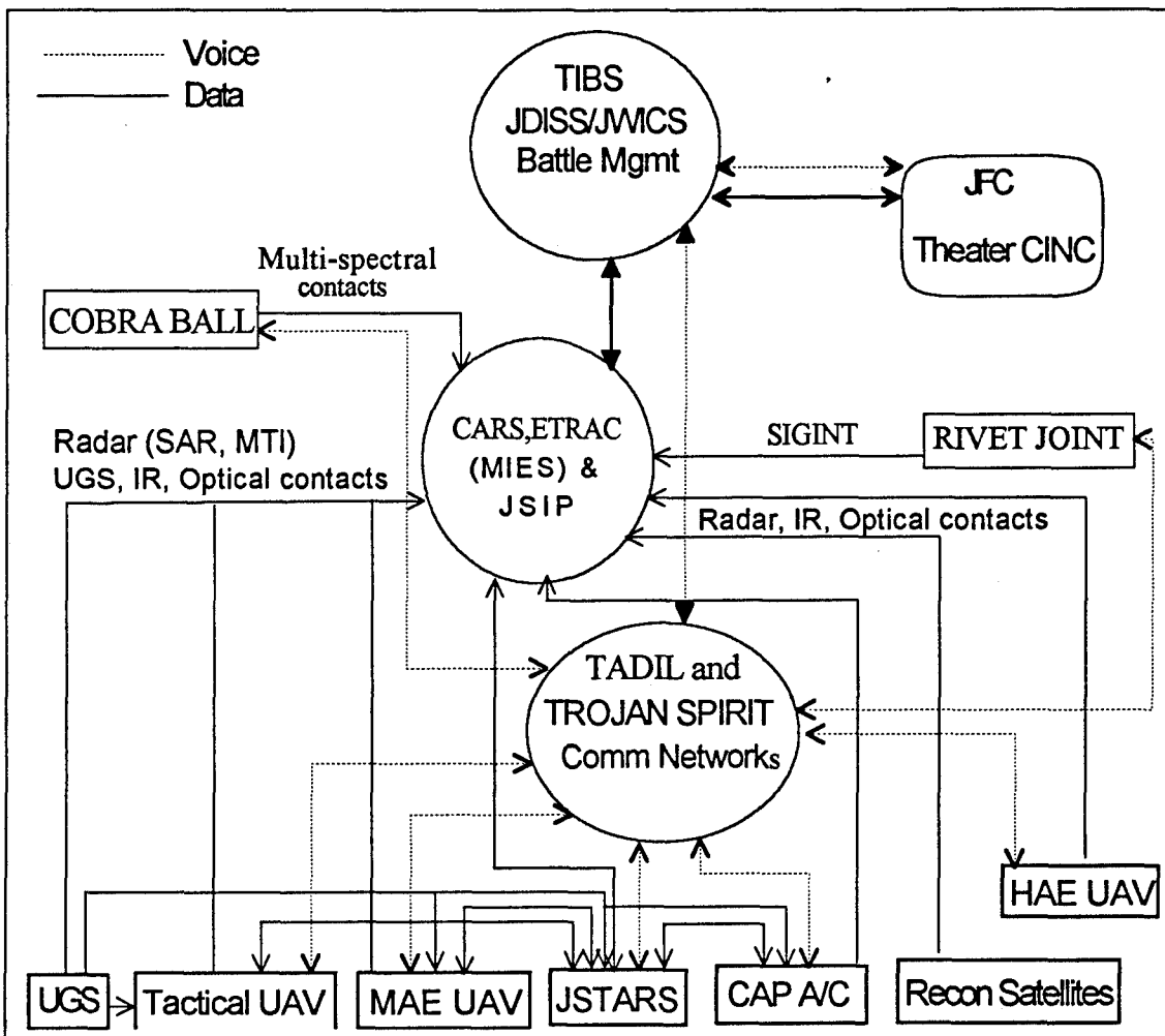
Figure 2: Notional platform integration and C4I of the joint anti-TBM infrastructure
