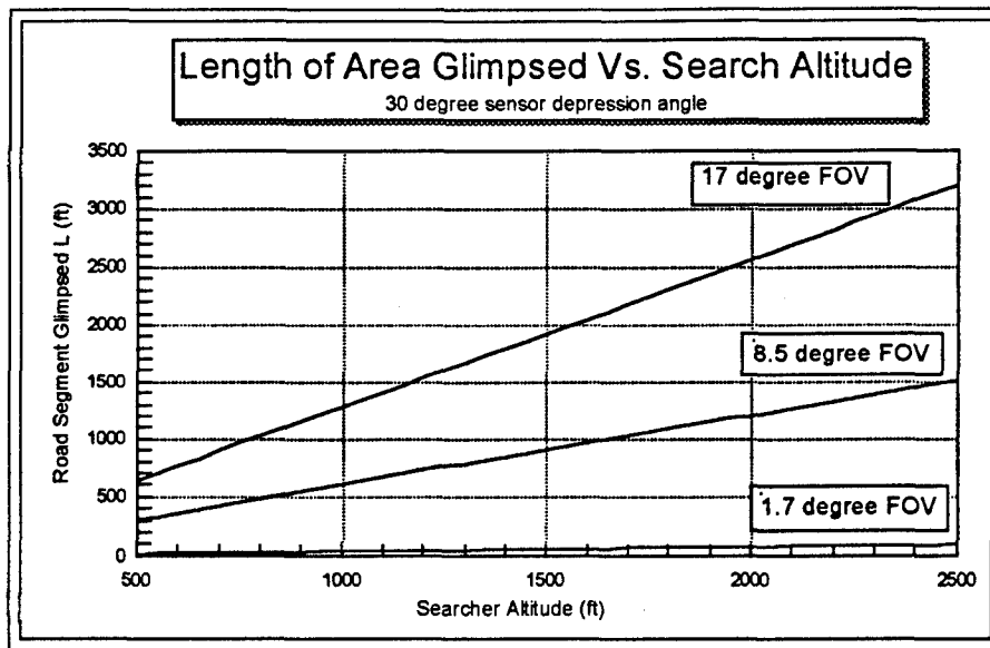
Figure 14: Length of area "glimpsed" versus search altitude and sensor FOV for the MKD-200 camera used aboard the PIONEER UAV with a 30° depression angle
