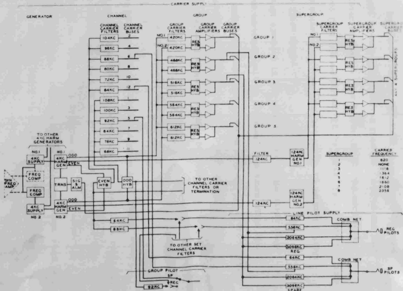
Fig. 7 - Block Schematic of the Carrier and Pilot Supply
