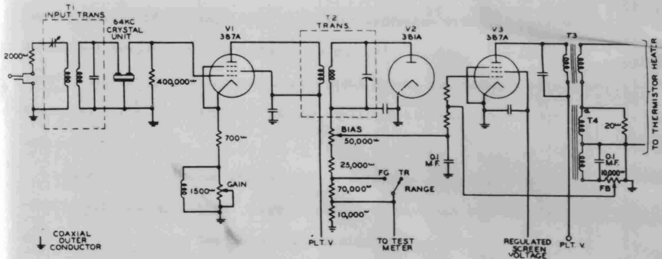
Fig. 16 - Simplified Schematic of 61A Regulator
