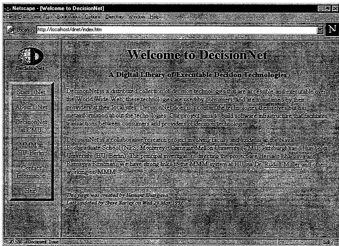
Figure 3. DecisionNet Shell.
