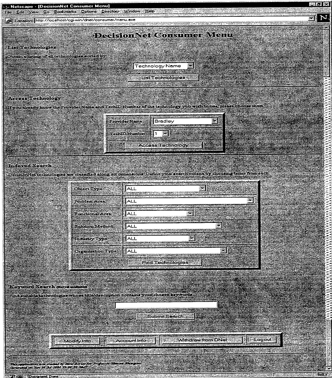
Figure 8. Consumer Menu.
